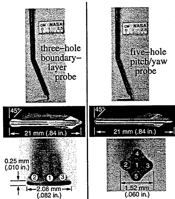
Fig. 3 Aerodynamic measurement probes
