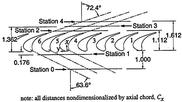
Fig. 2 Test section geometry and measurement plane locations
