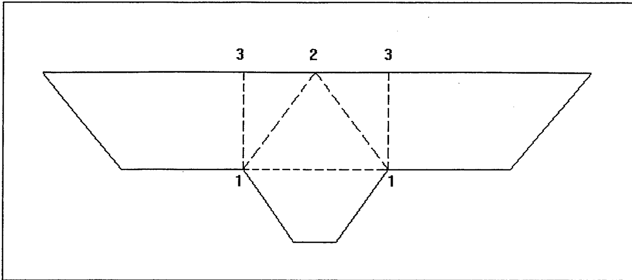
Figure 8. Definition sketch for channel divisions
