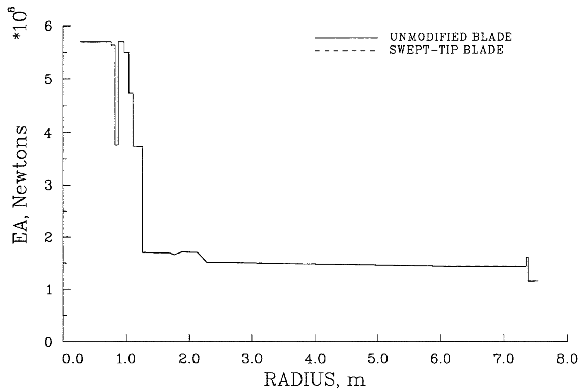
Figure A-5. Standard and swept-tip blade EA distribution.
