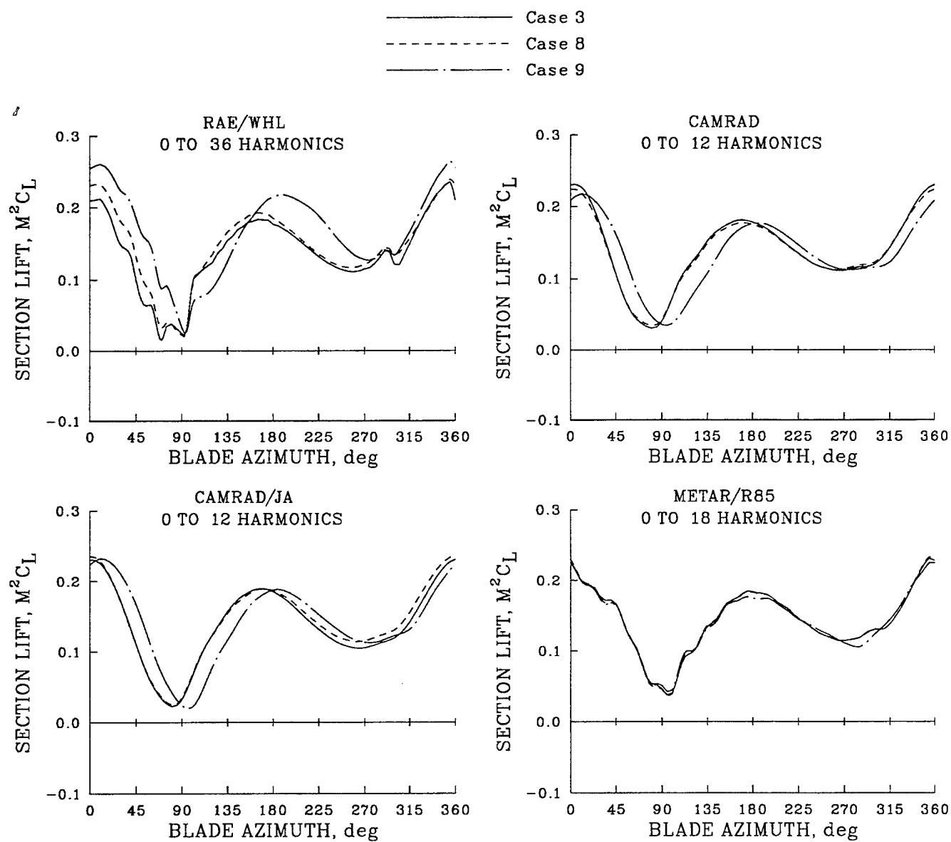
Figure 47. Comparison of normal force distribution as a function of azimuth for Cases 3, 8, and 9; 0.85R , all harmonics.
