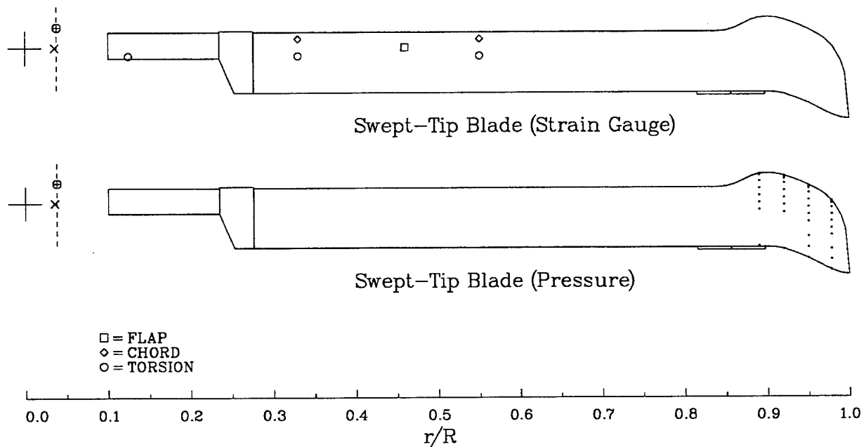
Figure 175. Instrumentation on Flight 487.
