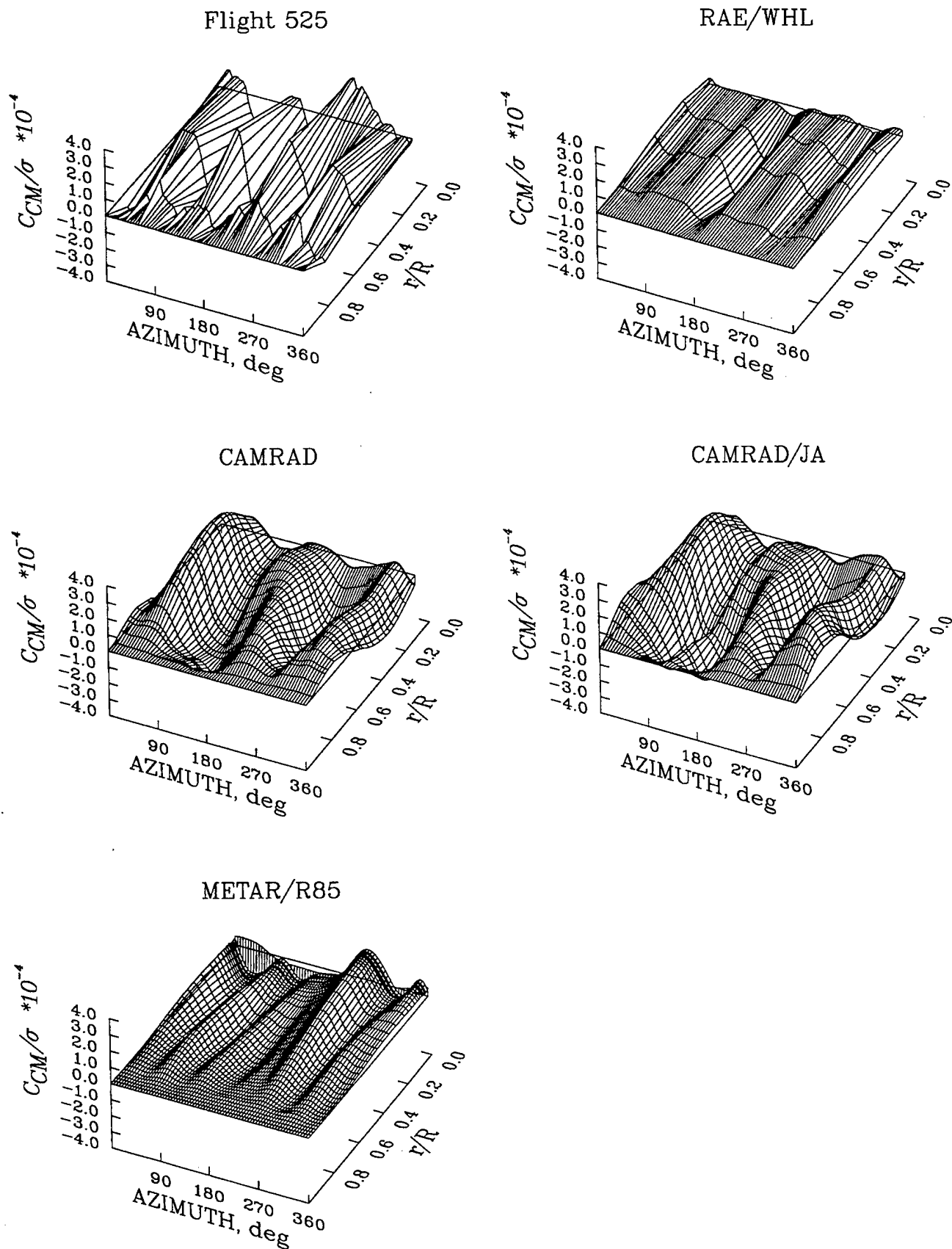
Figure 133. Comparison of measured and calculated chord bending moment as a function of azimuth and blade radius; \mu = 0.362 , Flight 525.
