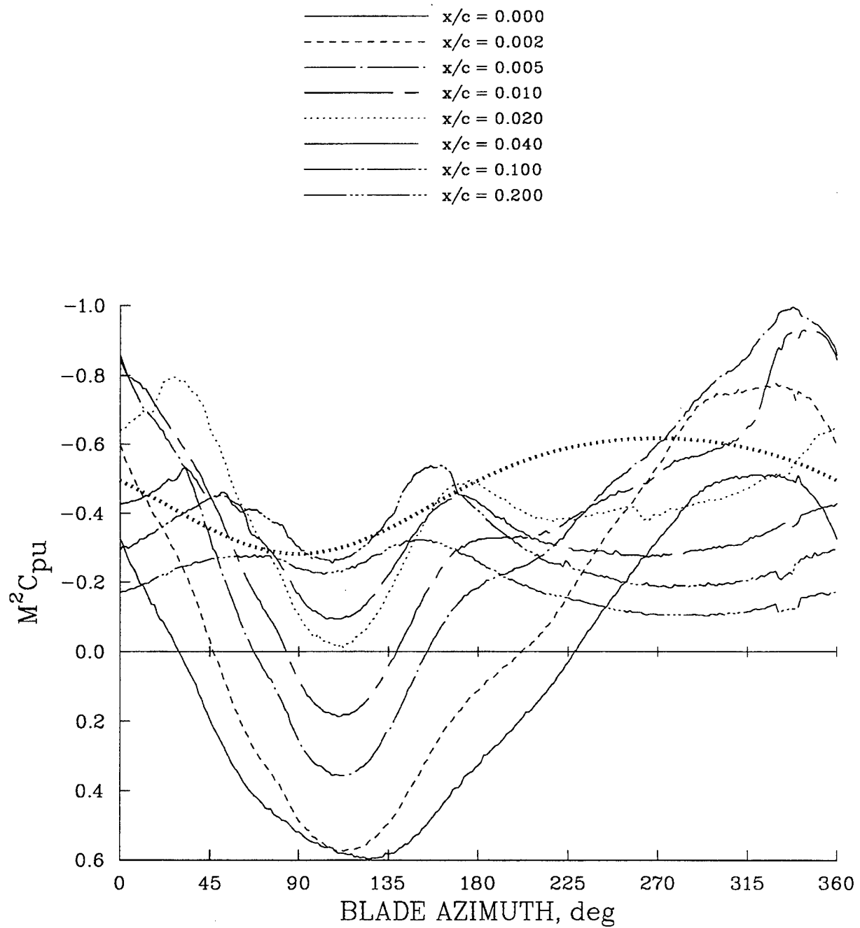
Figure 67. Upper surface pressure as a function of azimuth at high speed; 0.95R , \mu = 0.402 . M = 1 boundary shown as heavy dotted line.
