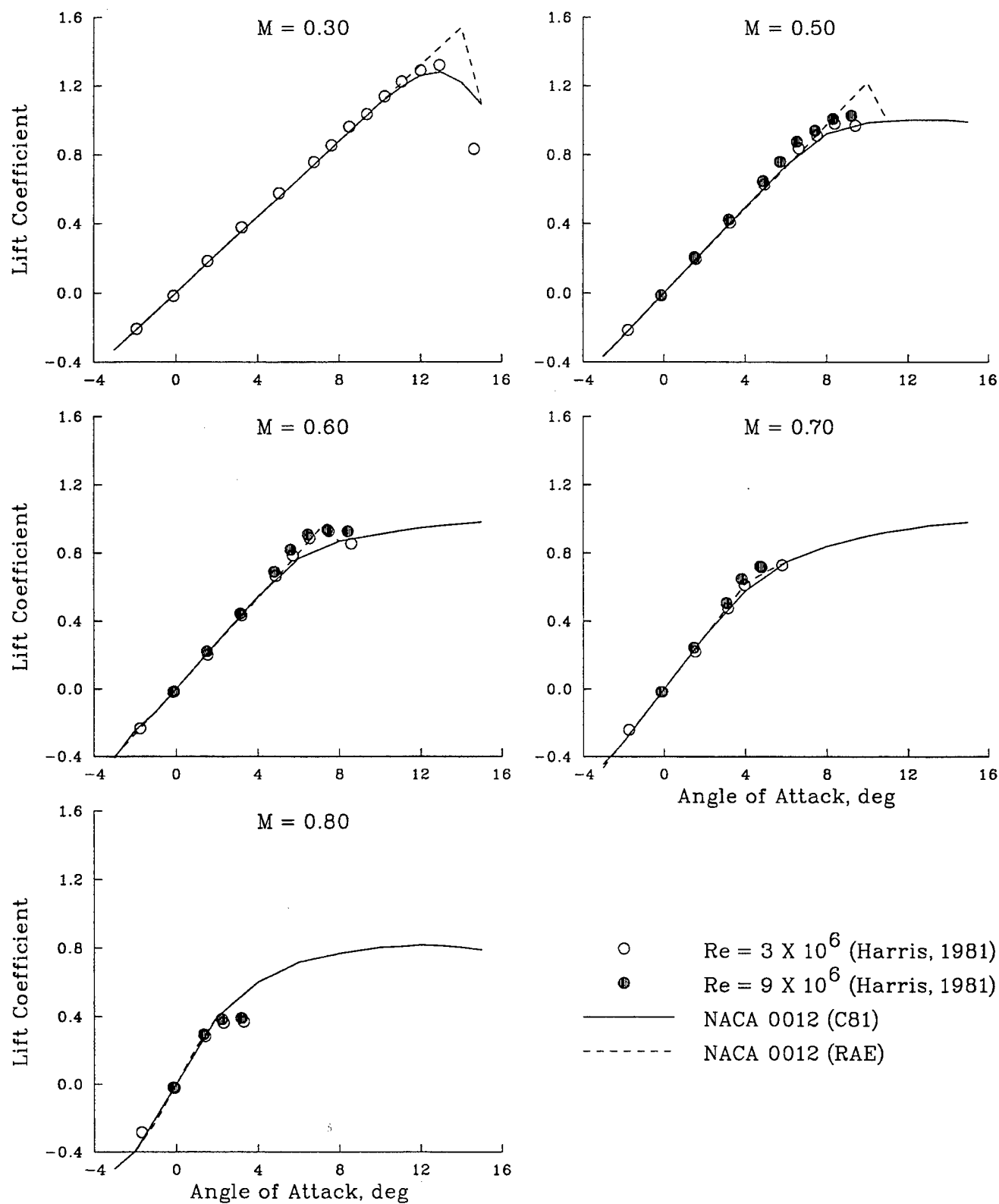
Figure 3. Comparison of lift coefficient from look-up tables with data from Harris (1981).
