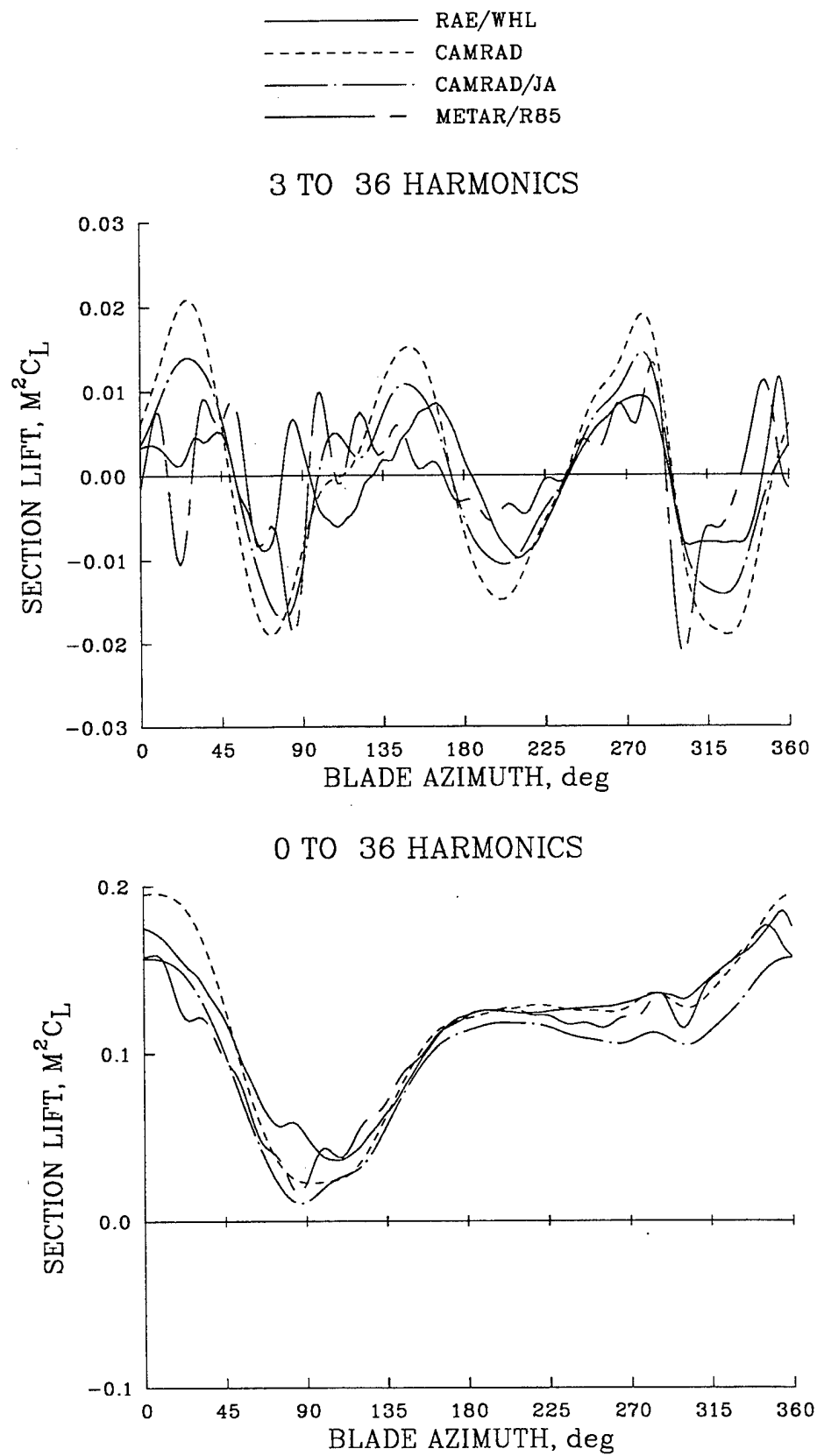
Figure 158. Calculated normal force as a function of azimuth at 0.95R ; Flight 123, \mu = 0.321 .
