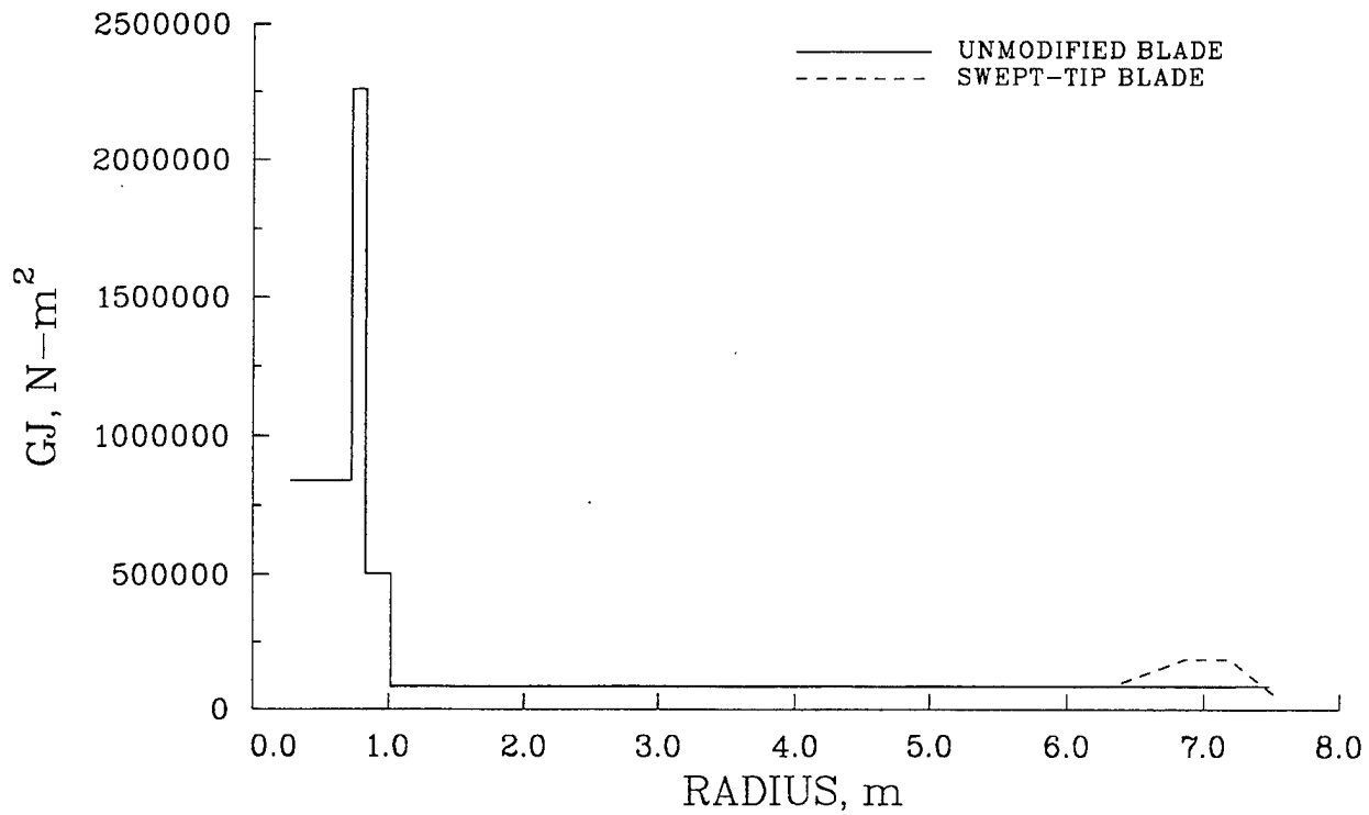
Figure A-8. Standard and swept-tip blade torsional stiffness distribution.
