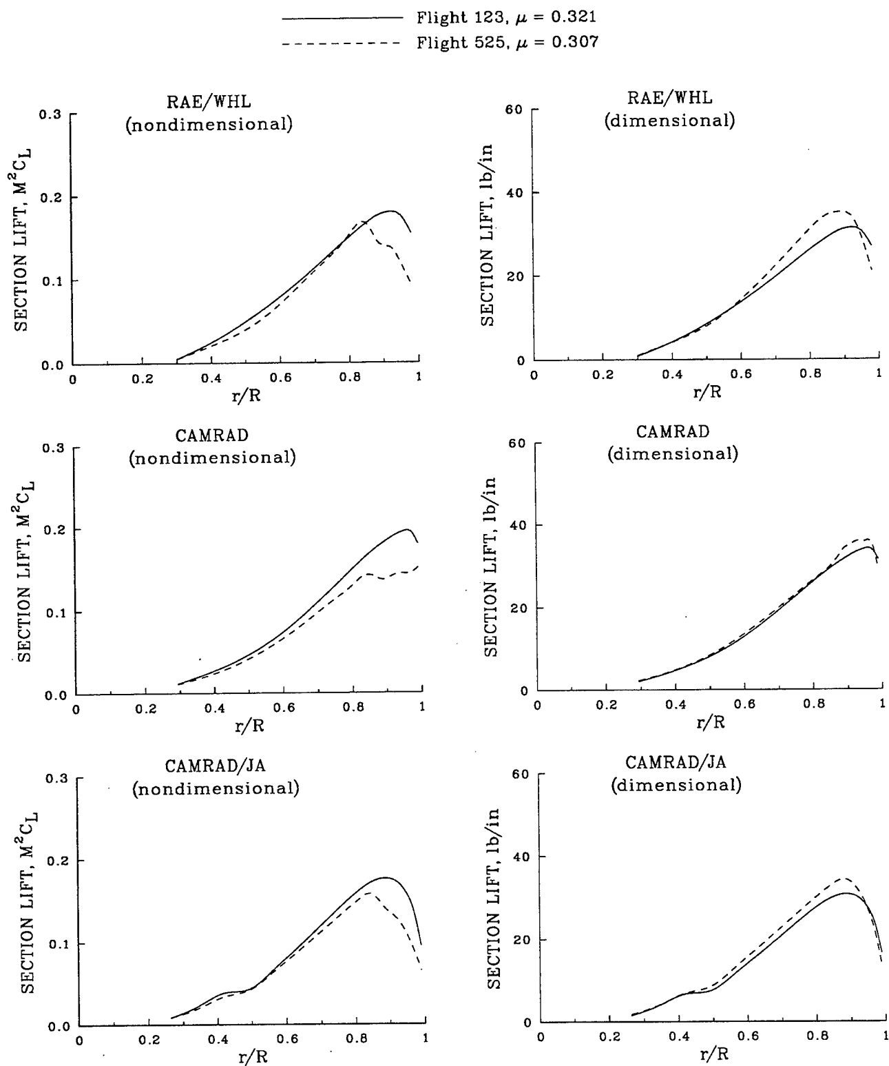
Figure 161. Comparison of calculated radial distributions of lift for a rectangular-tip and swept-tip blade; \psi = 0^\circ .
