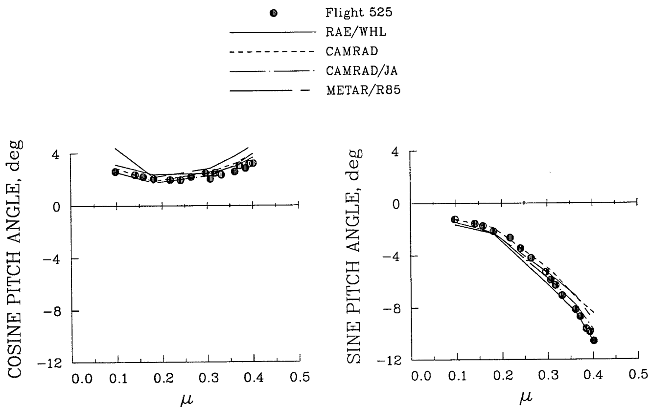
Figure 87. Comparison of measured and calculated cyclic pitch angles at the blade pitch bearing as a function of advance ratio for Flight 525.
