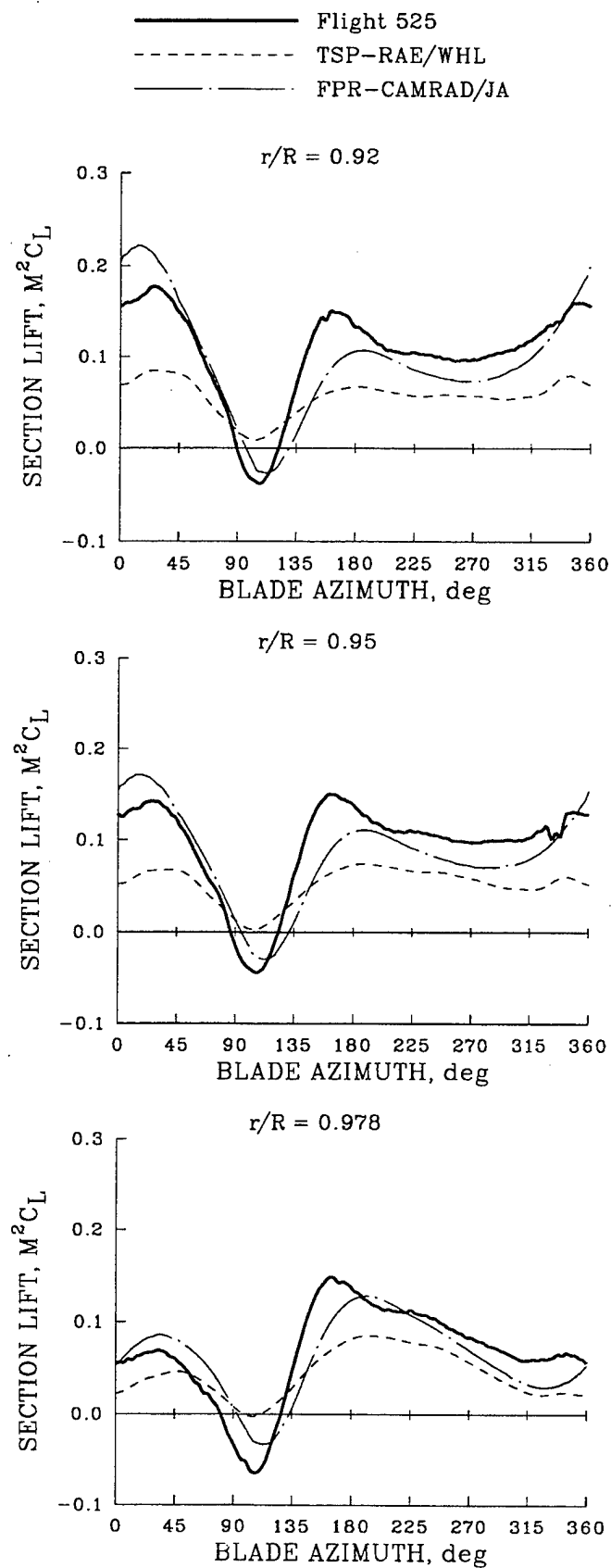
Figure 209. Comparison of hybrid CFD analyses with experiment for section lift; Flight 525.
