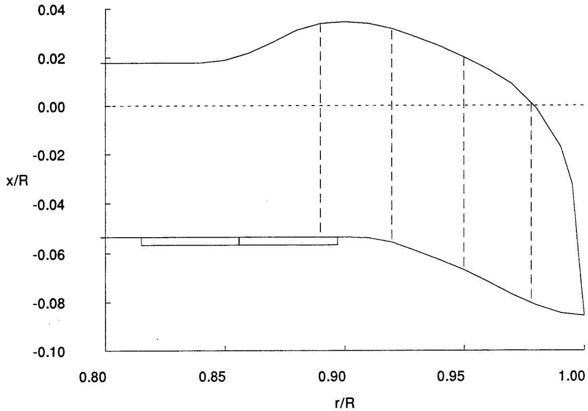
Figure 194. Swept tip planform of research Puma. Chordwise pressure transducer sections shown by dashed lines and feather axis by dotted line.
