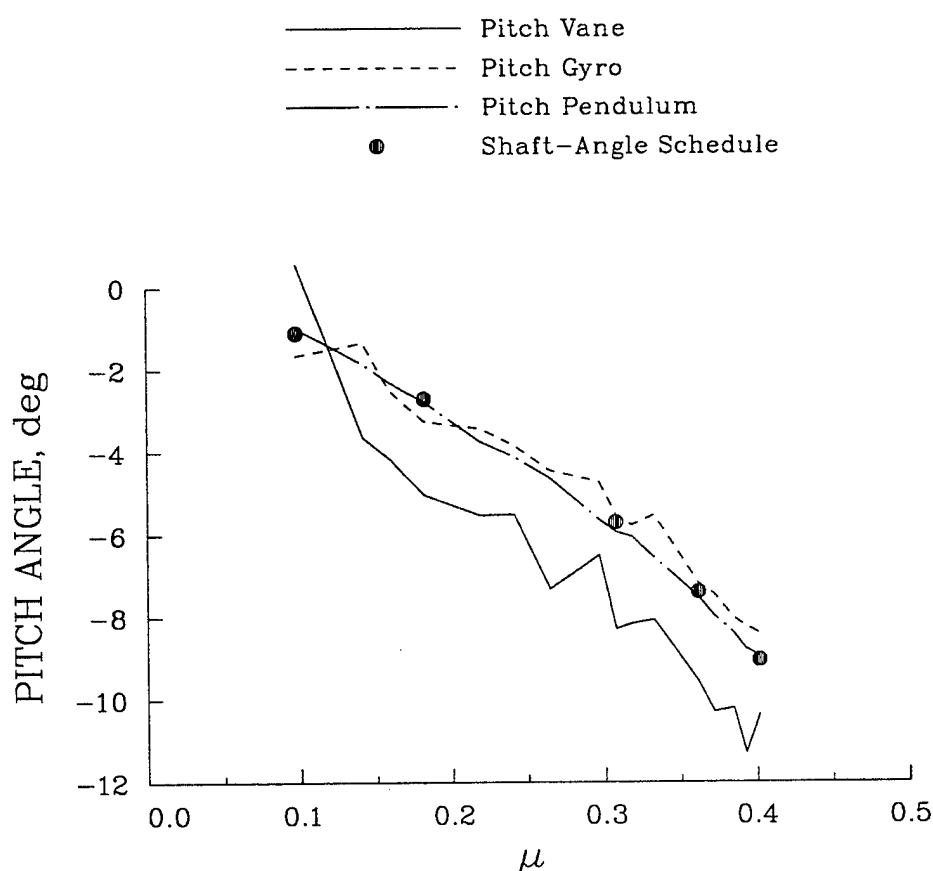
Figure 82. Shaft angle as a function of azimuth for three different measurements.
