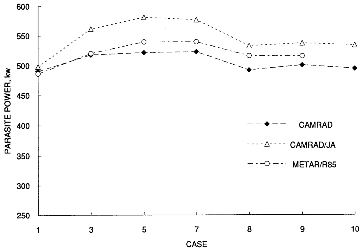
Figure 13. Calculated parasite power for Task 3 cases.
