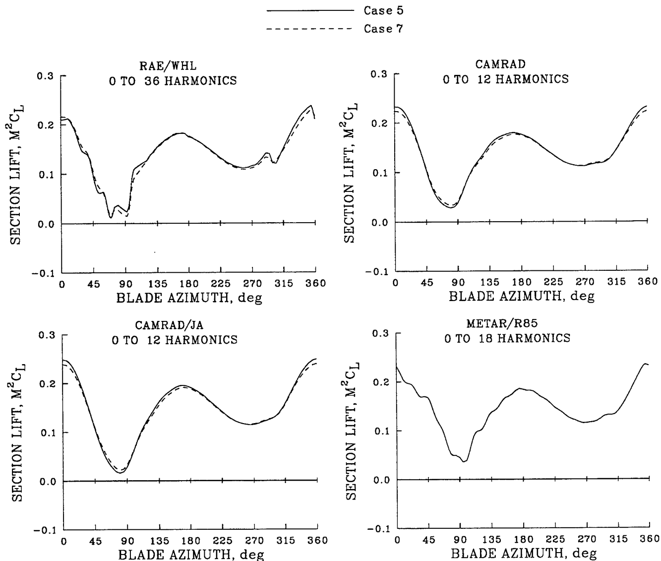
Figure 37. Comparison of normal force distribution as a function of azimuth for Cases 5 and 7; 0.85R , all harmonics.
