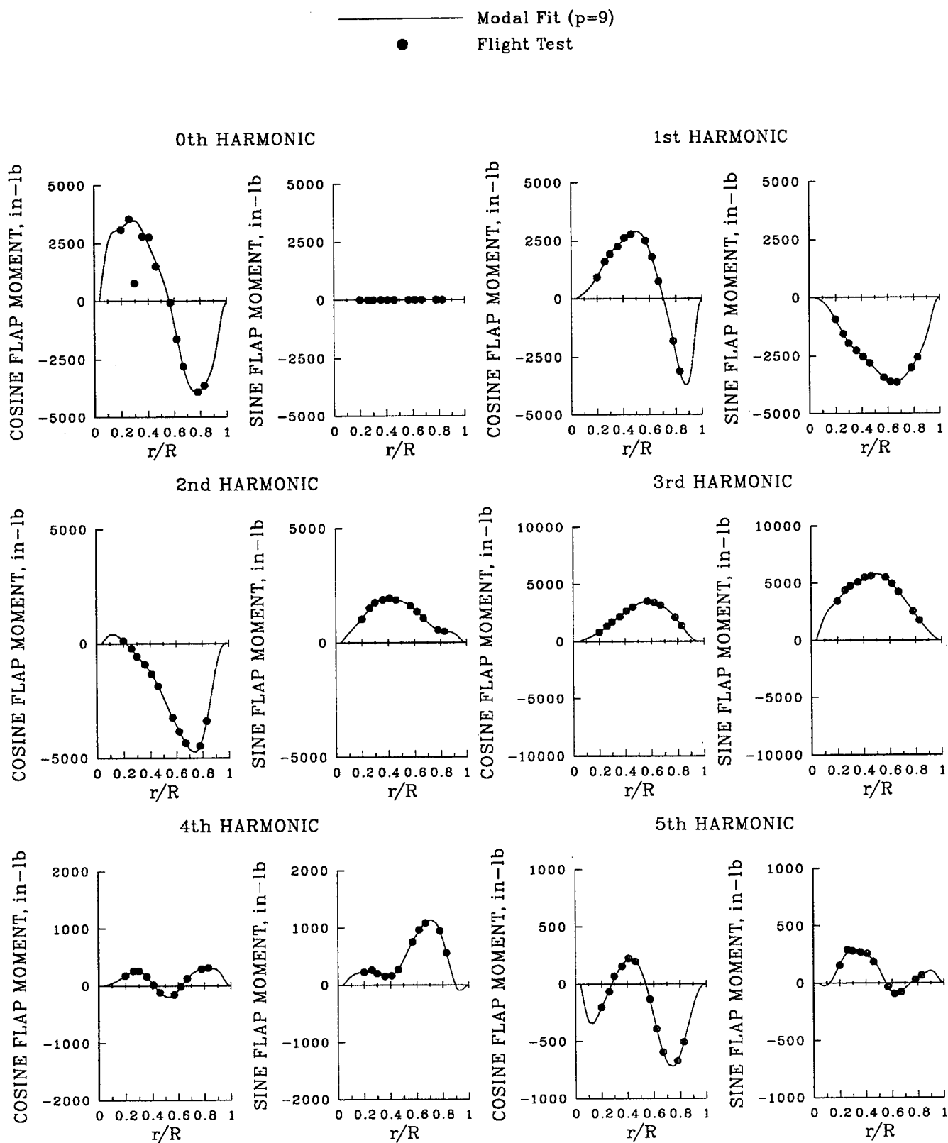
Figure 141. Modal fit of blade flap bending moment data using nine calculated modes; \mu = 0.402 .
