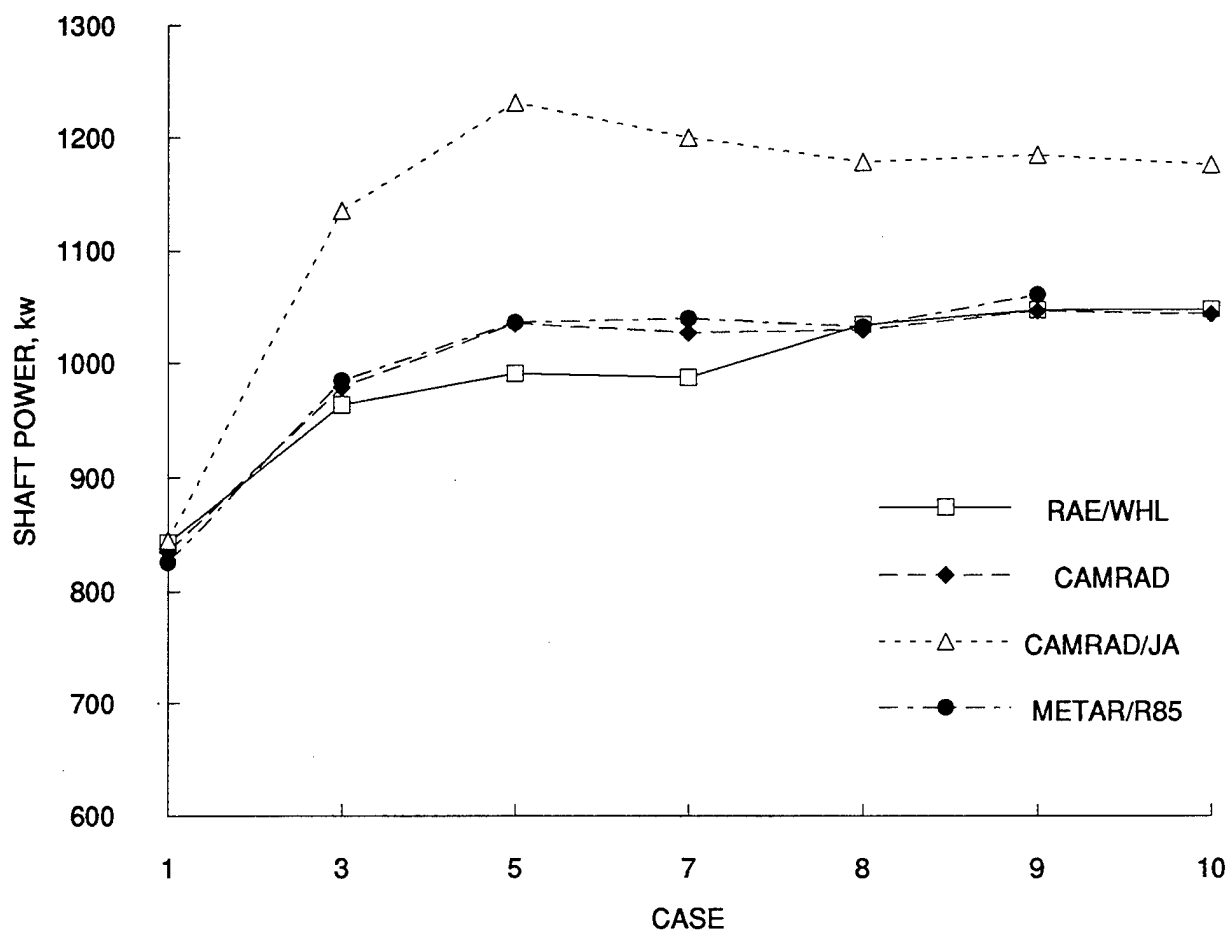
Figure 15. Calculated shaft power for Task 3 cases.
