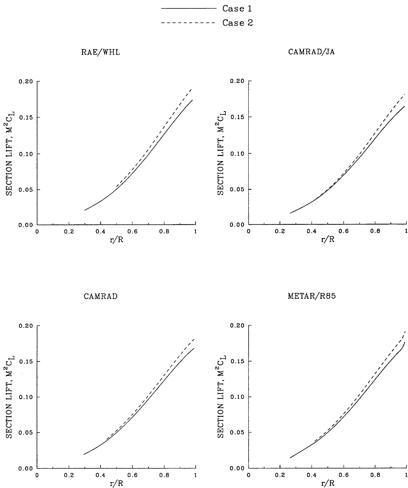
Figure 21. Comparison of radial distribution of steady normal force for Cases 1 and 2.
