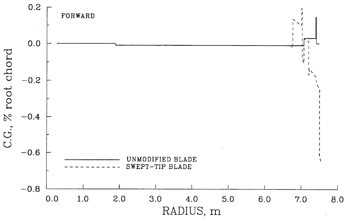
Figure A-4. Standard and swept-tip blade c.g distribution with respect to root quarter chord.
