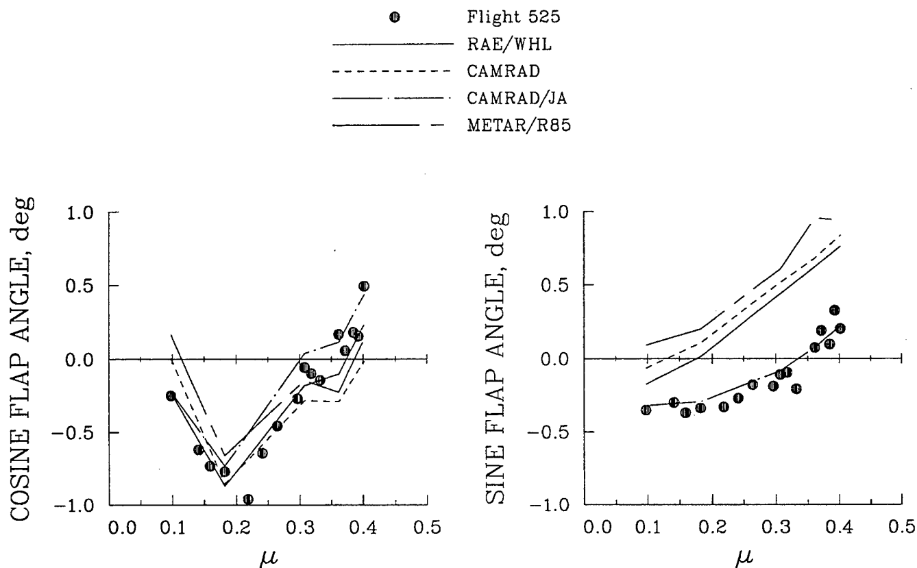
Figure 84. Comparison of measured and calculated first harmonic flapping as a function of advance ratio for Flight 525.
