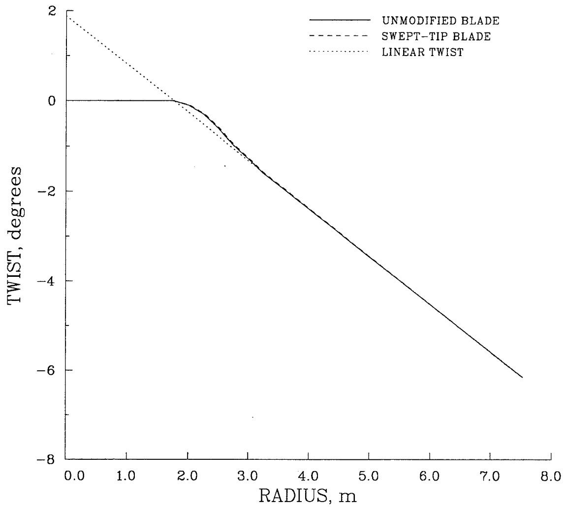
Figure A-2. Standard and swept-tip blade twist distribution.
