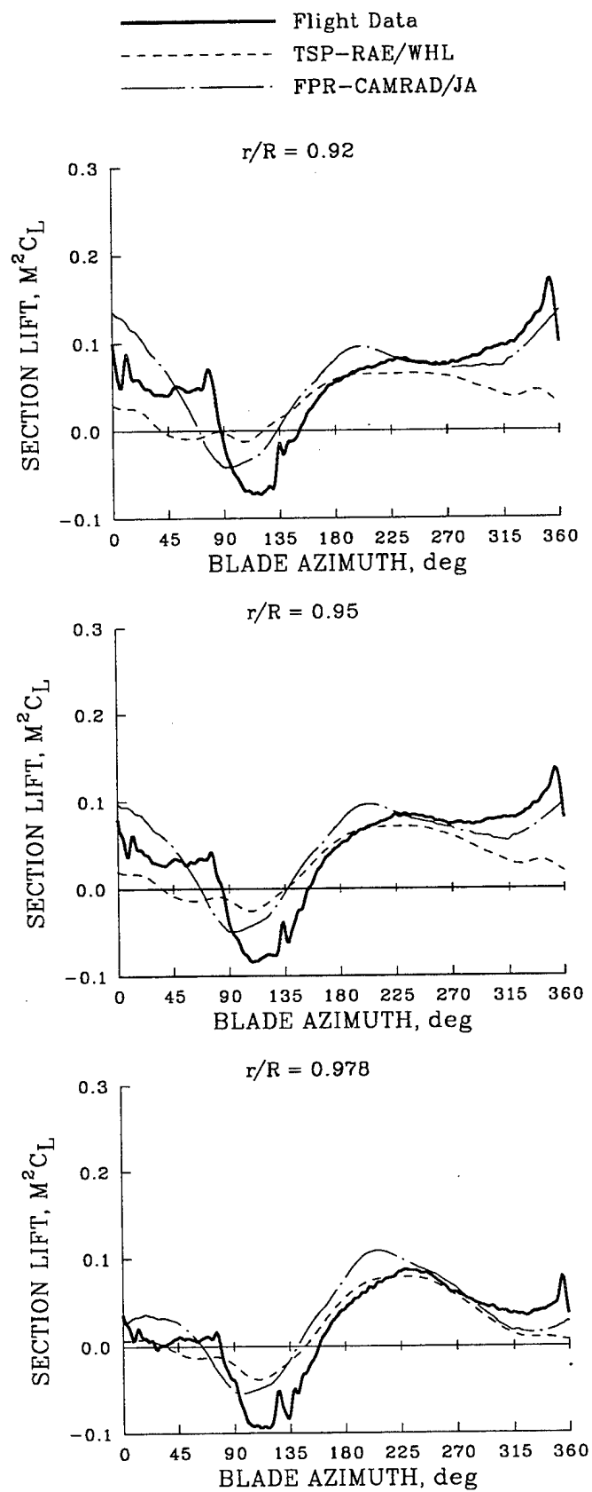
Figure 203. Comparison of hybrid CFD analyses with experiment for section lift; Flight 487.
