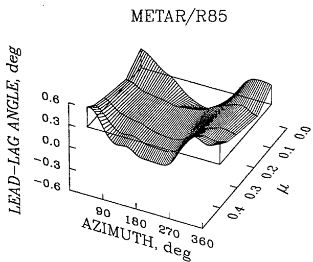
Figure 115. Comparison of measured and calculated blade lead-lag motion as a function of azimuth and advance ratio for Flight 525; 1-36 harmonics.
