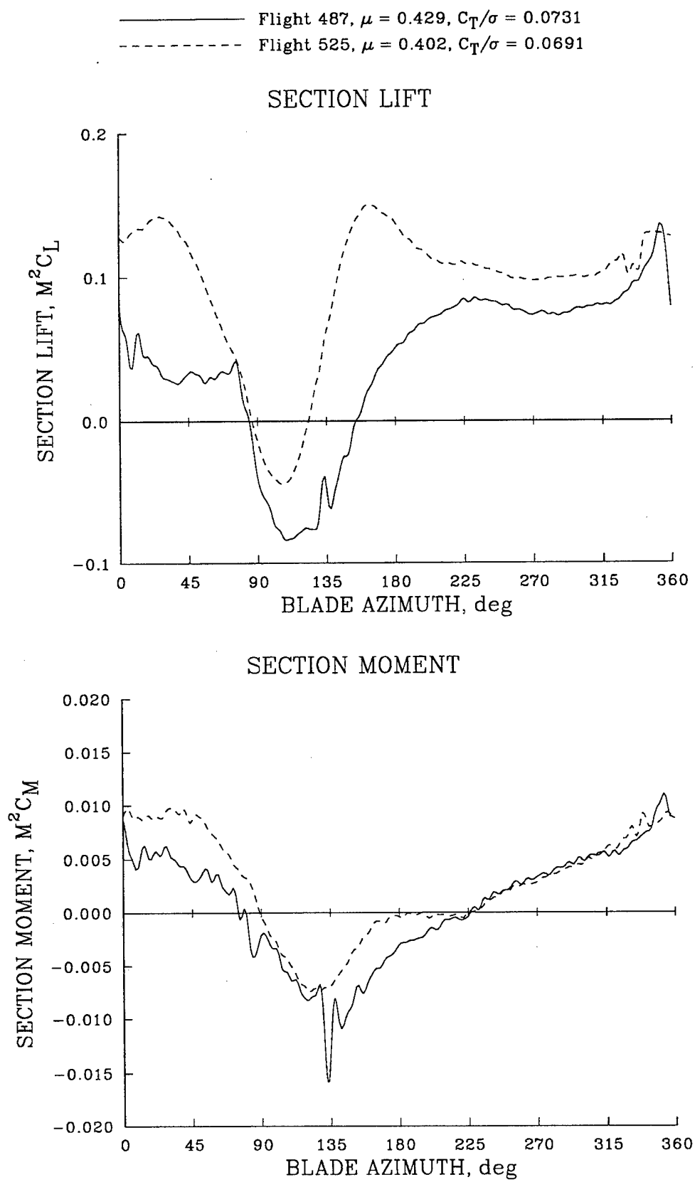
Figure 183. Comparison of normal force and pitching moment for flights 487 and 525; 0.95R .
