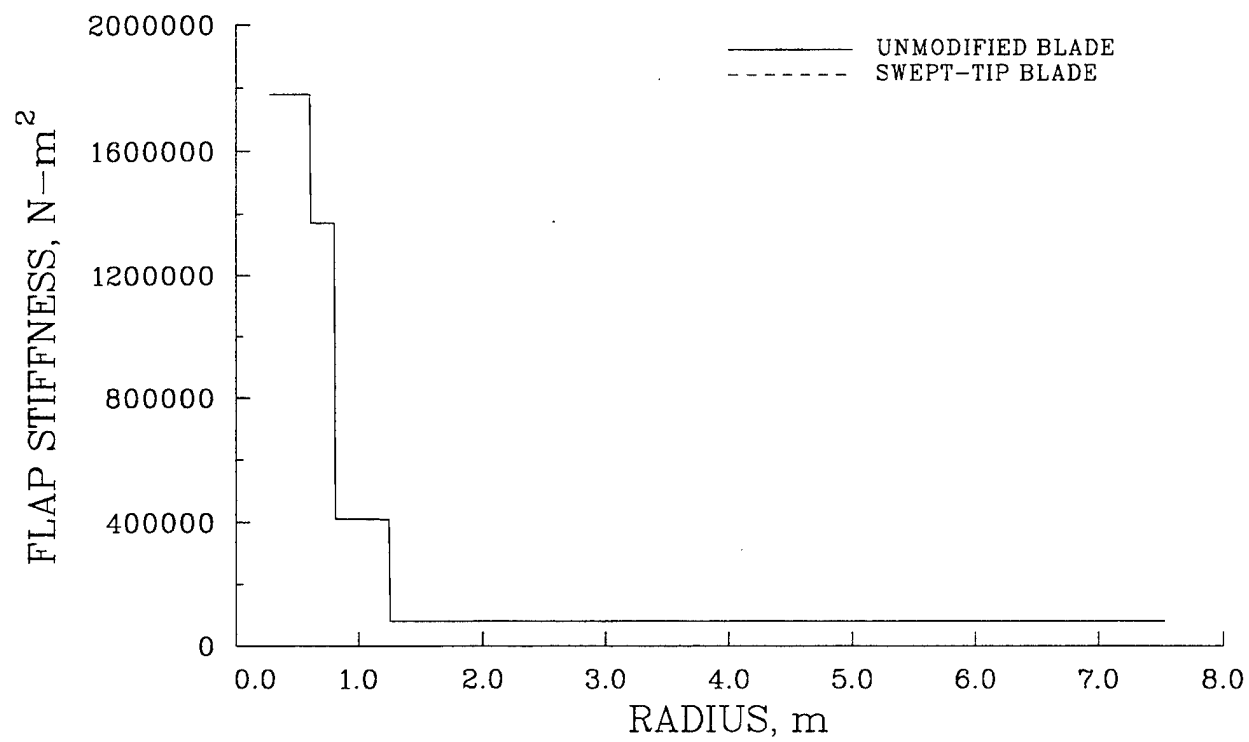
Figure A-6. Standard and swept-tip blade flap stiffness distribution.
