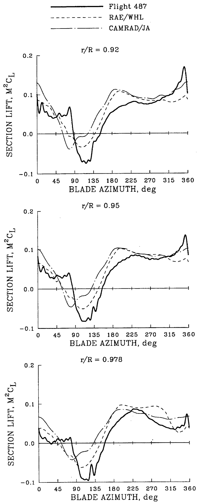
Figure 189. Comparison of experiment and calculation section normal force for the Flight 487 condition.
