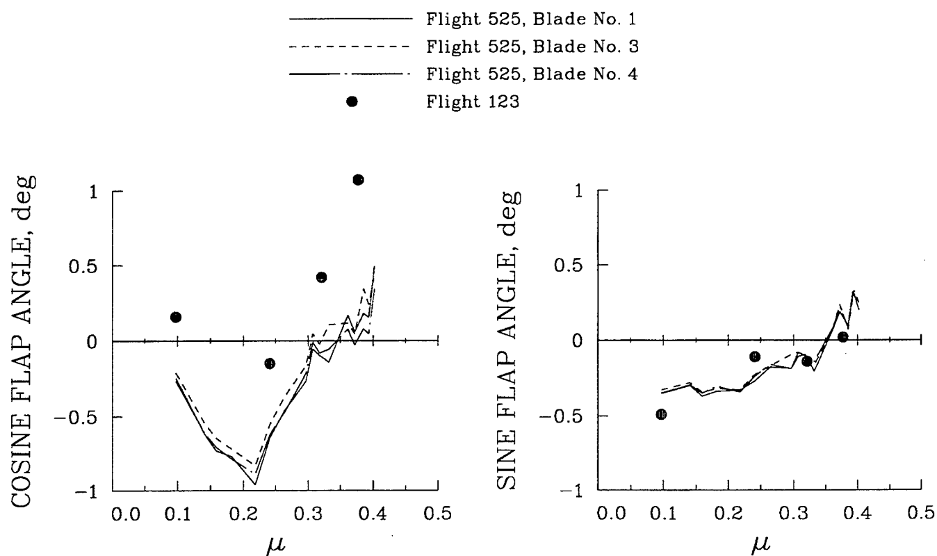
Figure 147. Flight 123 first harmonic flapping compared with Flight 525 values.
