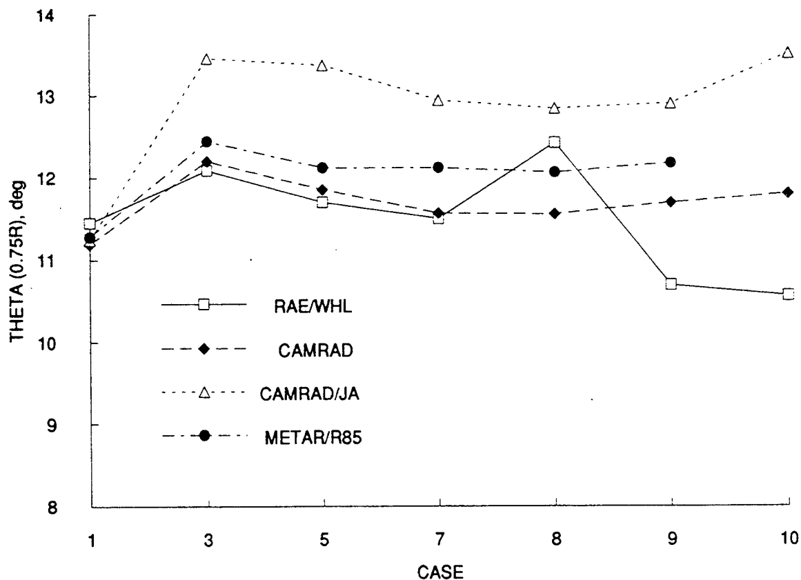
Figure 6. Calculated collective pitch for the Task 3 cases.
