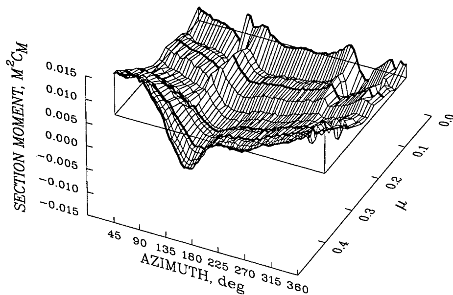
Figure 63. Section lift and pitching moment as a function of azimuth and advance ratio for Flight 525; 0.95R . Correlation cases shown by thickend lines.
