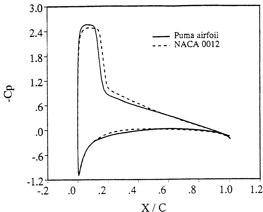
Figure 199. Viscous calculation results; M_\infty = 0.60 , \alpha = 6.0^\circ . NACA 0012: C_l = 0.8244 , C_d = 0.02333 , C_m = 0.02612 ; Puma airfoil: C_l = 0.7840 , C_d = 0.02349 , C_m = 0.02904 .
