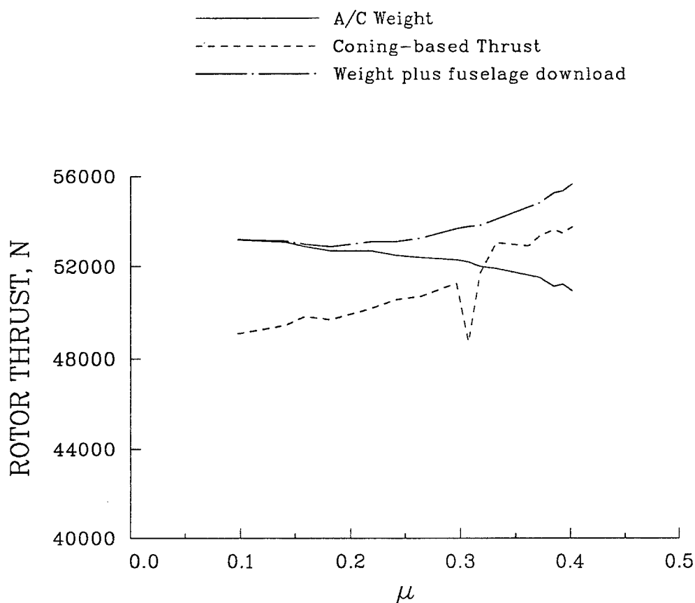
Figure 85. Aircraft gross weight, gross weight plus fuselage and stabilizer download, and coning-based thrust as functions of advance ratio.
