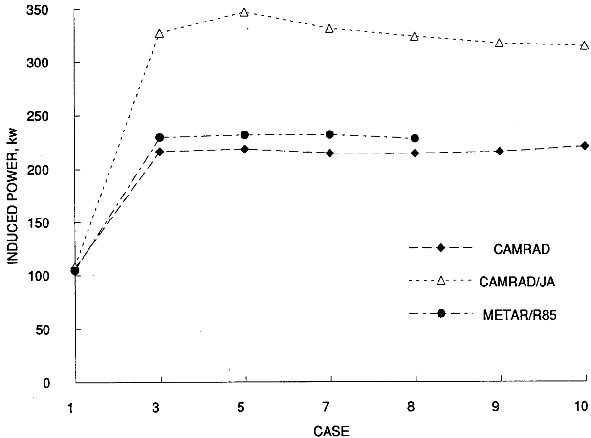
Figure 12. Calculated induced power for Task 3 cases.
