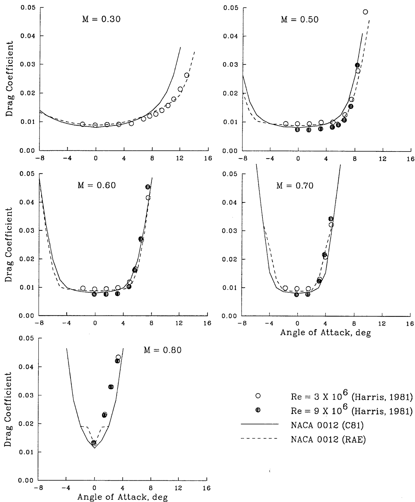
Figure 4. Comparison of drag coefficient from look-up tables with data from Harris (1981).
