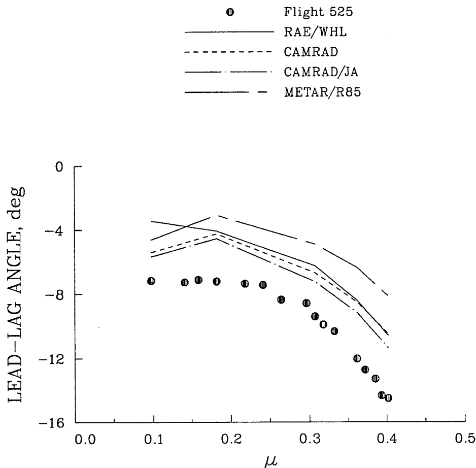
Figure 89. Comparison of measured and calculated blade steady lag angle as a function of advance ratio for Flight 525.
