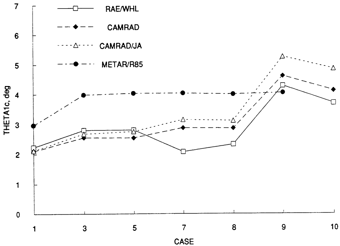
Figure 7. Calculated lateral cyclic pitch for the Task 3 cases.
