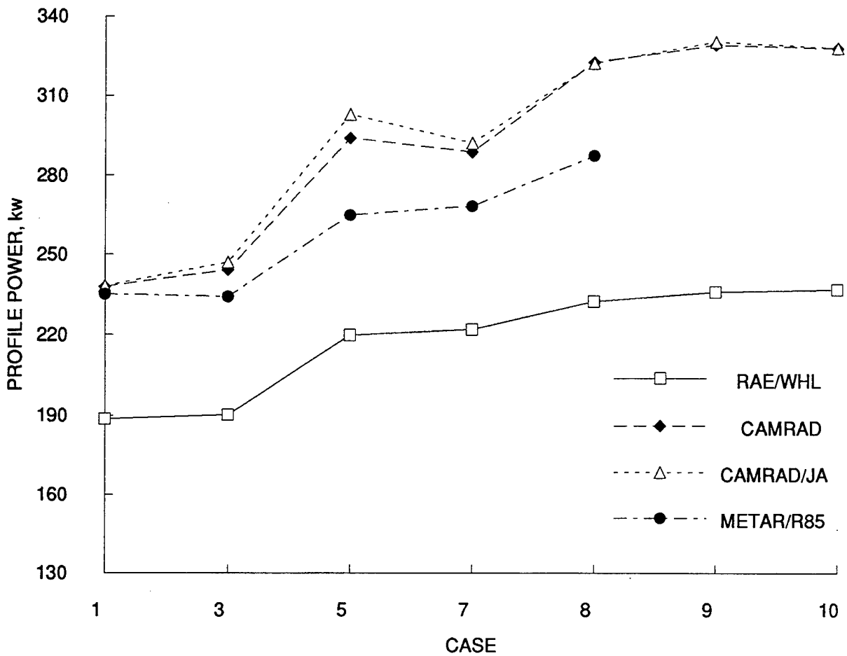
Figure 11. Calculated profile power for Task 3 cases.
