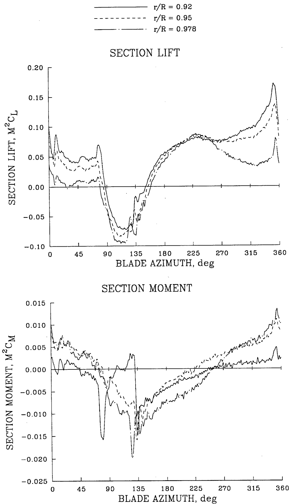
Figure 178. Section normal force and pitching moments; Flight 487.
