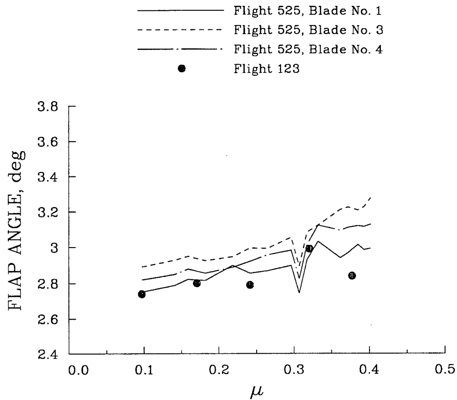
Figure 150. Flight 123 coning angles compared with Flight 525 values.
