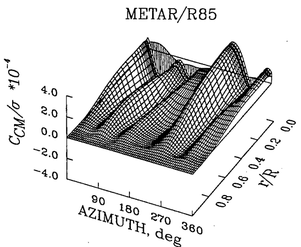
Figure 136. Comparison of measured and calculated chord bending moment as a function of azimuth and blade radius; \mu = 0.402 , Flight 525.
