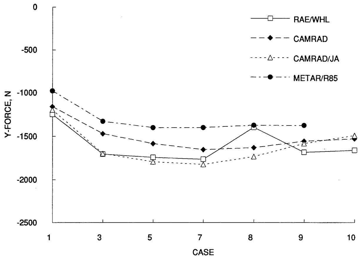
Figure 10. Calculated lateral forces for Task 3 cases.
