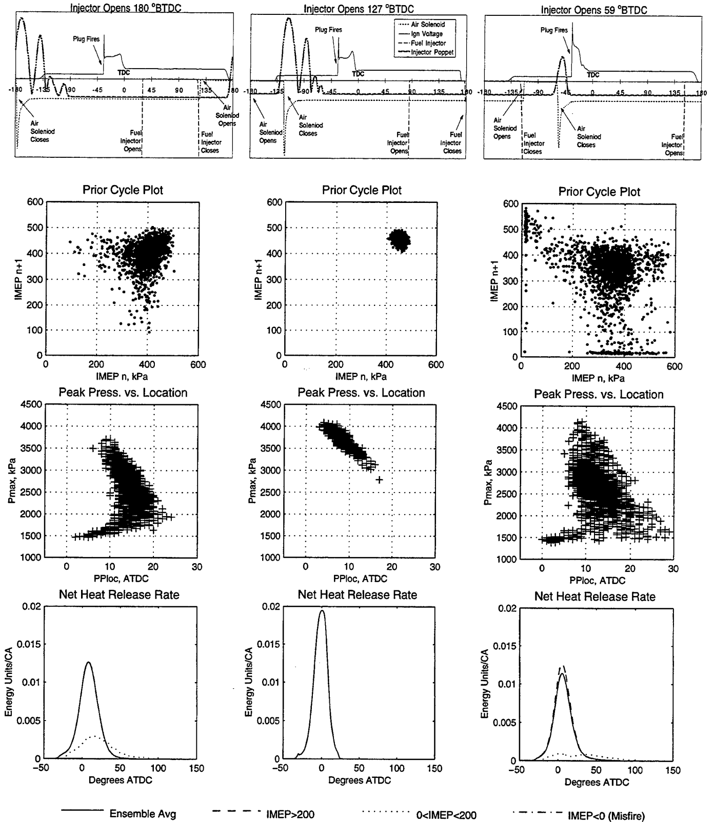
Figure 7: 2000 RPM High Load at Three Injection Timings
