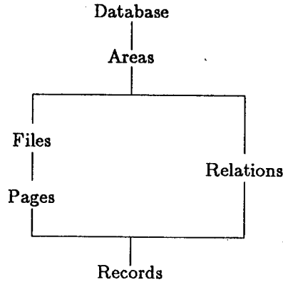
Fig. 2.1. A Lattice of Granularities.
