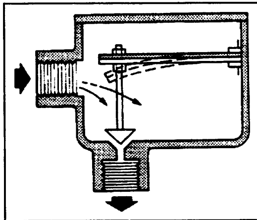
Figure 3. Bimetallic trap.
