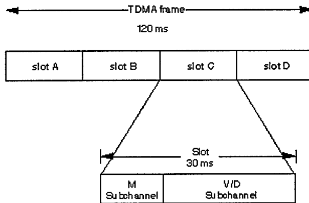
30 ms slot at 31.5 kbps (10.5 K symbol/sec)
