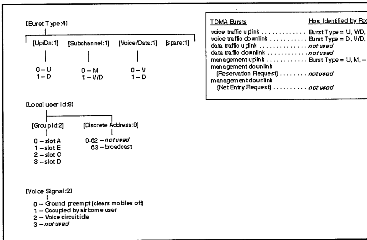
Figure 2-3. Burst Type, Local User Id and Voice Signal Fields (Voice-Only System Configurations)
