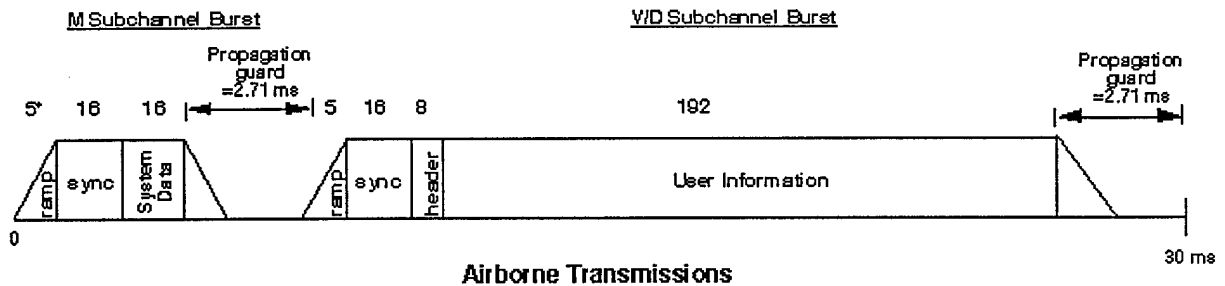
30 ms slot at 31.5 kbps (10.5 K symbol/sec)
