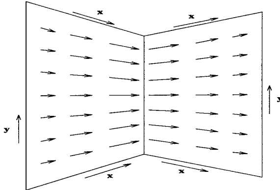
Figure 5: Velocity basis function on quadrilaterals
