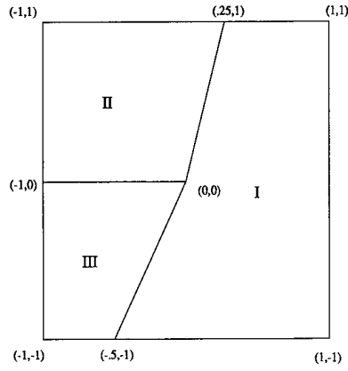
Figure 8: Distorted regions for Problem 6 with variable tensor permeability
