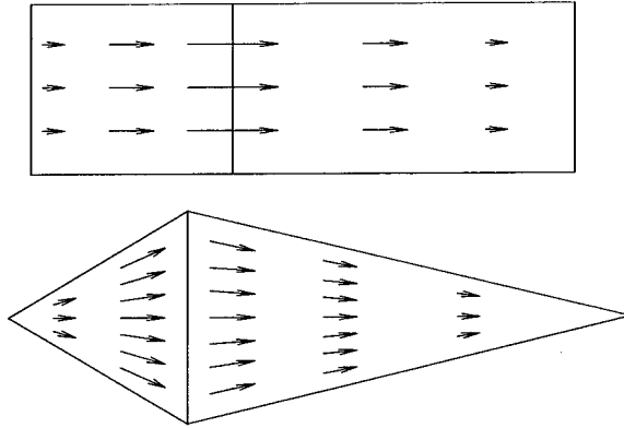
Figure 2: Velocity basis functions on rectangles and triangles
