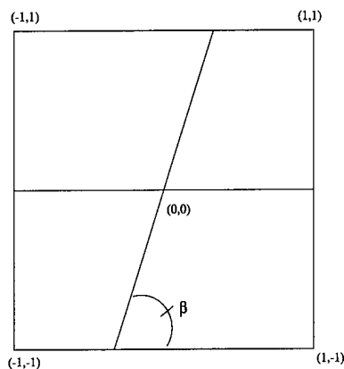
Figure 7: Macro-blocks of distorted grids
