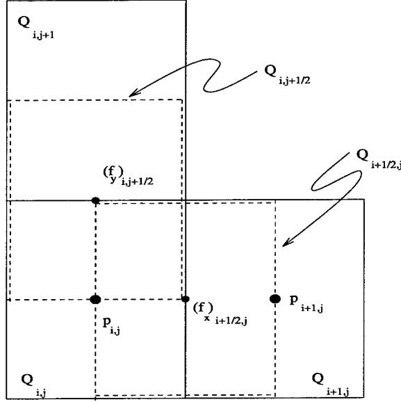
Figure 3: Unknowns and control volumes for rectangular grid
