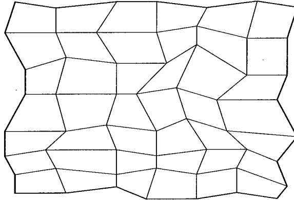
Figure 1: Logically rectangular grid of irregular quadrilaterals
