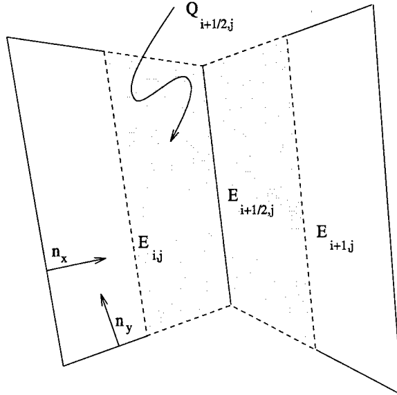
Figure 6: Control-volume mixed finite elements on quadrilaterals
