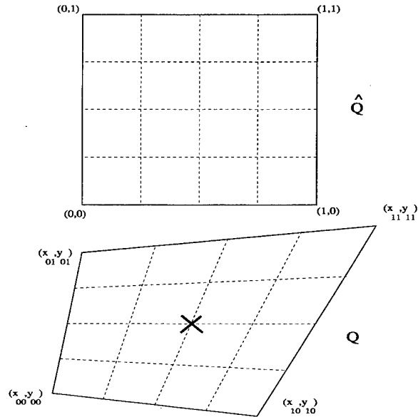
Figure 4: Reference quadrilateral \hat{Q} and quadrilateral Q
