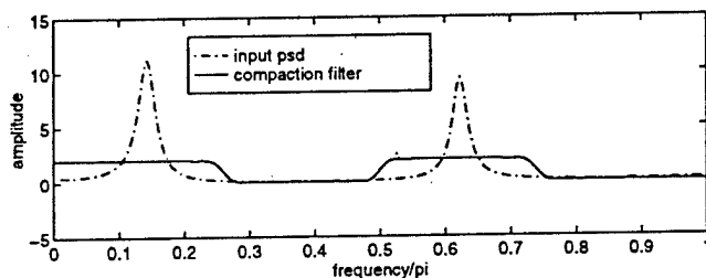
Figure 4. The psd of an AR(5) process, and the magnitude square of an optimal compaction filter designed by linear programming ( M = 2, N = 65 ).
