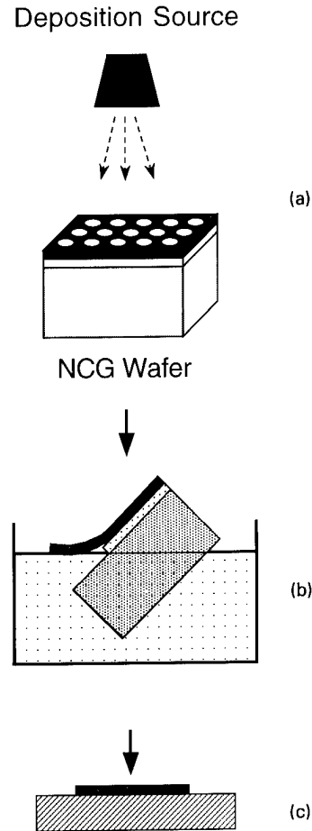
Fig. 4 — The preparation of NCG replica membranes: (a) an easily dissolved buffer layer and a desired membrane layer are deposited onto the surface of an NCG wafer; (b) the membrane is released by dissolving the buffer layer in an appropriate chemical solution; and (c) after rinsing, the membrane is placed on a substrate for a desired patterning application.
