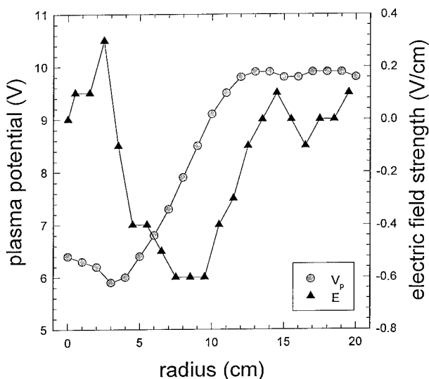
Fig. 4 — Electric field and plasma potential profiles produced by the MRE.
