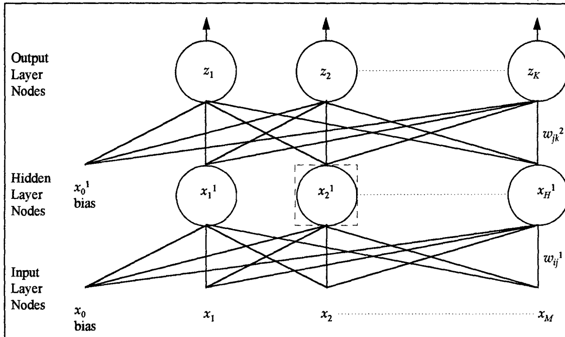
Figure 2. Multilayer Network
