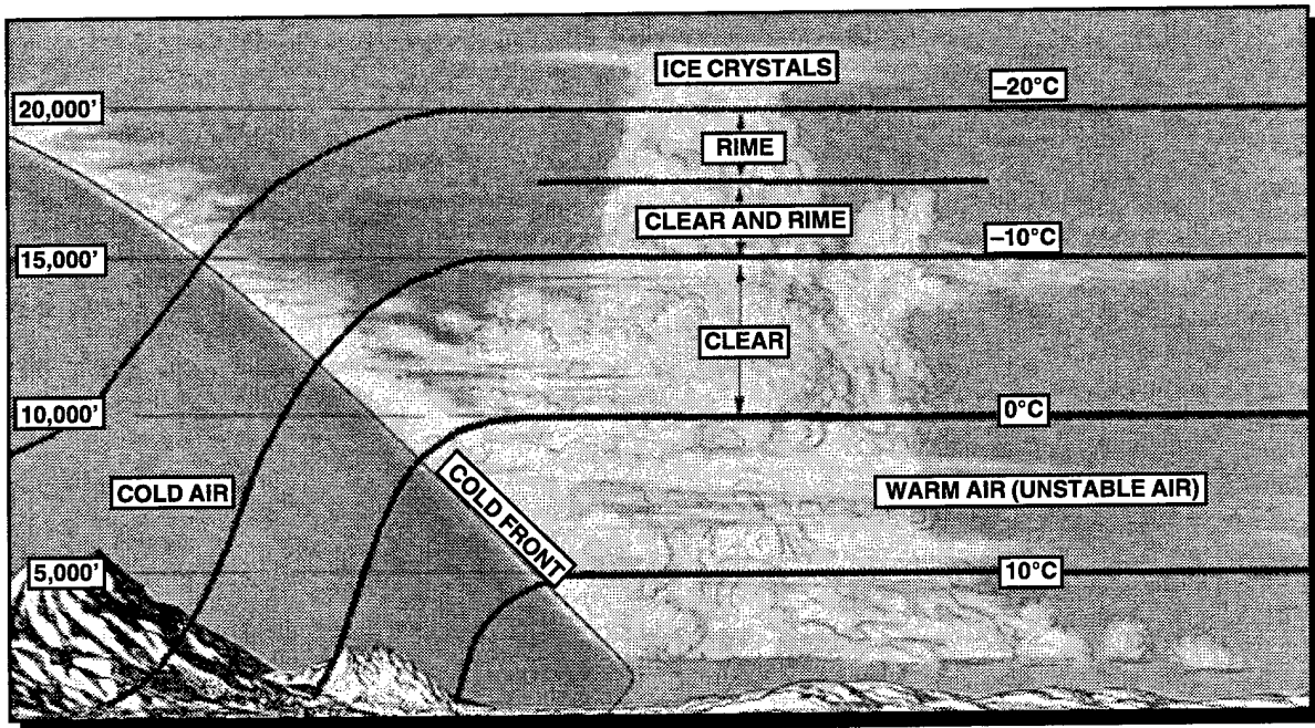
Figure 2. Icing Associated with Cold Fronts
