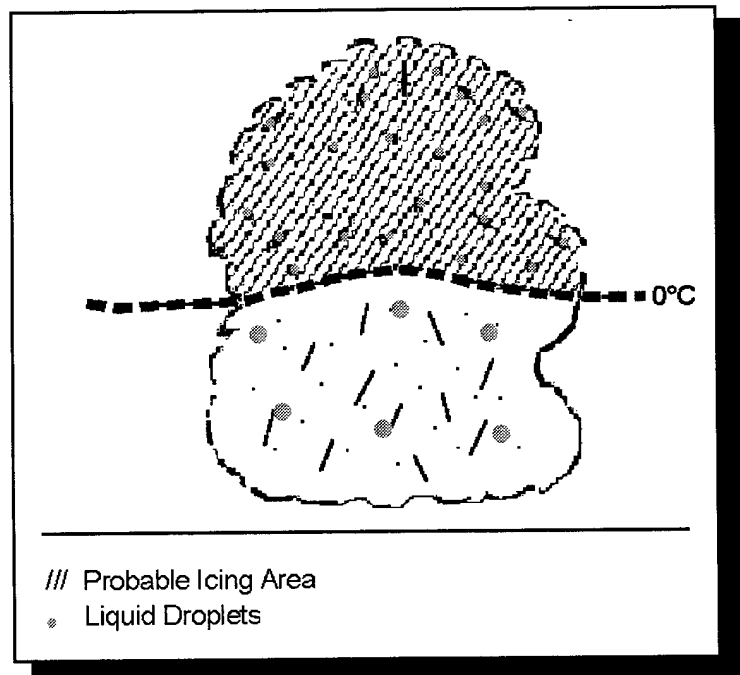
Figure 3. Icing Associated with Cumuliform Clouds
