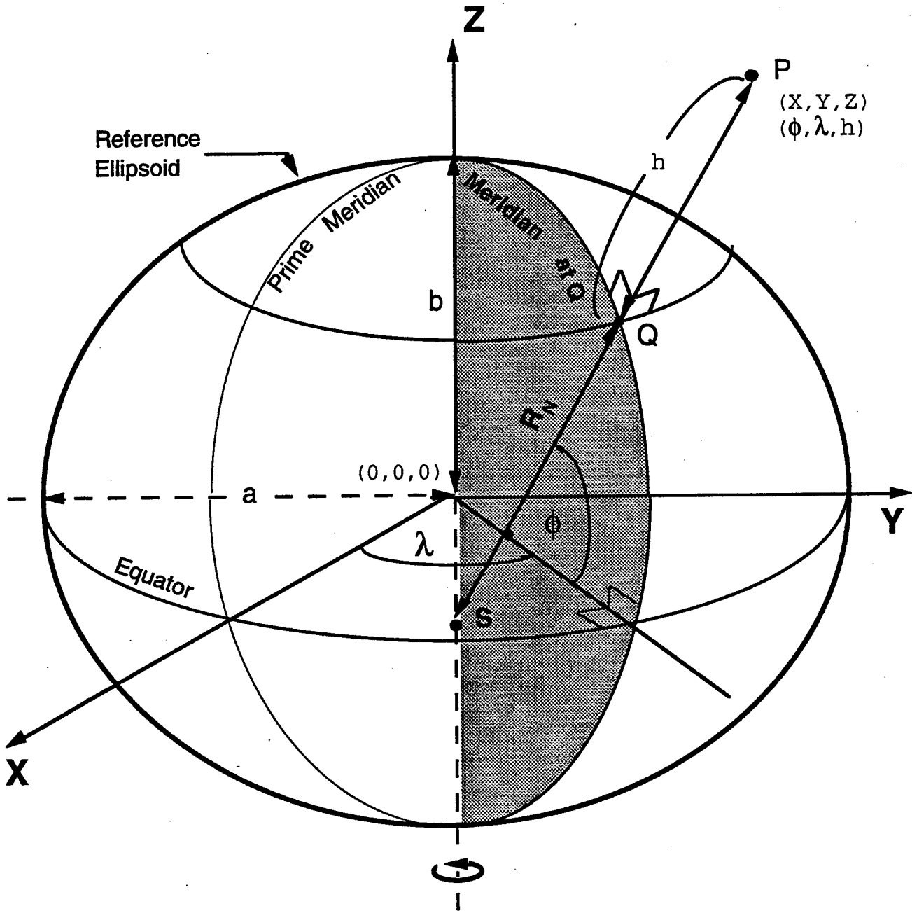
Figure 4.2 The geometric relationship between Cartesian and geodetic coordinates.
