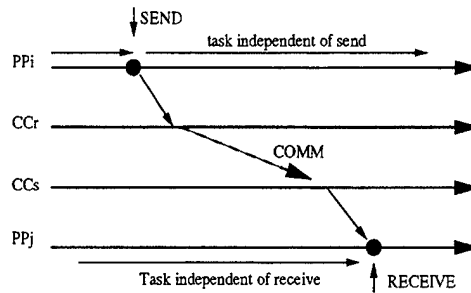
Figure 7: Proteus Communication Scheduling
