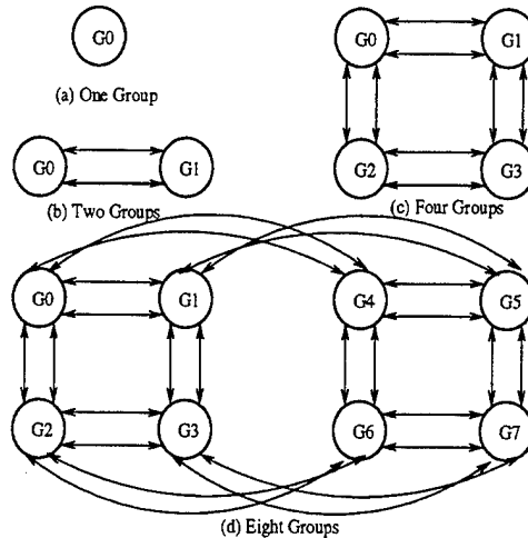
Figure 12: Some configurations of the Proteus system
