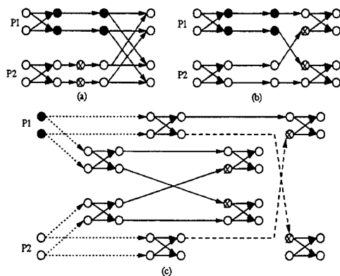
Figure 11: a) Tradition butterflies, b) Optimized butterflies, c) Optimized butterflies with overlapping communication/computation.
