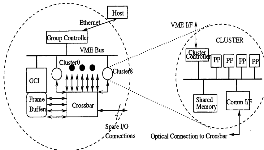
Figure 1: The Proteus System Architecture
