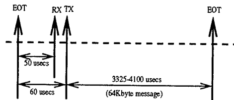
Figure 4: The Proteus Communication Cycle Timing
