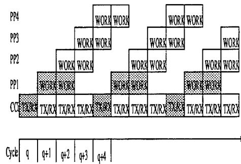
(b) Simple exchange with 4 PPs per Cluster
