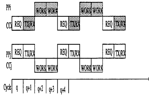
(a) Simple exchange with one PP per Cluster
