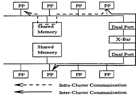
Figure 2: Proteus Communication Paths
