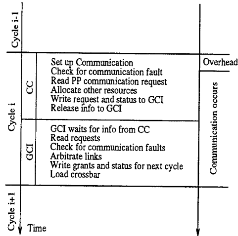
Figure 3: A Breakdown of the Proteus Communication Cycle
