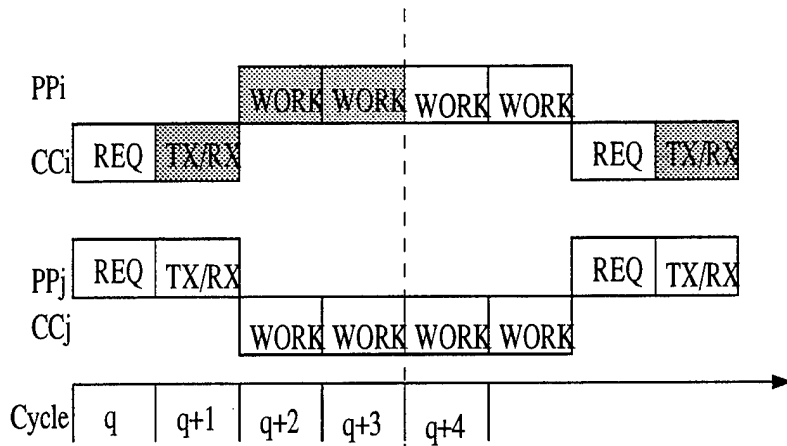
(a) Single PP with realistic workload
