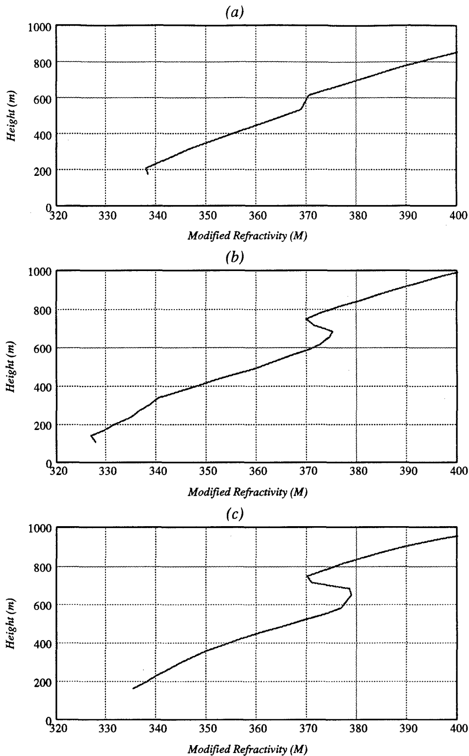
Figure 31. 12 UTC modified refractivity profiles for (a) Wilmington, (b) Wright-Patterson AFB, and (c) Circle Hill, OH on October 5, 1996.
