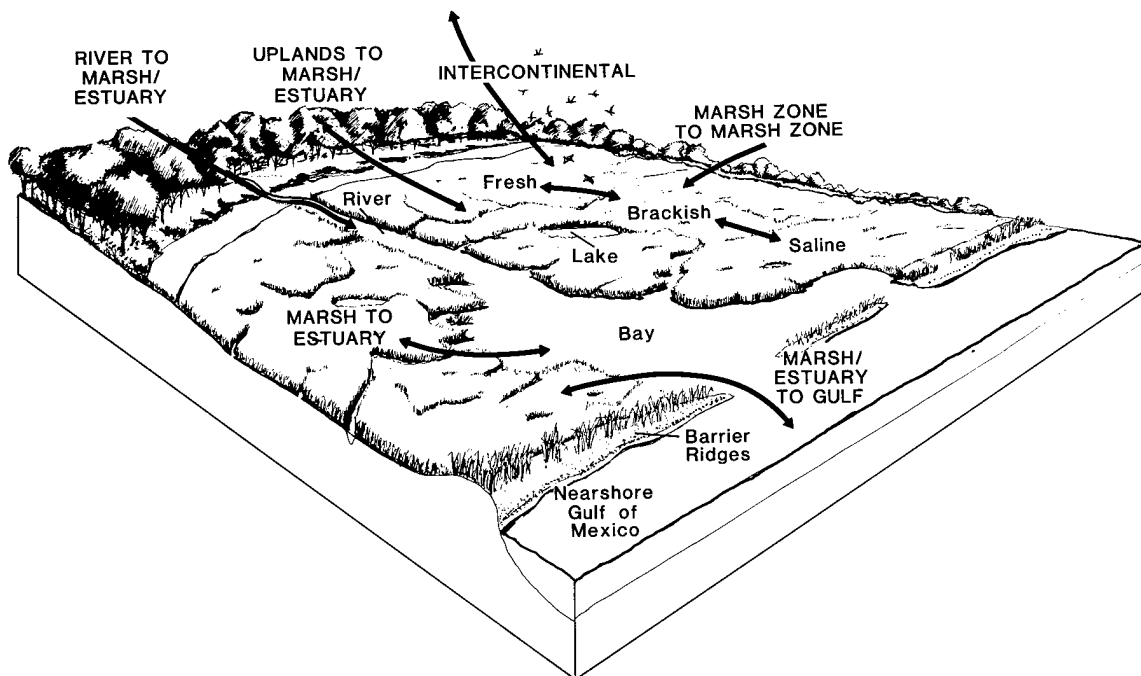
Figure 65. Conceptual diagram illustrating the coupling of delta marshes to other ecosystems.
