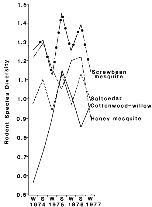
Figure 35. Rodent species diversities in four community types in the lower Colorado River Valley. Densities are calculated from the average densities (N/270 trap nights) of Peromyscus eremicus , P. maniculatus , Perognathus penicillatus , Dipodomys merriami , and Neotoma albigula caught in a given community type for a given time of year (Anderson et al. 1977).
