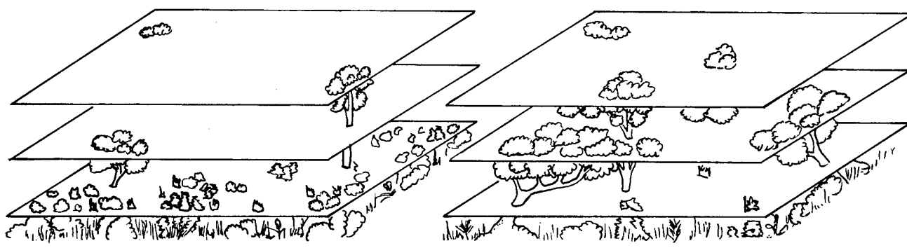
Figure A-7. Diagrammatic representation of foliage diversity (patchiness) in the horizontal plane at each of three vertical layers. The blocks represent patches of roughly 2 ha (5 acres). From Anderson and Ohmart (1984c).
