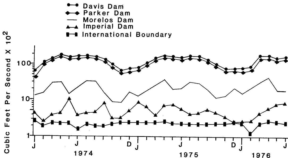
Figure 25. Patterns of monthly discharge of the lower Colorado River main-stream at various points between Davis Dam and the U.S.-Mexico Boundary, 1974 through 1976; compiled from U.S. Geological Survey. From Minckley (1979).
