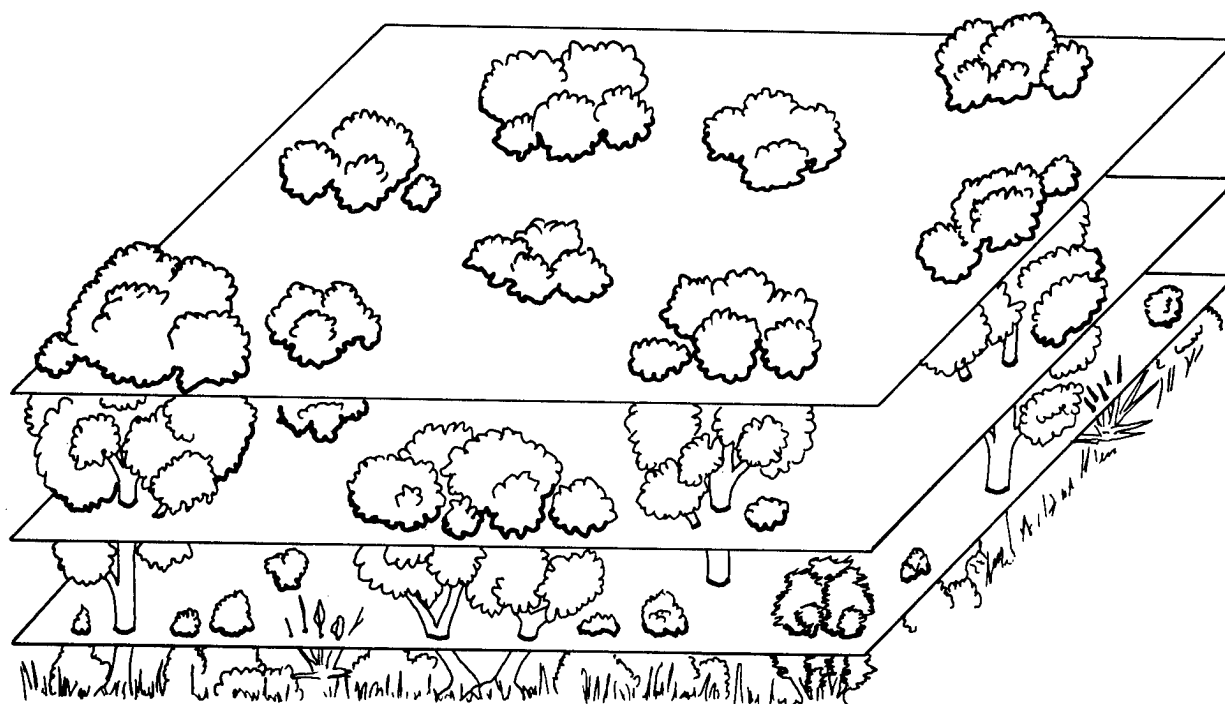
Figure A-6. Diagrammatic representation of foliage diversity in the vertical plane. The stand shown depicts an area of at least 10 ha (25 acres). From Anderson and Ohmart (1984c).
