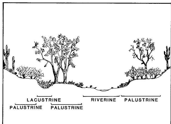
Figure A-1. Semidiagrammatic representation of wetland systems on the lower Colorado River and their designation as riverine, lacustrine, or palustrine. Adapted from Minckley and Brown (1982).
