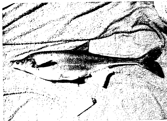
Figure 22A. Three species of Southwestern big-river fishes that were all once abundant in the lower Colorado River. Bonytail chub ( Gila elegans ) is now found only in very low numbers at Lake Mohave, while it is apparently extirpated throughout the rest of its historical range. Photo by W.L. Minckley.
