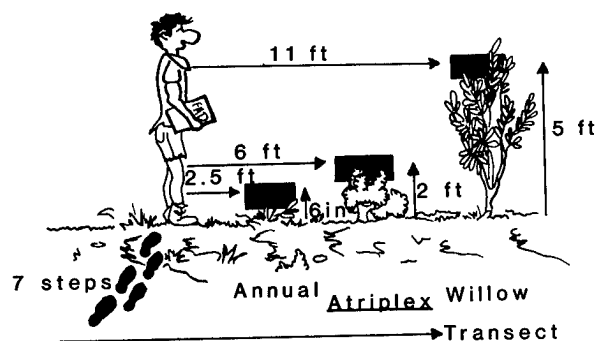
Figure A-2. Selection of vegetation for foliage density measurements. From Anderson and Ohmart (1984b).
