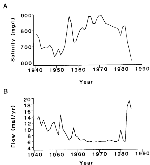
Figure 27. A. Mean annual salinity at Imperial Dam (1941-85). B. Mean annual flow at Imperial Dam (1941-85). Adapted from U.S. Department of the Interior (1987).
