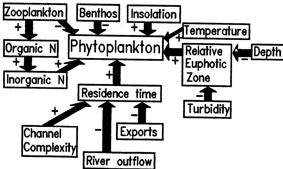
Figure 22. Conditions controlling phytoplankton abundance. Positive and negative signs indicate the effect of increasing the source element on the target element.
