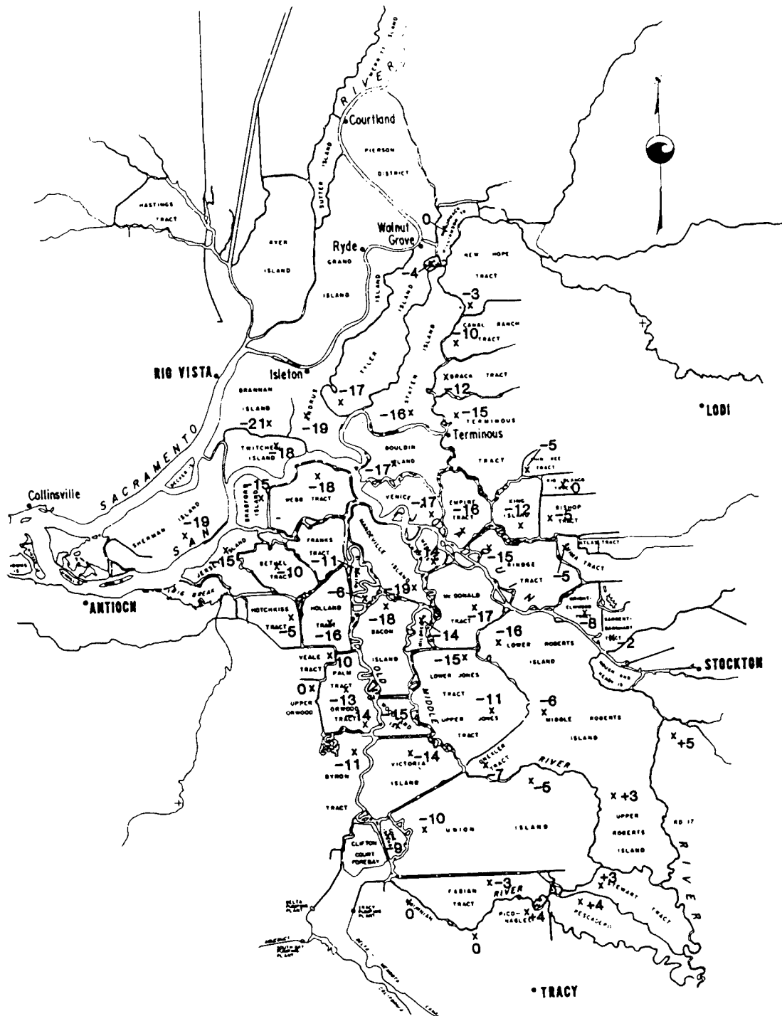
Figure 8. Depth (in feet) of subsidence in delta islands. From California Department of Water Resources (1982).
