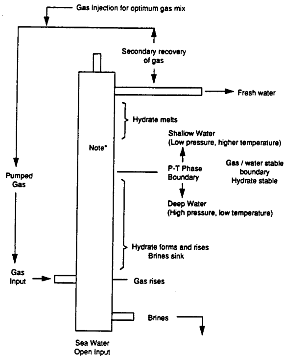
Figure 22. Diagram of desalination column to be operated in the ocean. Natural gas is pumped into the lower part of a desalination column at P-T conditions that are favorable to its forming natural clathrate in the saline water. The natural gas essentially instantly forms a clathrate and heavier brines. The clathrate rises owing to its inherent buoyancy into the upper part of the column, where it melts to release gas and fresh water. Heat produced by the process of hydrate formation is dissipated at depth by both the rising hydrate crystals and the heavier brines, which sink after cooling. A natural fractionation takes place in the column, which will have fresh water in the upper part, where it can be pumped off. Brines will sink toward the bottom of the column and dissipate into the seawater.
