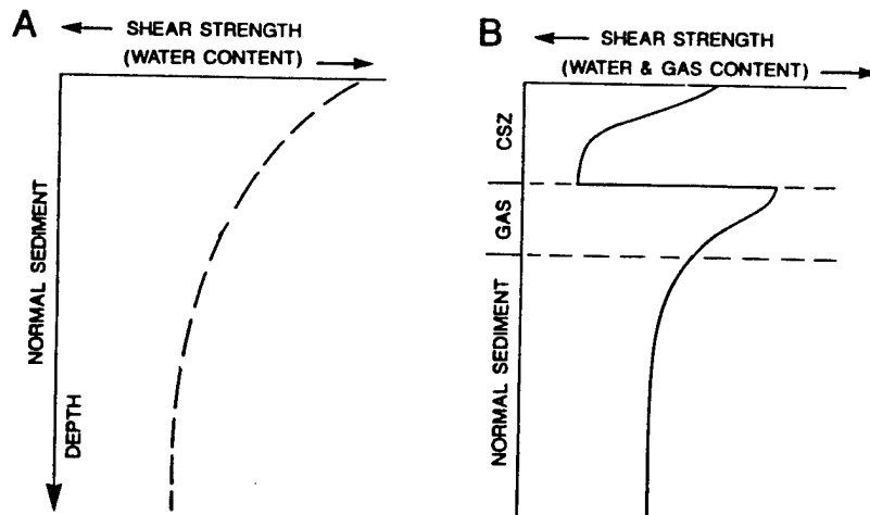
Figure 17. Shear strength profile of a generalized sediment column with clathrate trapping gas charged fluids. The position of any line showing incipient failure in relation to the generalized shear strength lines are inherently very complex, depending on sediment particle size and composition, cohesion, porosity and permeability, etc. No particular case is modeled because of the lack of detailed sediment data from the area from the surface and the underlying sedimentary succession.
