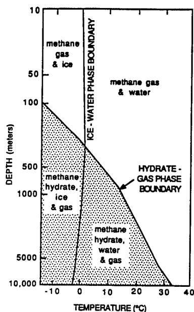
Figure 2. Phase boundary diagram of water-ice-gas-hydrate stability field for fresh water. From Kvenvolden & McMennamin (1980) and Collett (1983), attributed to redrawing from Katz et al. (1959). Addition of NaCl to water mixture shifts the curve to the left; addition of CO 2 , H 2 S, ethane, and propane to the mixture shifts the boundary to the right and increases the hydrate stability field. (10 m = 1 Atm or 1 bar at sea level. 100 Atm. or 1,470 lb/in 2 = 1 Megapascal, [MP])
