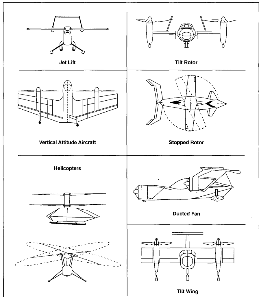
Figure 3-27 VLAR Candidate Technologies
