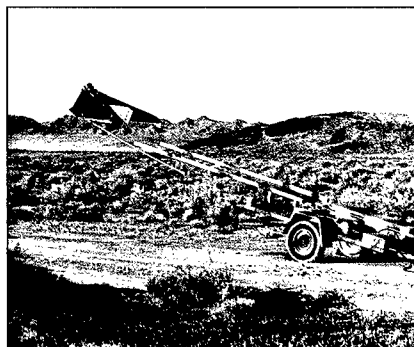
Figure 3-21 EXDRONE Rail Launch
