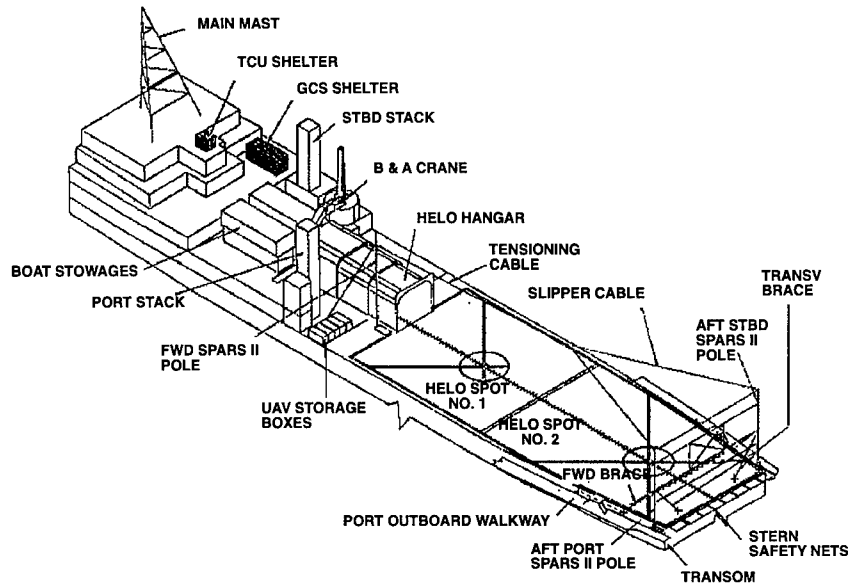
Figure 3-12 Pioneer LPD Configuration
