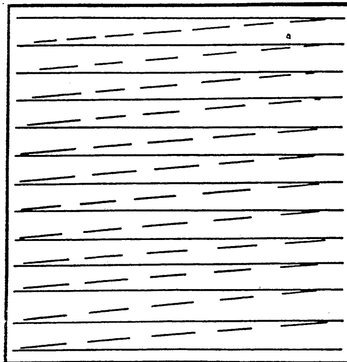
Figure 6.1 TV Raster
