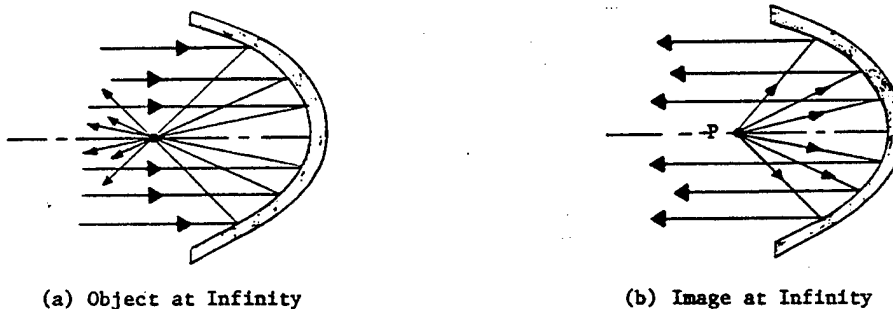
Figure 8.2.25. The Paraboloidal Mirror
