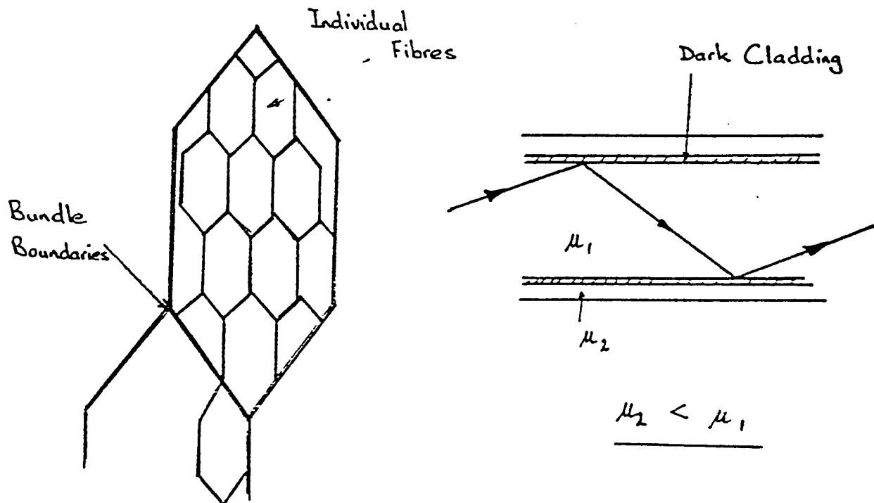
Figure 5.21 Fiber Optics
