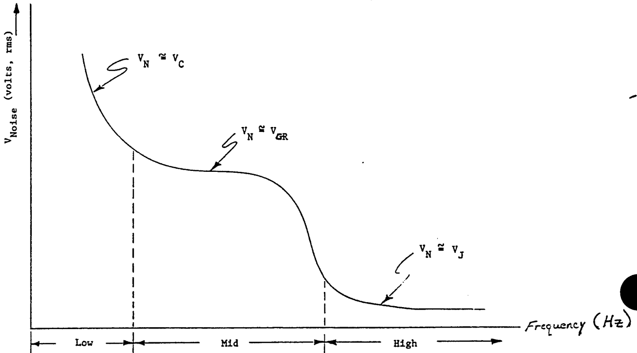
Figure 5.10 Radiation Detector Noise
