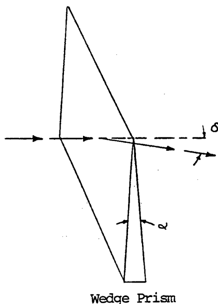
Figure 8.2.32. Beam Deviation
