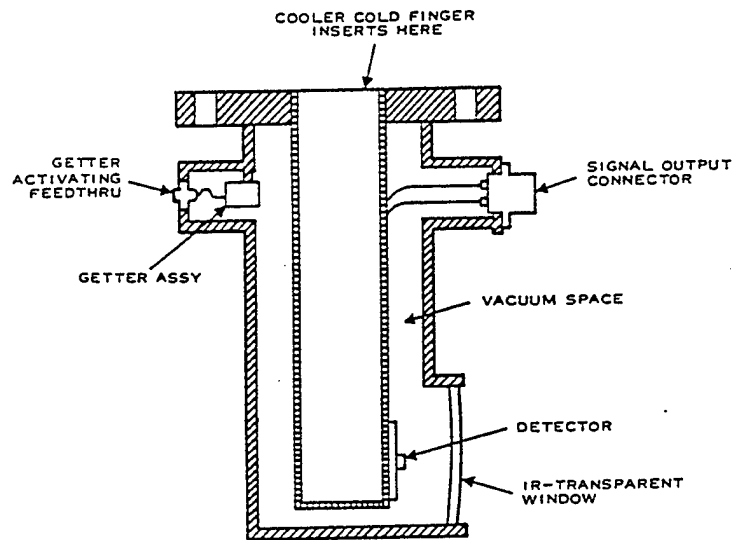
Figure 5.11 Dewar Assembly
