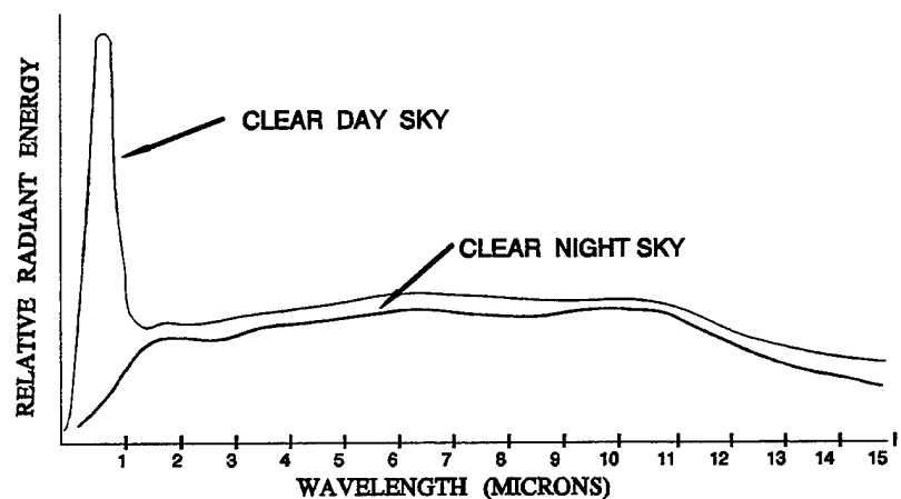
Figure 2.7 Spectral Energy Distribution of Background Radiation from the Sky
