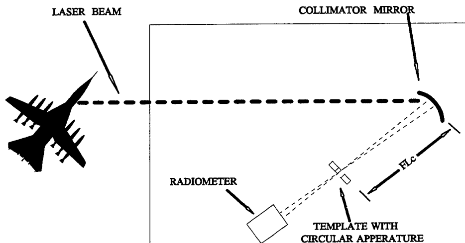
LASER BEAM DIVERGENCE TEST SETUP
