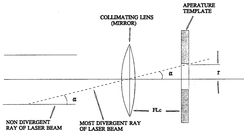
LASER BEAM DIVERGENCE TEST GEOMETRY
