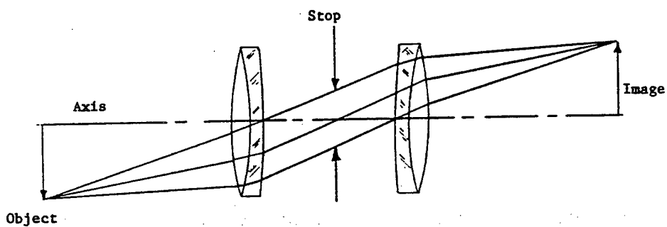
Figure 8.2.13. Correction of Lens Aberrations by the Use of Multiple Lenses of Different Refractive Index
