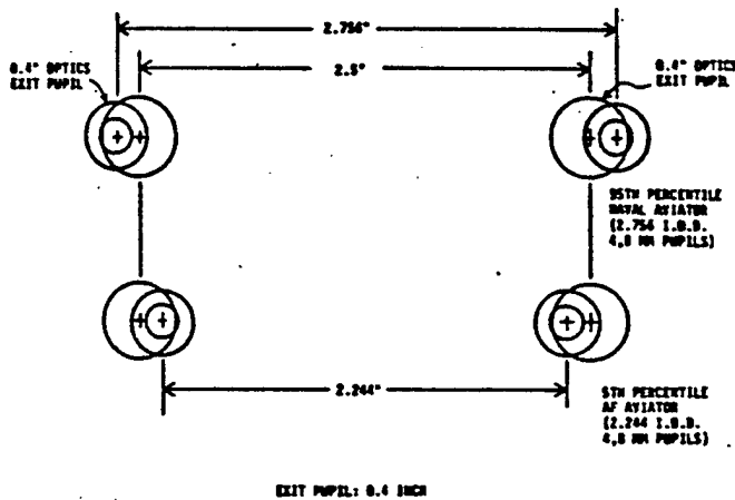
EXIT PUPIL/EYE SPACING CONSIDERATIONS (SCALE 2:1)
