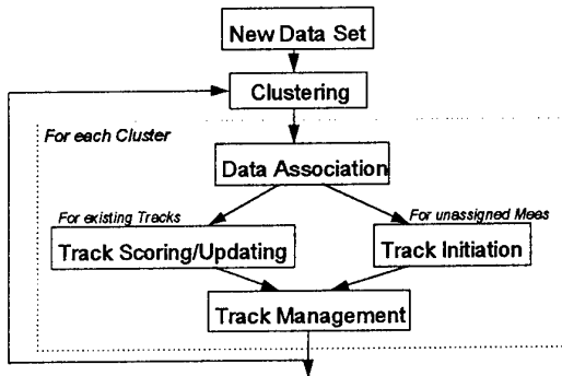
Figure 1. Algorithm Summary
