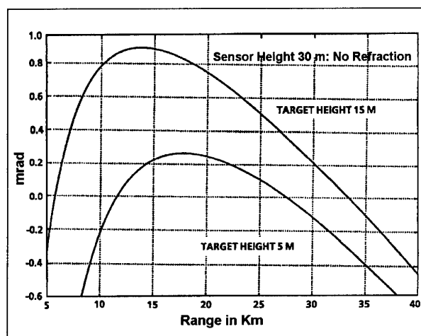
Figure 7. Threat elevation angle relative to the horizon as a function of altitude
