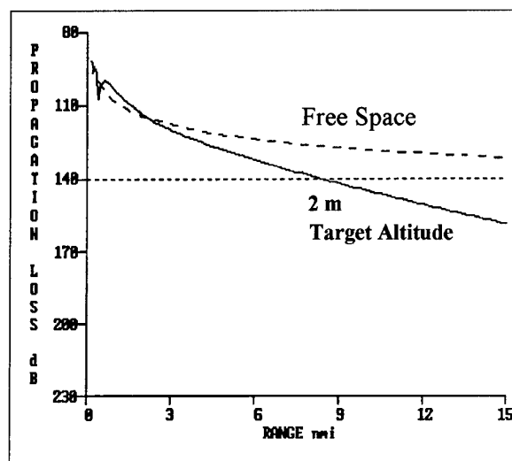
Figure 2. Propagation Loss vs. Range
