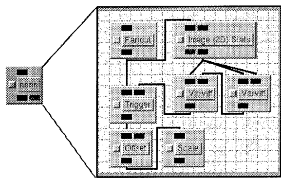
Figure 4.5 Normalization Module
