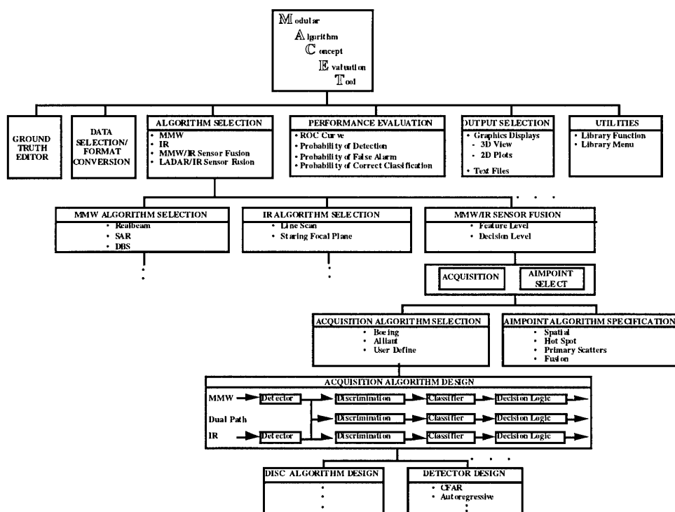
Figure 3.1-2. MACET Architecture
