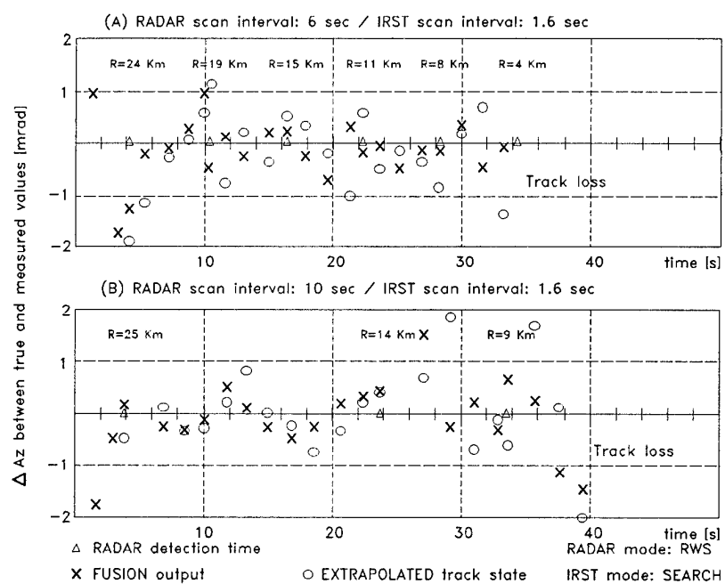
Fig 5 - RADAR to IRST Cueing
