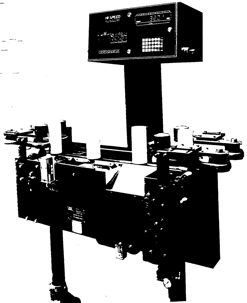
Checkmate, (shown with the Hi-Speed CM-60 Checkweigher) provides feedback to the filler.
