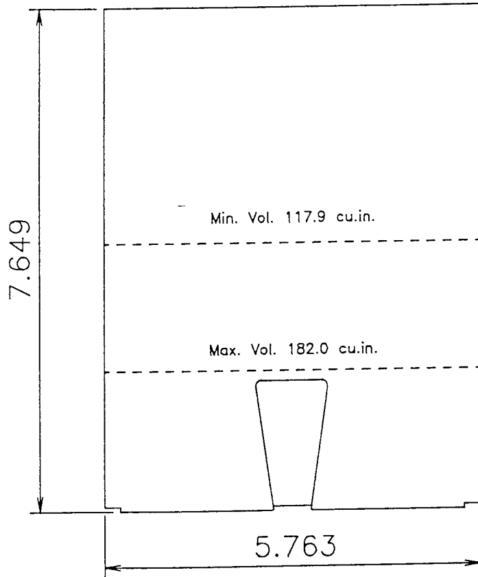
Tray Pack Transfer Cup
