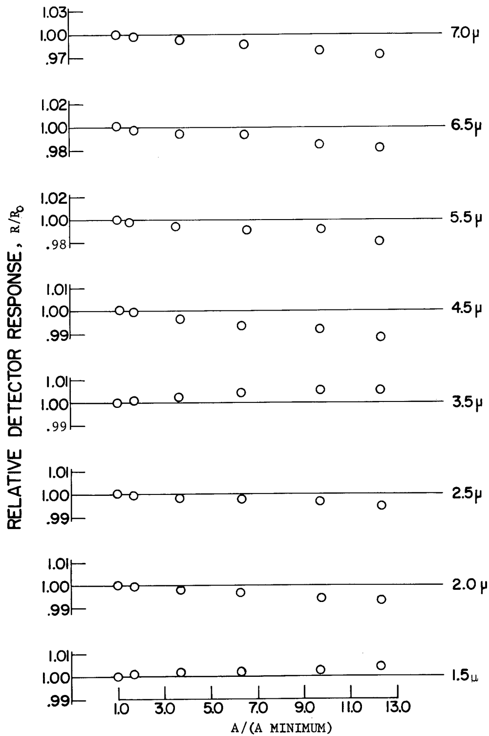
Area Sensitivity Test Results for Internal Shield With the Sulfur-Coated Sphere
