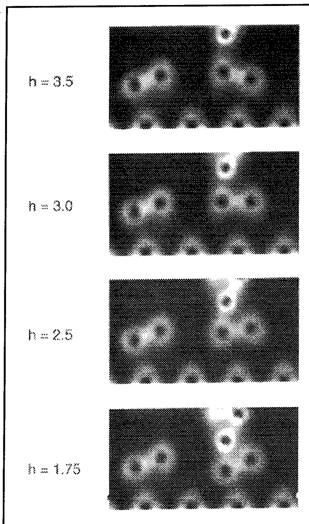
Figure 2. The sequence of charge density cross sections (from top to bottom) as the tip pulls up and flips the dimer. Same convention for h as in figure 1.
