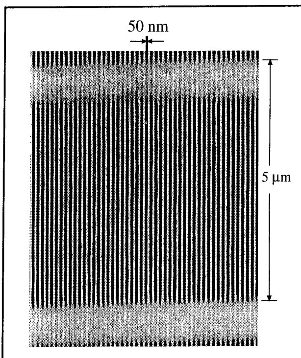
Figure 35. Scanning electron micrograph of a free-standing 100 nm period grating in a silicon nitride membrane of area 500\text{ }\mu\text{m} by 5\text{ mm} .
