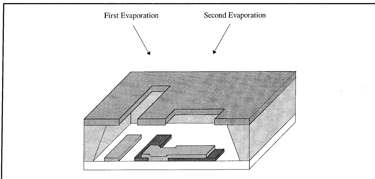
Figure 2. Double-angle evaporation schematic.
