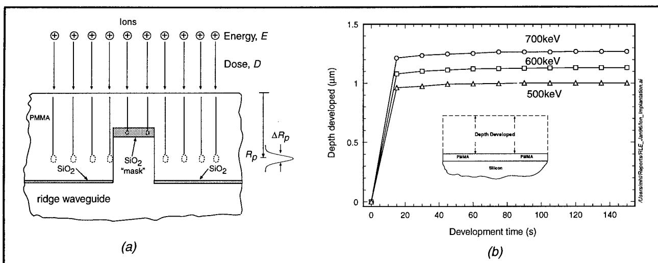
Figure 27. (a) When high energy ions are implanted, the majority of the ions stop at a particular depth governed by the energy of the ion. This allows one to develop the thick PMMA down to a thin film for x-ray exposure; (b) the depth of the developed PMMA saturates at a particular depth dependent on the energy of the implanted ion. The ion dose was 1 \times 10^{13} \text{ cm}^{-2} . The PMMA was developed in a solution of 1:2 MIBK:IPA at 21° C.
