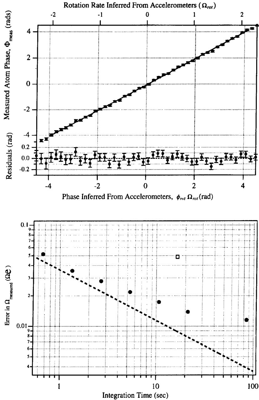
Figure 12. (a) A plot of the measured interferometer phase, \phi_{\text{meas}} , versus the inferred phase from the accelerometer readings, \phi_{\text{rot}} , from a combination of 20 second runs totaling approximately 400 seconds of data ( \sim 10 sec of data per point). There is a 0.8 percent difference between these measurements with a total error of 1 percent. (b) Reproducibility of the interferometer measurement when driven by a 4.6 Hz sinusoidal motion. The standard deviation of the fluctuations in the measured rotation of the 4.6 Hz spectral peak is plotted versus integration time (circles). This is compared to the shot noise limited error versus integration time (dashed line).
