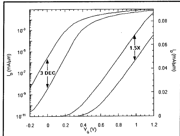
Figure 17. Subthreshold characteristics of an L_{eff}=0.2 μm device on linear and log scale showing 3 decade reduction in off current and 1.5 times increase in drive current when the threshold voltage is switched.
