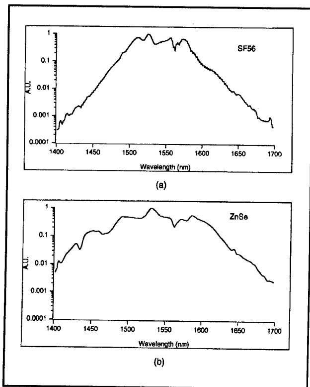
Figure 10. Continuum generated (a) in SF56 glass and (b) in ZnSe. The spectrum is displayed on a log axis normalized to the spectrum maximum and covers a spectral range of 1400 - 1700\ \text{nm} .
