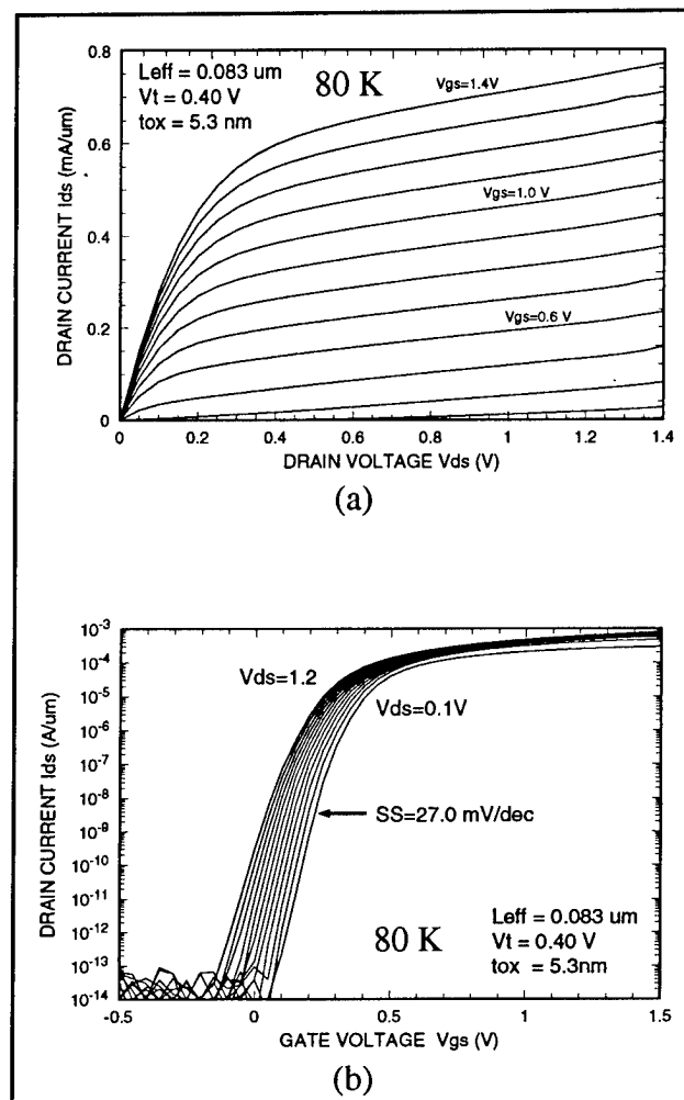
Figure 15. I-V characteristics of an 83 nm-channel-length NMOSFET cooled to 80 K.
