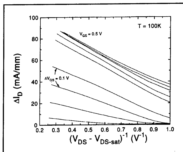
Figure 7. Kink magnitude vs. V_{DS} - V_{DS(sat)} . L_G = 0.8 \mu\text{m} .
