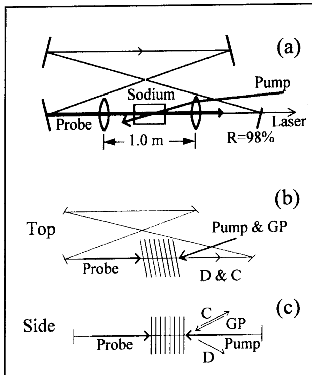
Figure 8. Schematic of experimental setup. (a) Setup for generating a strong back-propagating probe beam using a ring laser. (b) and (c) Top and side view, respectively, of setup for measuring grating diffraction efficiency.
