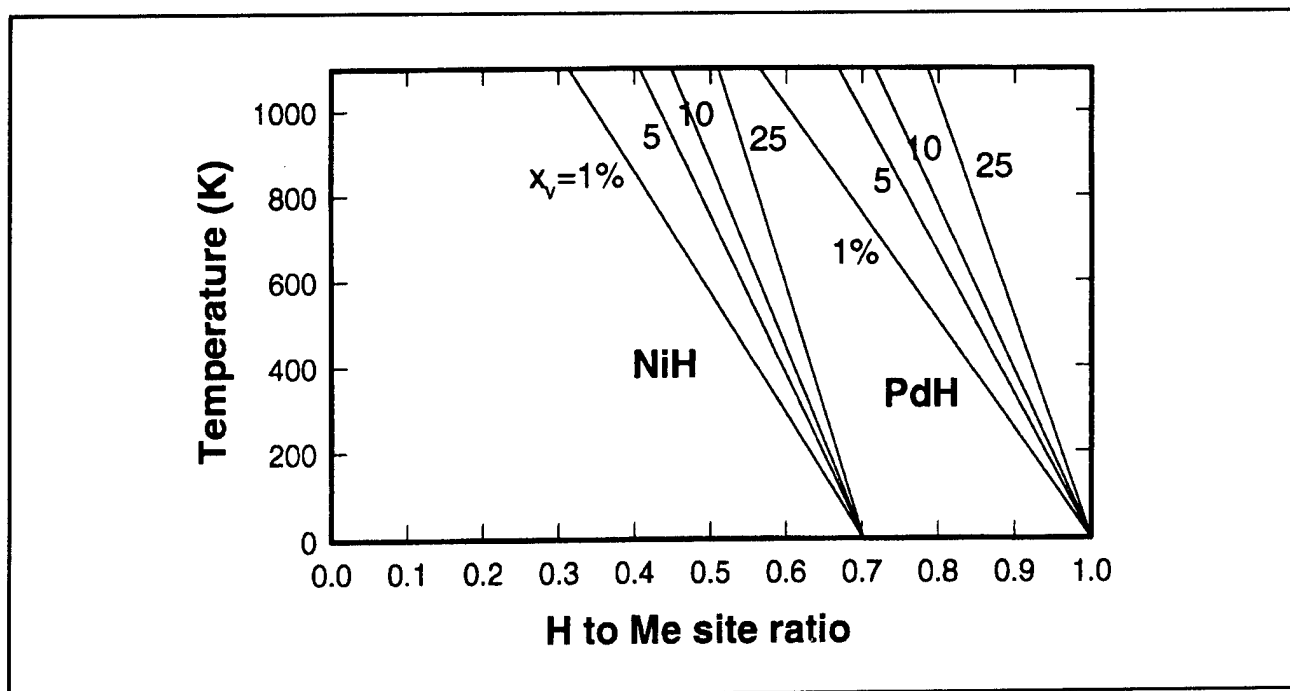
Figure 24. Estimated temperature and hydrogen loading required for the production of vacancy phase \text{Pd}_{1-x}\text{H} and \text{Ni}_{1-x}\text{H} .
