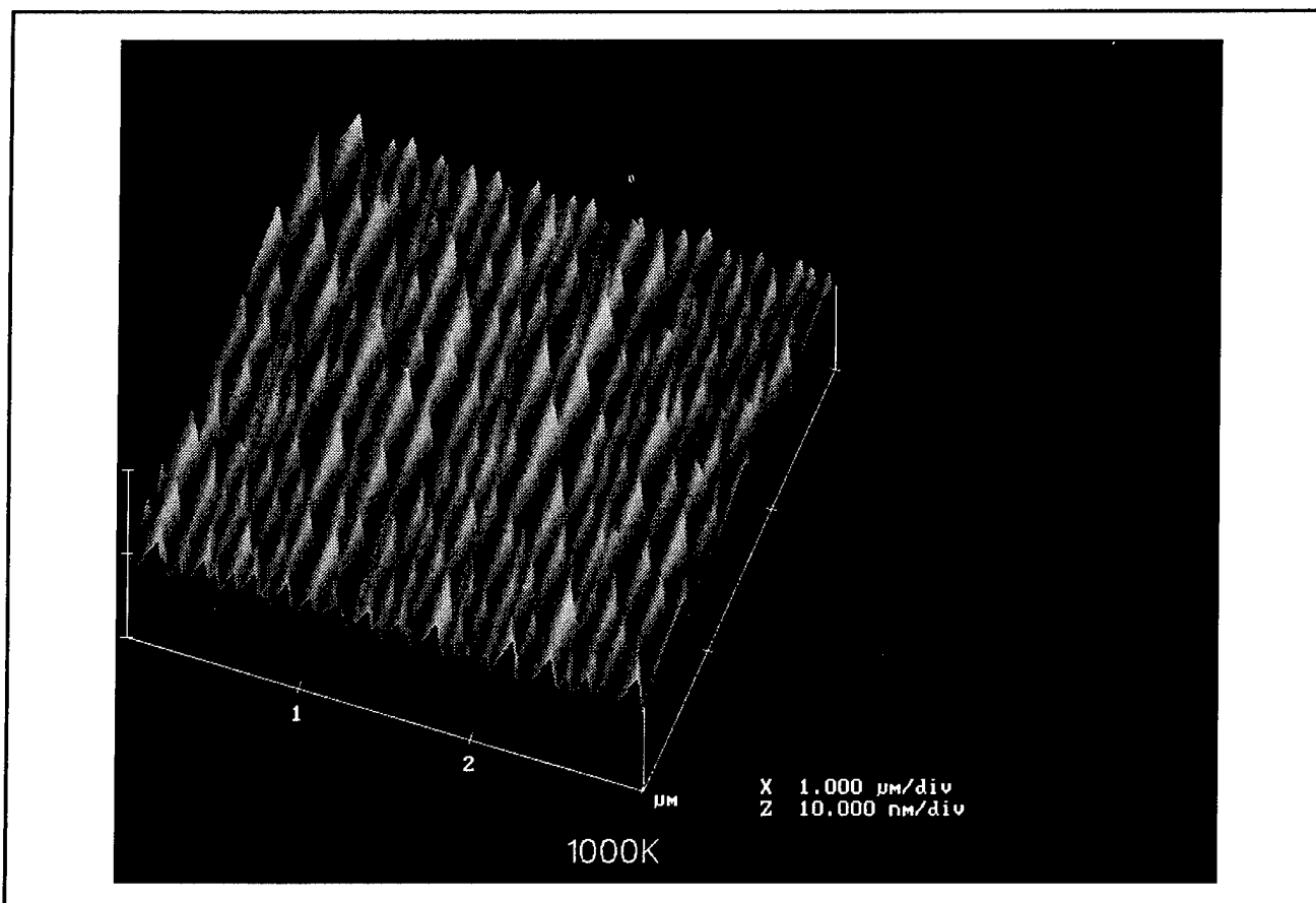
Figure 4. AFM image of the surface morphology of a stepped Si(113) surface tilted towards (\bar{1}\bar{1}0) , quenched from 900 K.
