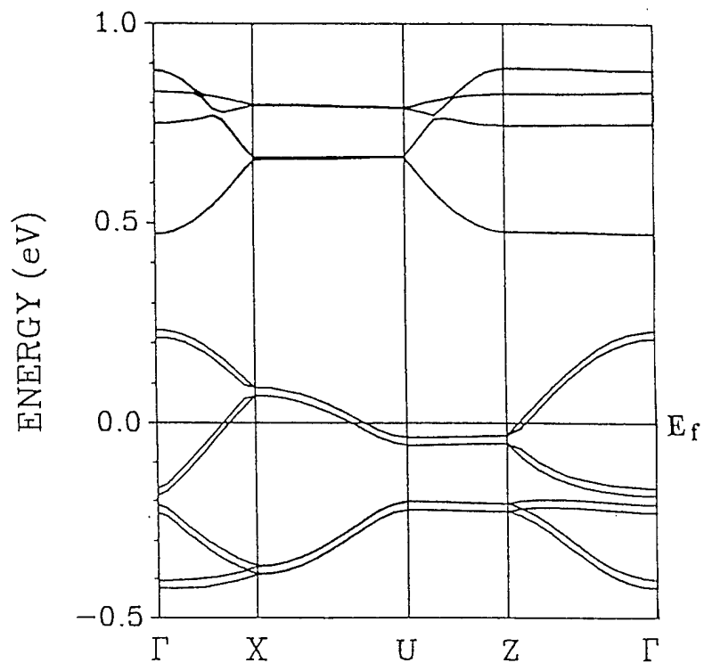
The band structures of \kappa -(ET) 2 [N(CN) 2 ]Br
