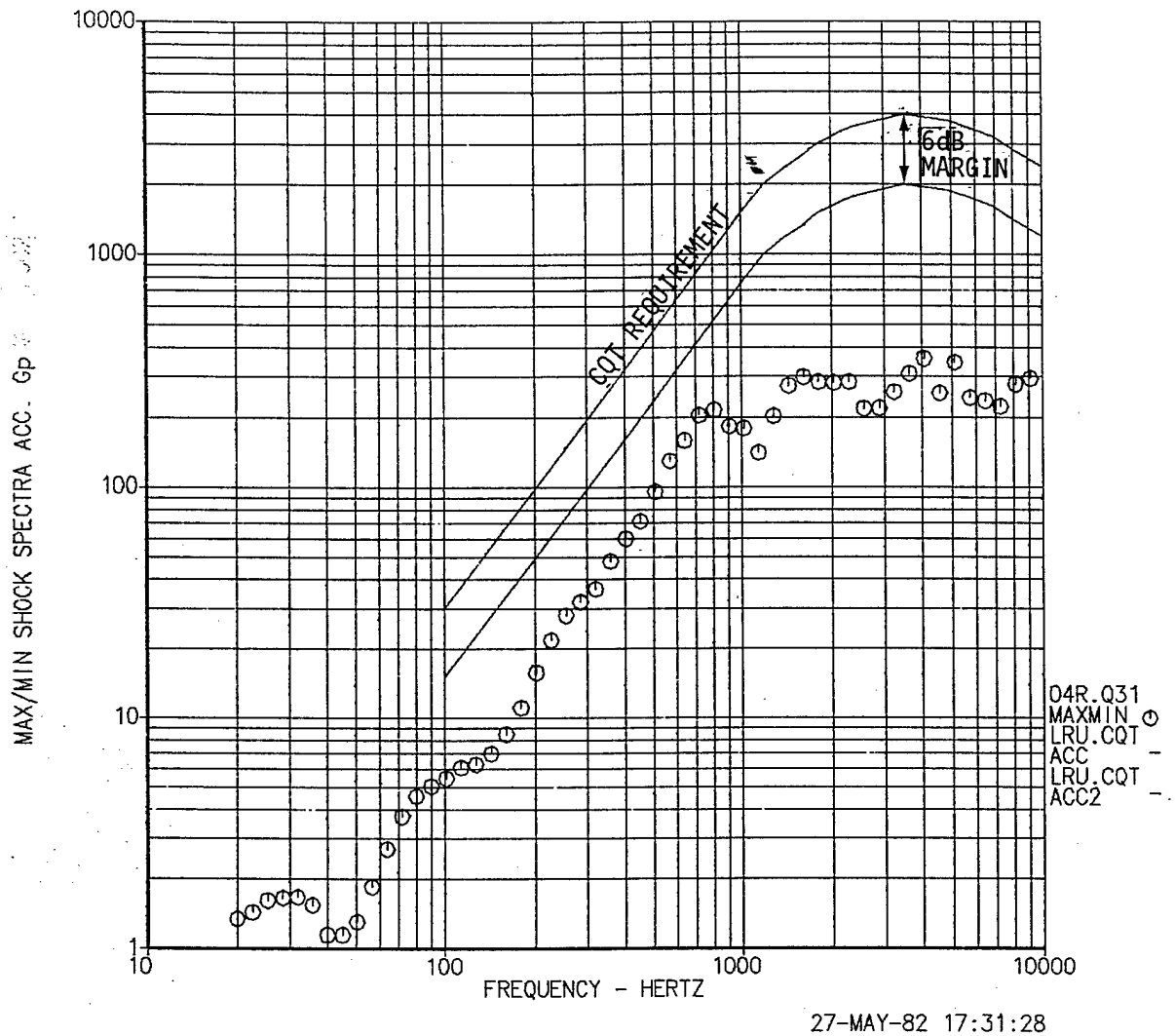
FIGURE 2-33 SHOCK SPECTRA ( Q = 10 ) H04R QTV PYROSHOCK TEST 3 PULSE 1
