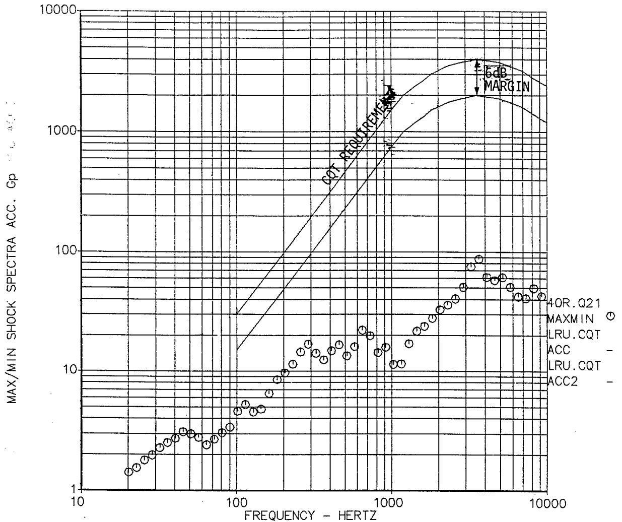
FIGURE 2-163 SHOCK SPECTRA ( Q = .10 ) H40R QTV PYROSHOCK TEST 2 PULSE 1
