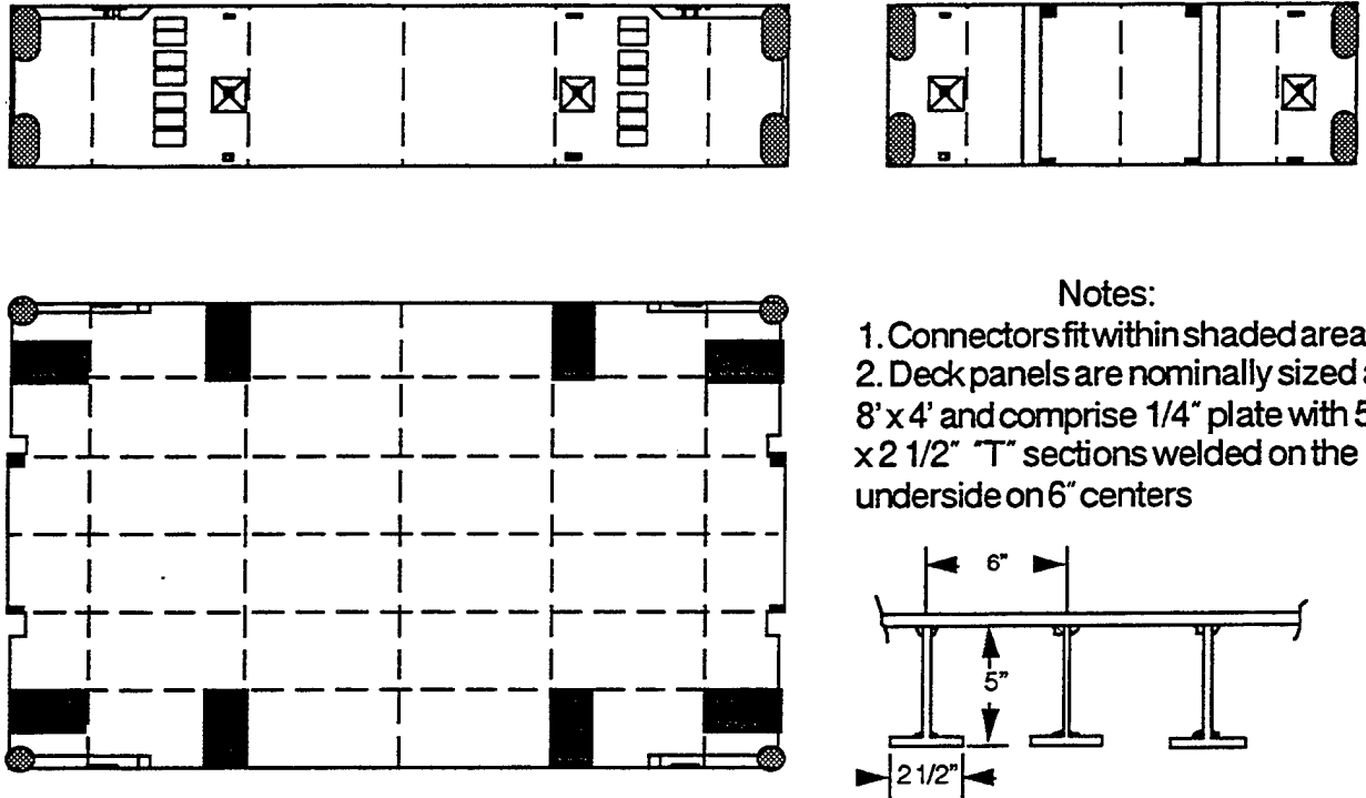
Figure 3-5. ACB Lighter deck layout with 48 x 96-inch frame spacing
