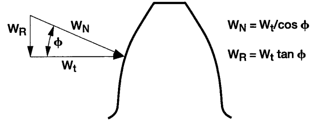
Figure 3.—Gear tooth profile showing normal load W_N .
