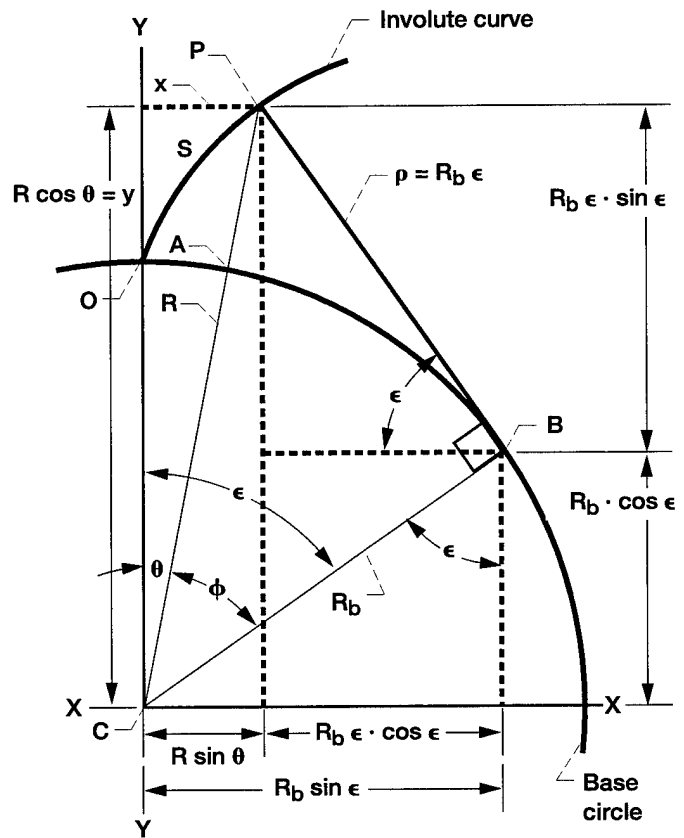
Figure 1.—Involute curve geometry.
