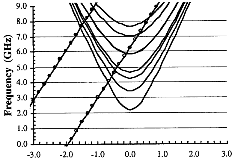
Figure 1. Dispersion curve showing the backward wave intersections for the fundamental (line with open circles) and second harmonics (line with solid circles) for (solid lines from bottom to top) TE 11 , TE 21 , TE 01 , TE 31 , TE 41 (TE 12 ), TE 51 , and TE 02 . Note that the TE 41 and TE 12 are indistinguishable, since the Bessel zeros are 5.3176 and 5.3314, respectively. Parameters: V=400 kV, I = 2 kA, B = 4 kG, \alpha = 0.7 .
