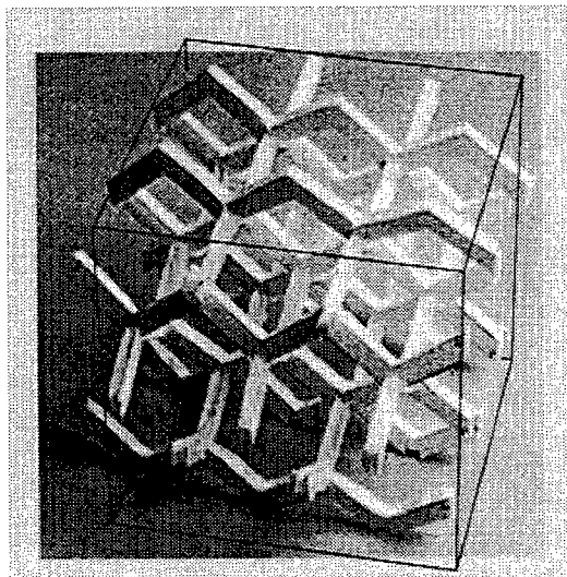
Figure 7. 3-D diamond lattice, wire mesh PBG structure.
