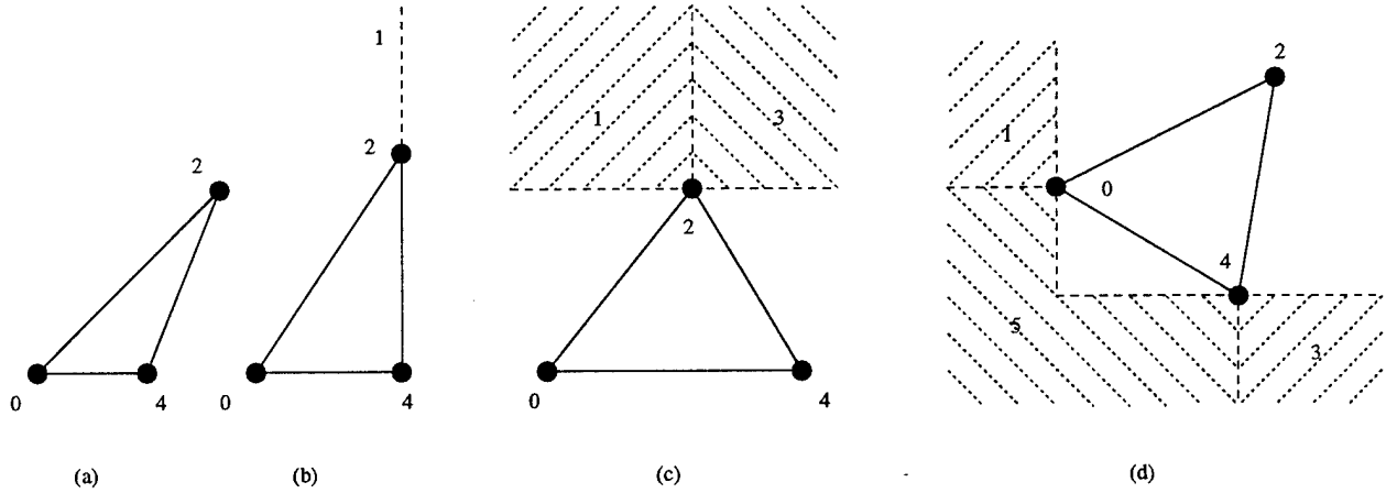
Figure 8: Illustration for Lemma 4.2.
