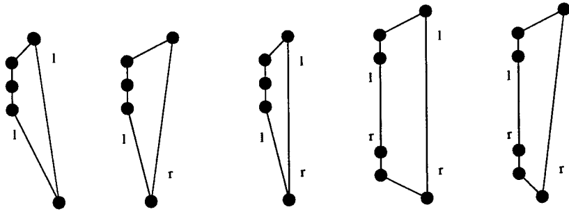
Figure 14: Drawings for face F_i for 0 < i < t .
