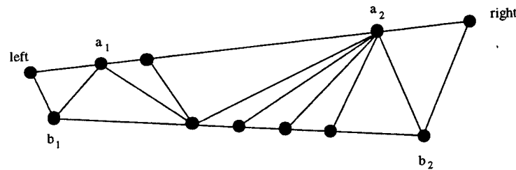
Figure 6: How to draw a maximal outerplanar open RID graph.
