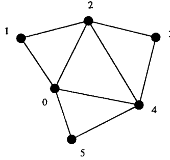
Figure 7: A non-open RID outerplanar graph.
