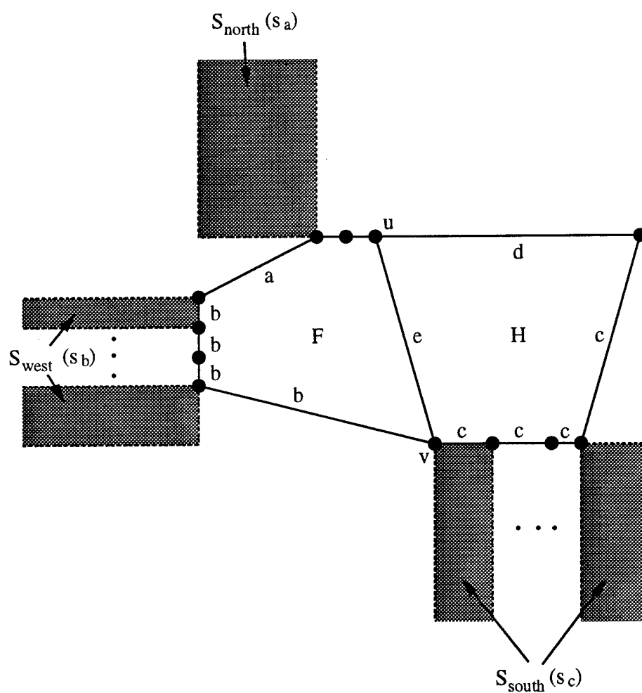
Figure 17: Face F corresponding to the dual vertex of degree 3. All possibilities for the placement of labels b and c are shown.
