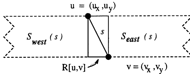
Figure 11: Strips for segment s .
