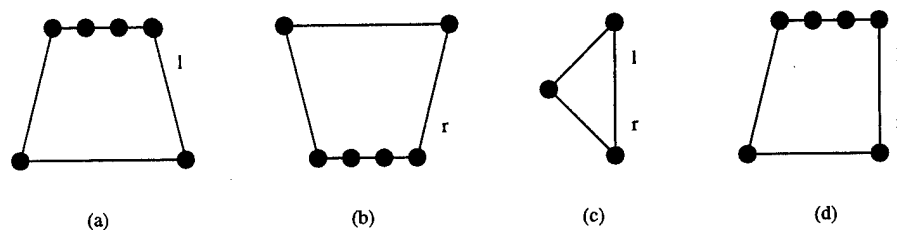
Figure 13: Drawings for face F_0 .
