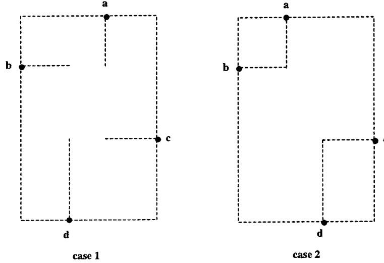
Figure 10: Figure for Theorem 4.4.
