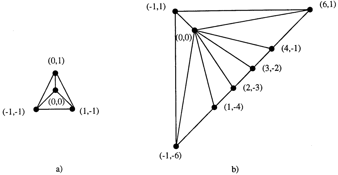
Figure 4: Illustration for Theorem 4.1 for a) n = 4 and b) n = 8 .
