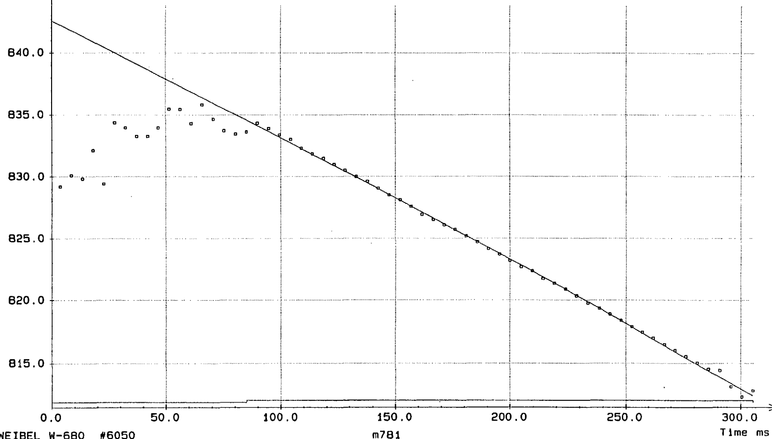
Figure C-1. Velocity vs. time plot for round 33165.
