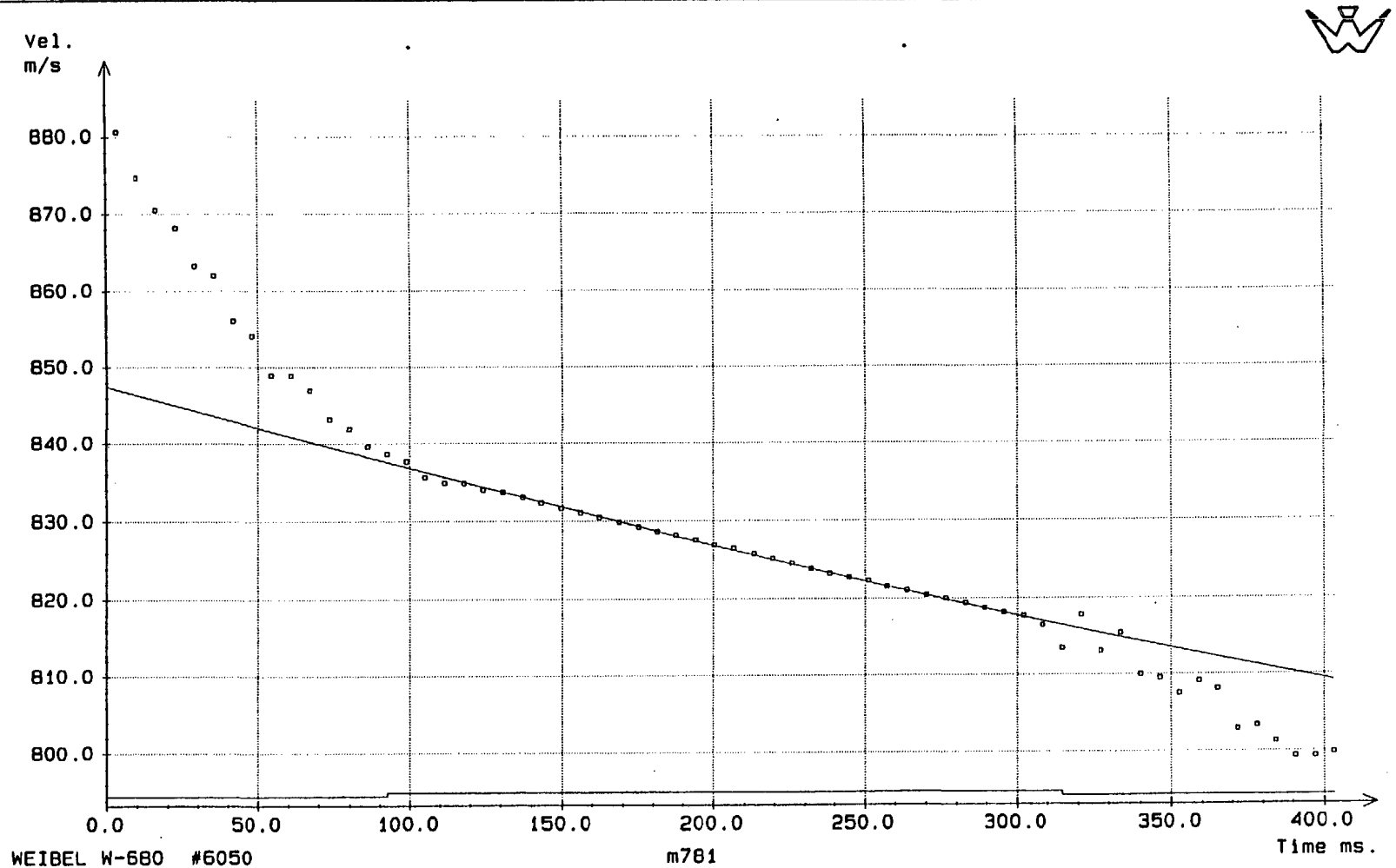
Figure C-2. Velocity vs. time plot for round 33166.
