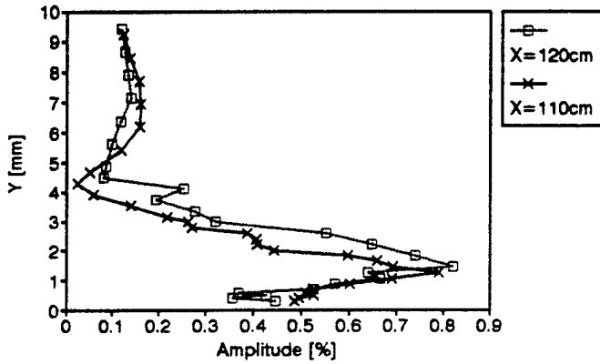
HPS Amplitude vs Y-Loss of Coherence X_p=50\text{cm}, Z_p=-4\text{cm}, Z=Z_p , High Amp
