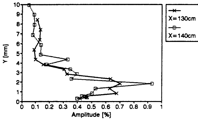
THPS Amplitude vs Y-Loss of Coherence X_p=50\text{cm}, Z_p=+4\text{cm}, Z=0 , High Amp
