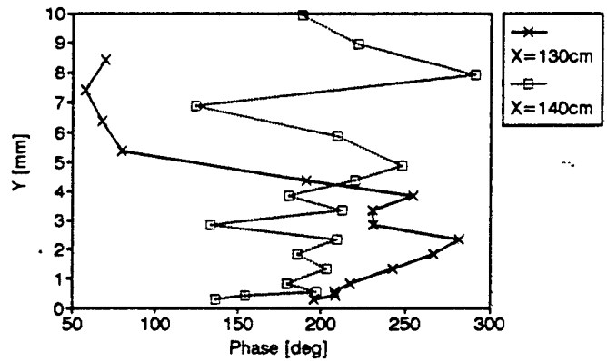
THPS Phase vs Y-Loss of Coherence X_p=50\text{cm}, Z_p=+4\text{cm}, Z=0 , High Amp
