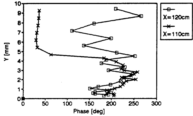
HPS Phase vs Y-Loss of Coherence X_p=50\text{cm}, Z_p=-4\text{cm}, Z=Z_p , High Amp
