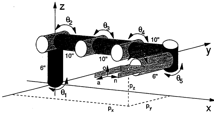
Figure 1. Six degree-of-freedom elbow manipulator.
