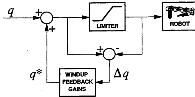
Figure 2. Robot joint commands with Windup Feedback compensation.
