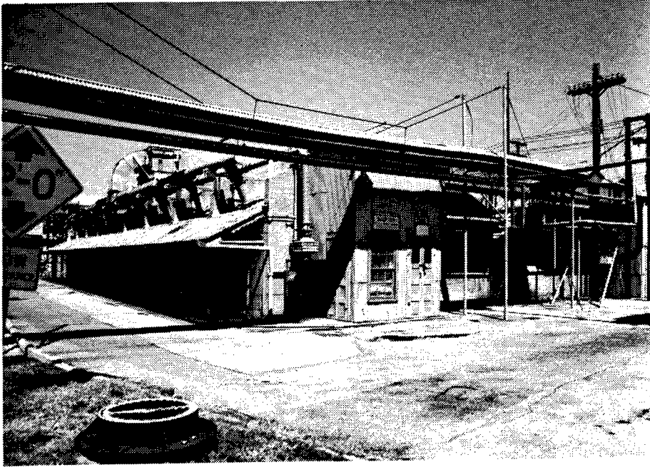
Figure 56. Building 1508: Mix House with an uncovered walkway connecting the two halves of this Mix House. Each half contains eight bays.
