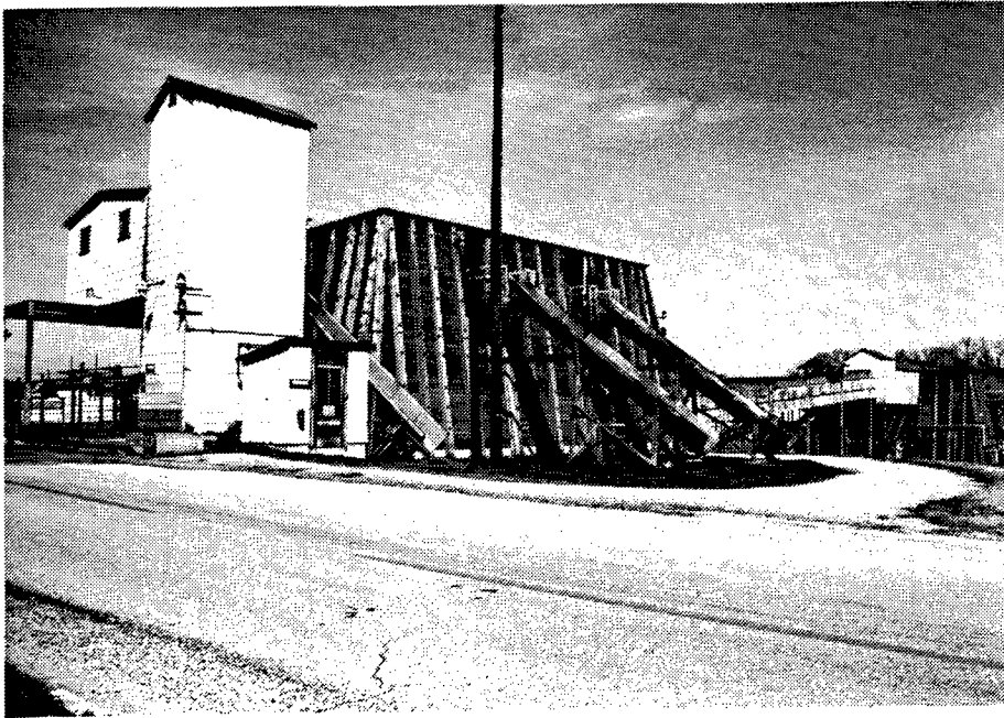
Figure 95. Building 1825 and Building 1875: The Final Blend House (foreground is Building 1825) is connected to the Can Pack House (Building 1875) by a conveyor system.
