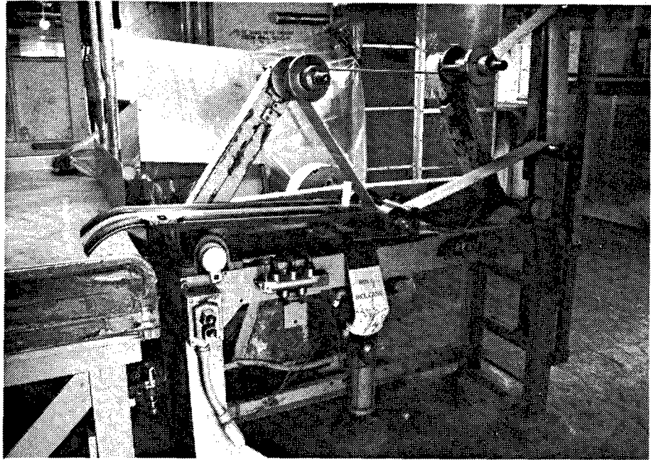
Figure 120. Building 9309-03: Carpet Roller in Rolled Powder House #4.
