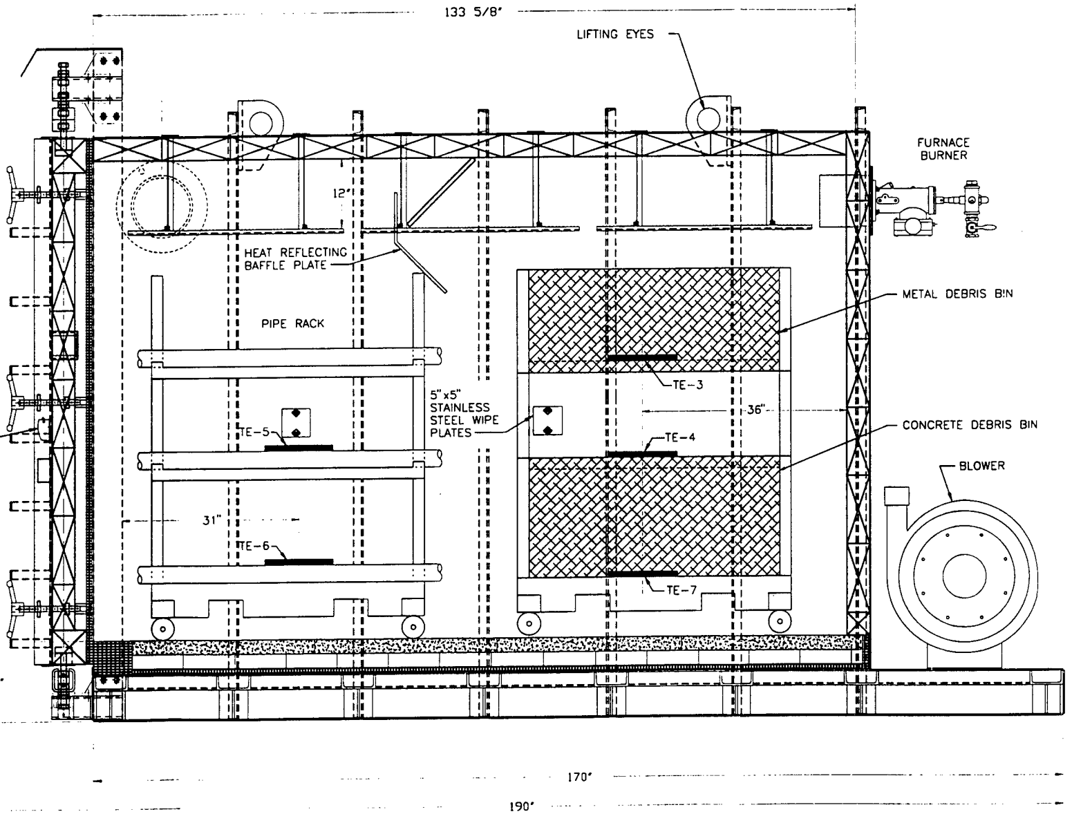
SIDE VIEW/SECTION
