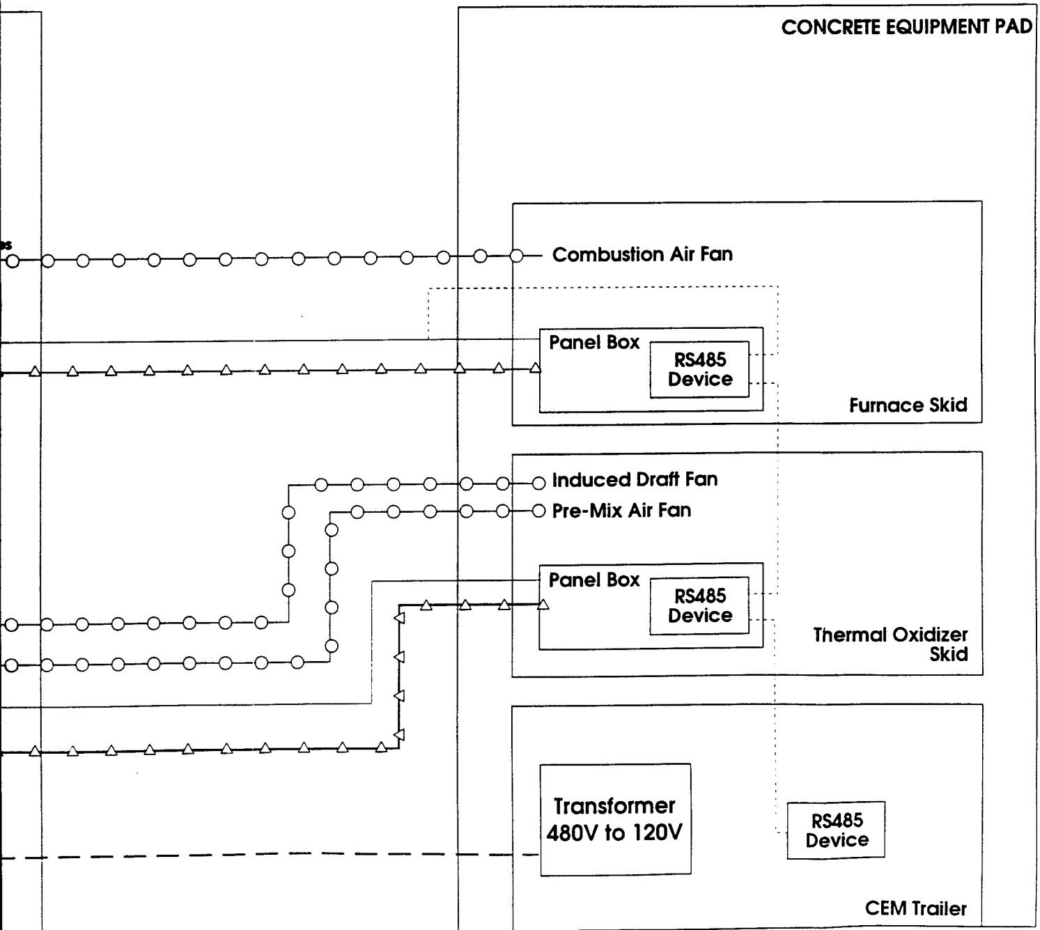
FIGURE 3-5 INTERCONNECTION W
