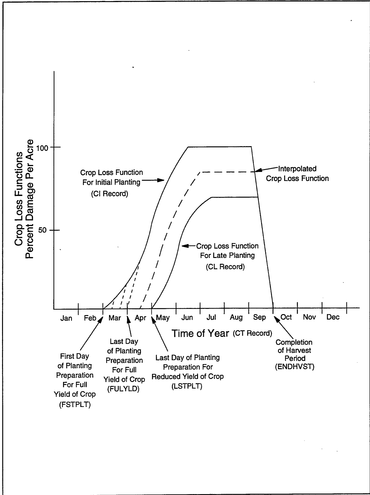
FIGURE 7 Crop Loss Analysis Concepts
