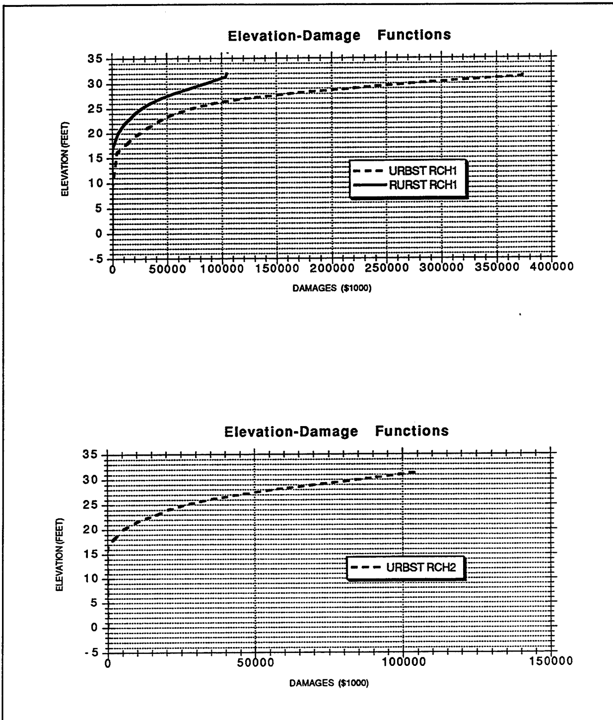
FIGURE C.3 Elevation-damage Functions for Reach 1 and Reach 2 of the Tulsa Data Set
