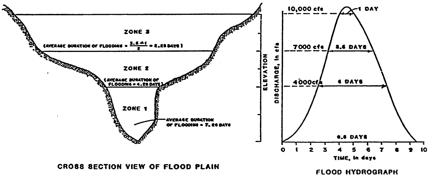
FIGURE 11 Flood Zone Concepts
