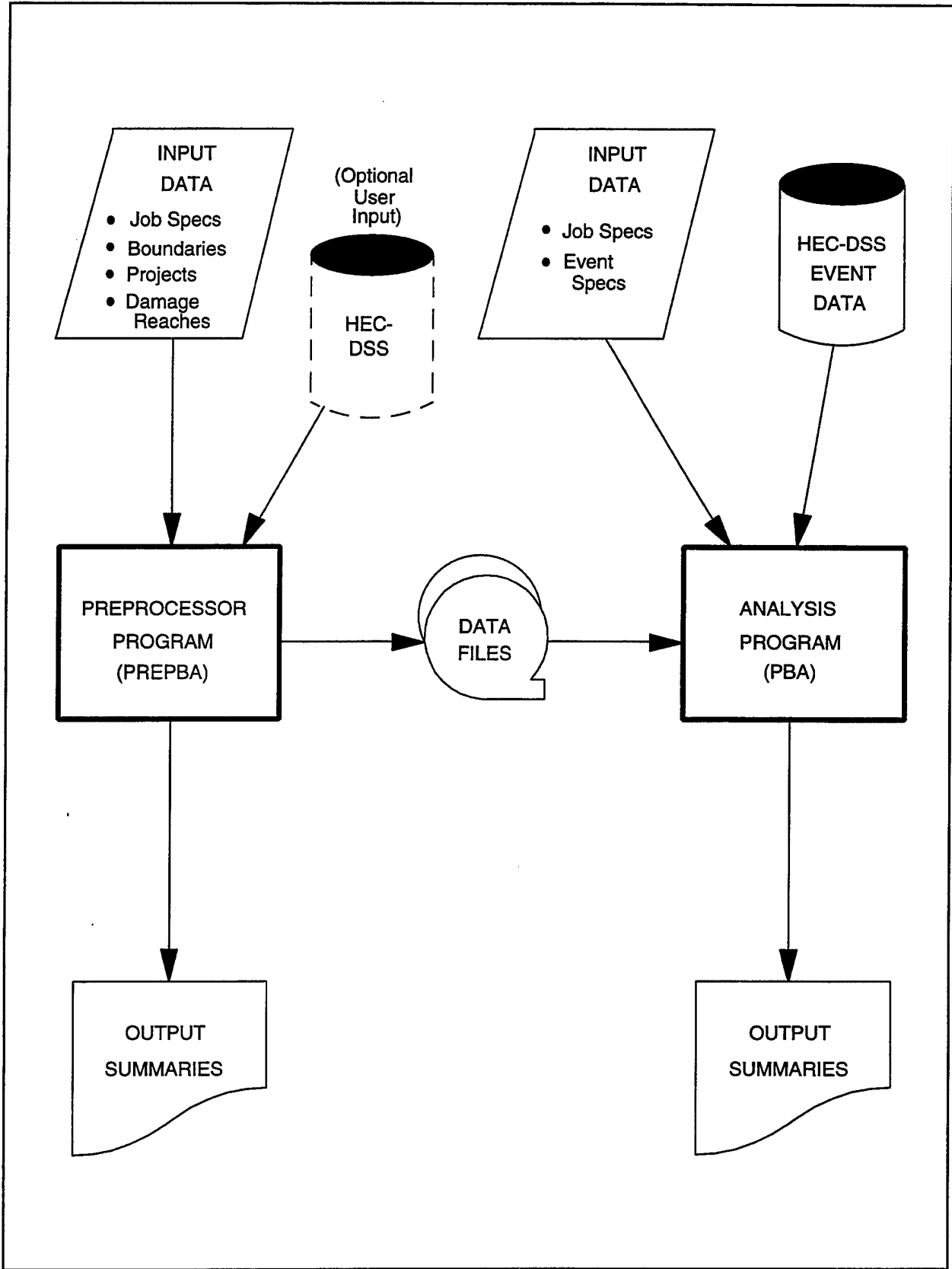
FIGURE 1 Project Benefit Accomplishment Package (HEC-PBA)
