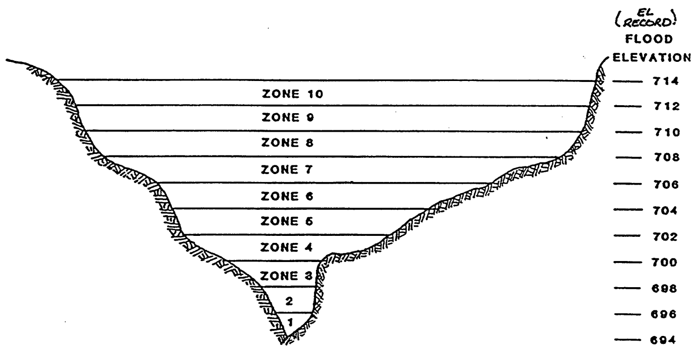
FIGURE 12 Flood Zone Computation Intervals
