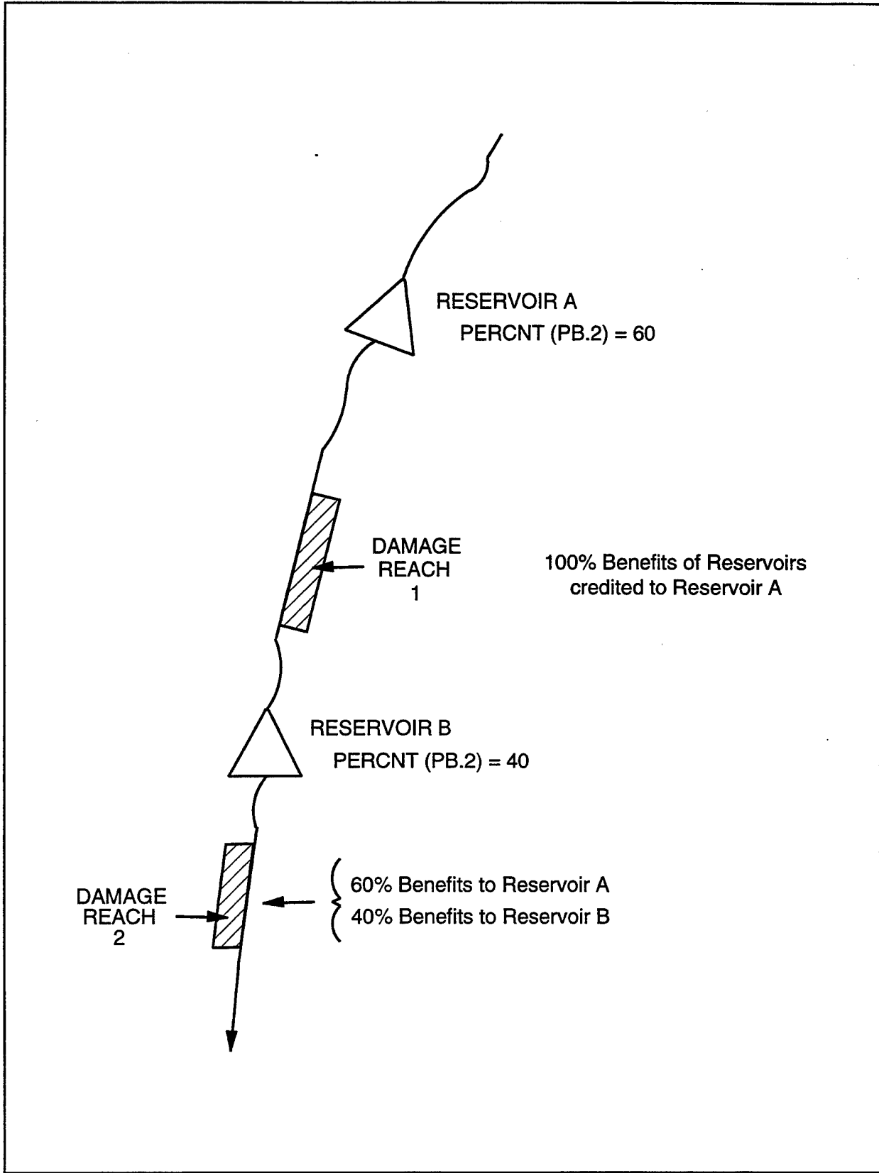
FIGURE 16 Reservoir Benefit Allocation Concepts
