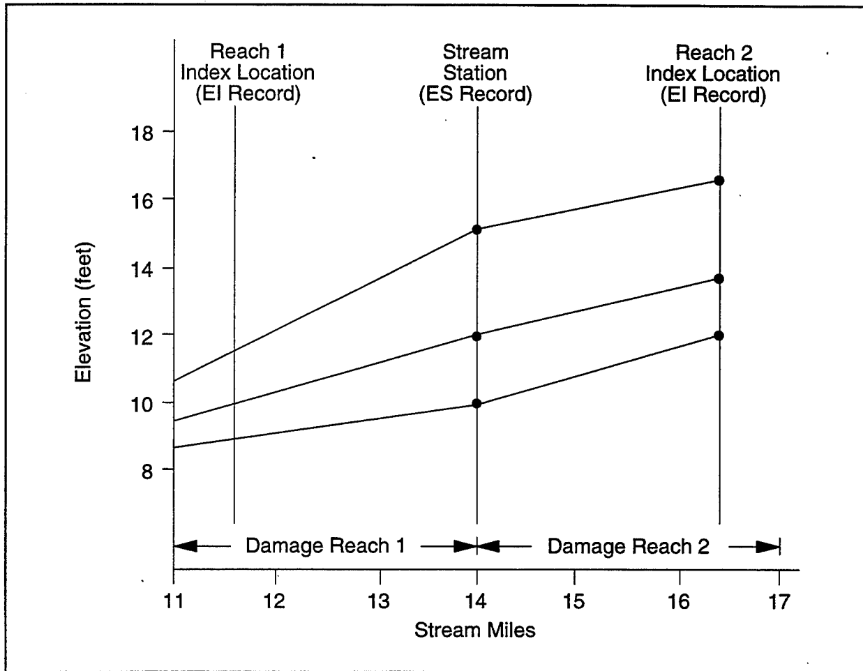
FIGURE 9 Transfer Relationships Between a Stream Station and Two Index Locations
