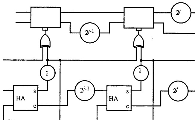
FIGURE 7. Eliminating 3dB couplers with modified control
