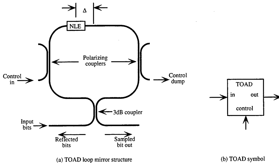
FIGURE 8. TOAD gate structure and symbol
