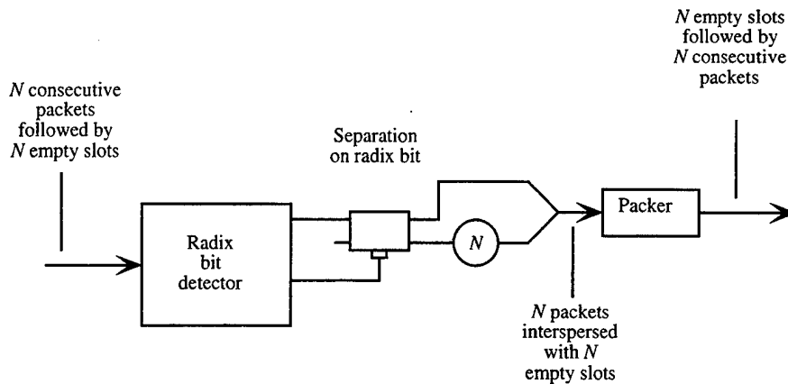
FIGURE 3. Sorter Stage for One Radix Bit
