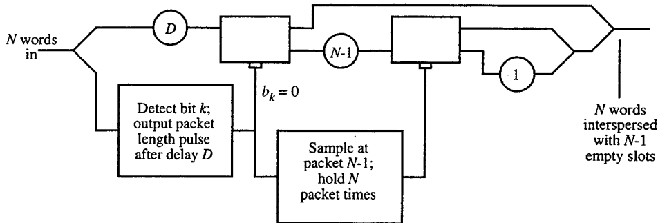
FIGURE 6. Smart append for length 2N-1 sparse stream
