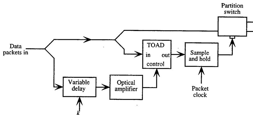
FIGURE 9. Devices making up the radix bit partition section
