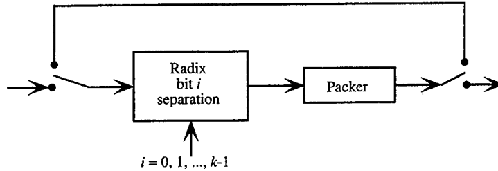
(b) Serial recirculating radix sorter
