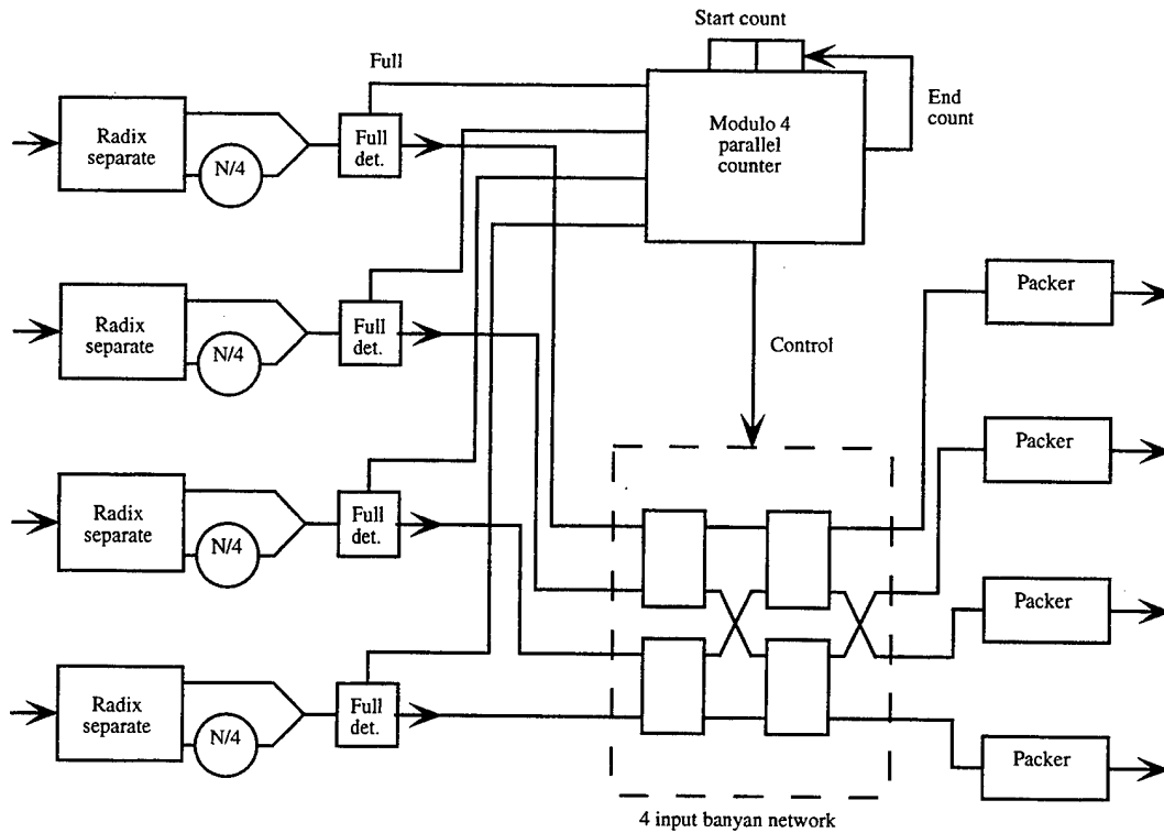
FIGURE 11. Space-time radix sorter stage with 4 parallel channels
