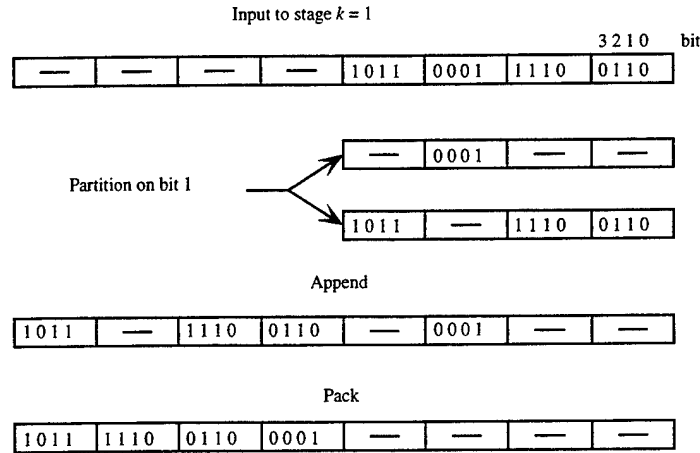
(a) Single radix bit separation and packing
