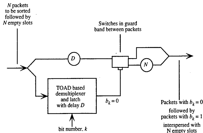
FIGURE 4. Separation on One Radix Bit
