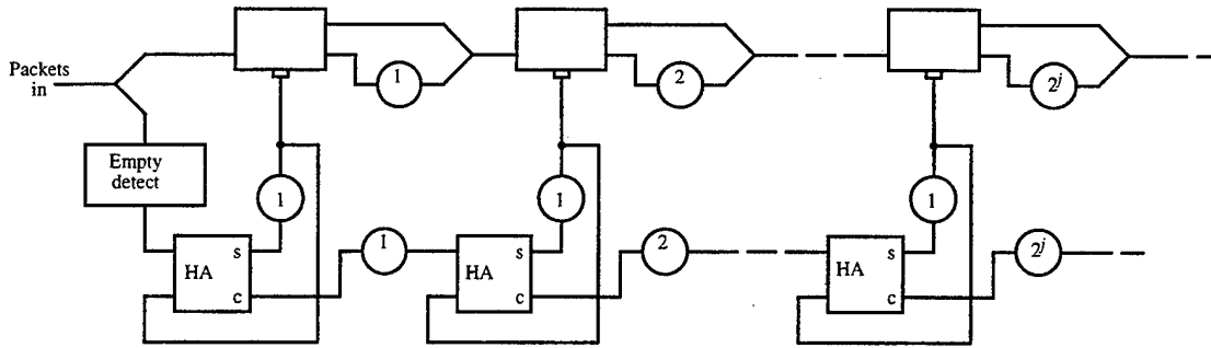
FIGURE 5. The packer line and its control
