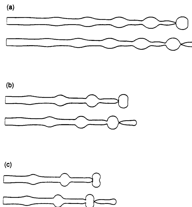
FIG. 4. Effect of inflow velocity disturbance magnitude, We = 100 , k = 0.70 , (a) q' = 2\% , (b) q' = 4\% , (c) q' = 6\% .
