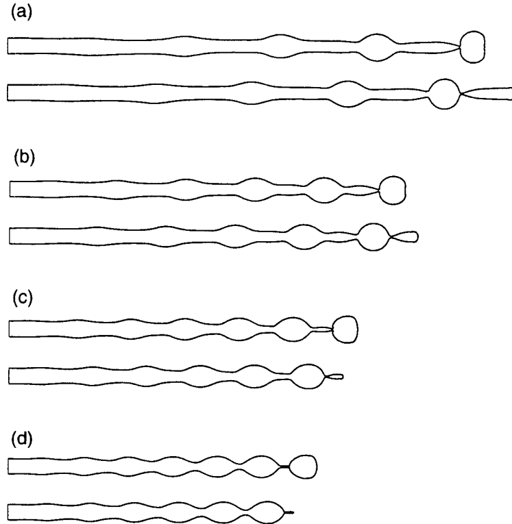
Figure 3: Effect of Longitudinal Disturbance Frequency on Behavior of Liquid Jet at We = 100 , q' = 2\% . (a) \omega/\omega_g = 0.71 , (b) \omega/\omega_g = 1.0 , (c) \omega/\omega_g = 1.29 , (d) \omega/\omega_g = 1.57
