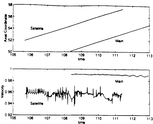
FIG. 10. Droplet center of mass position and velocity ( We = 100 , k = 0.7 , q' = 2\% ).
