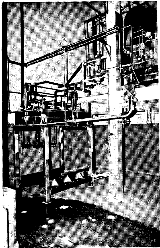
Figure 66. Building G-12: Loading machine.
