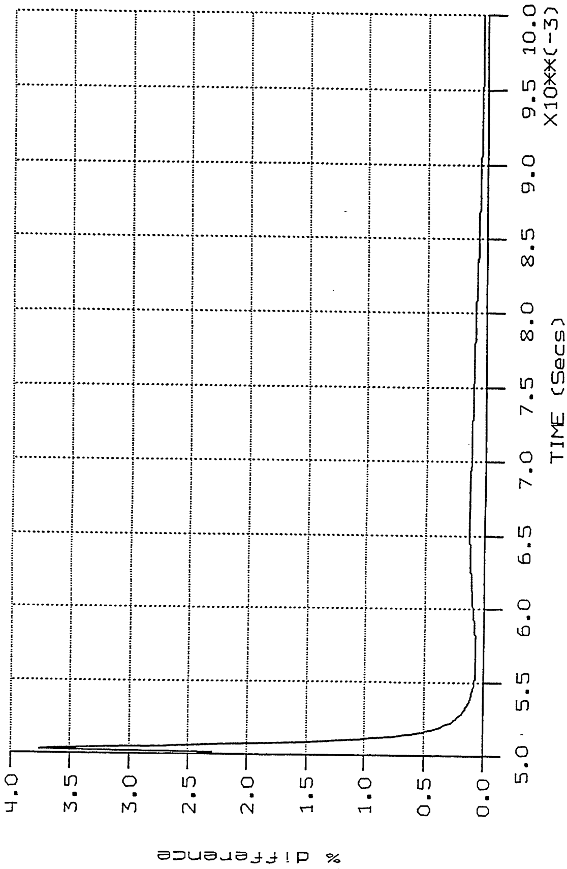
Figure 3.12 -- Percent difference between theoretical and ACQ step change in surface heat-flux
