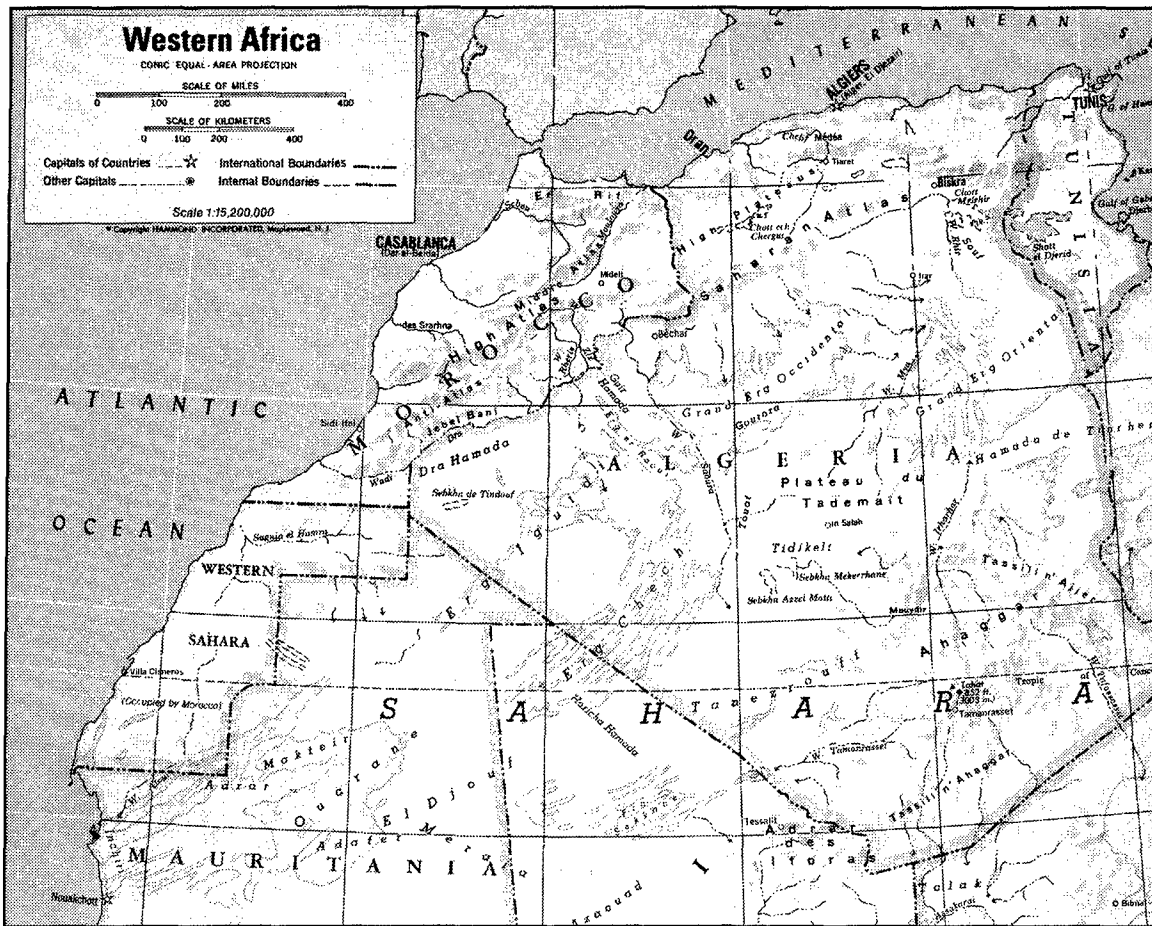
Figure 4-1. Topography of the Sahara.
