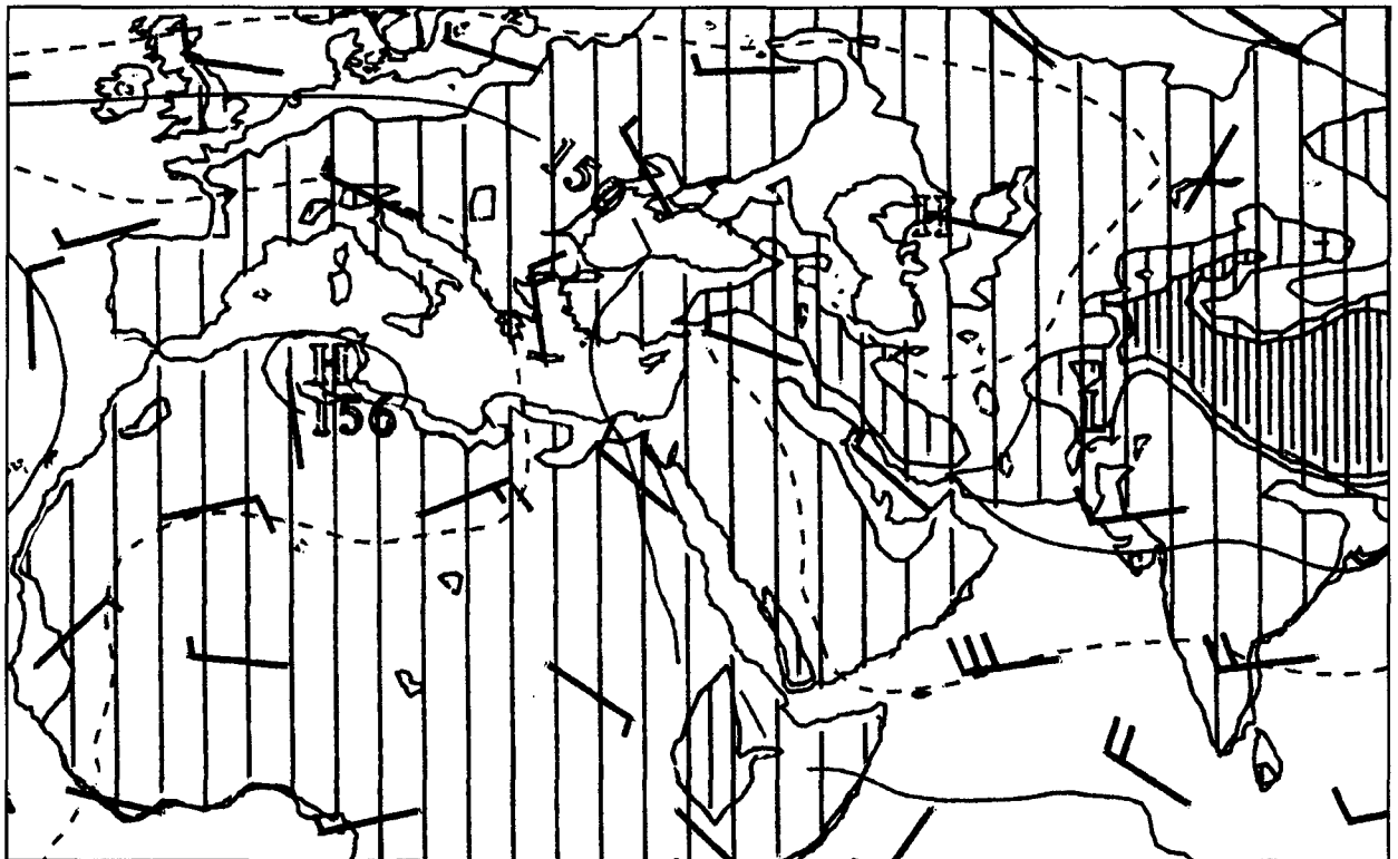
Figure 2-11. Mean January (top) and July (bottom) 850-mb Winds (knots) and Heights (meters). Local points of highest and lowest pressure are designated with H's and L's. Vector mean wind in 5-knot increments are shown. Winds less than 2.5 knots are depicted as a shaft with barbs. Contours of mean geopotential height (solid and dashed lines) in dekameters. Solid lines are labeled, dashed intermediate lines are unlabeled. Solid vertical lines indicate terrain elevations (tighter line spacing denotes higher elevation).
