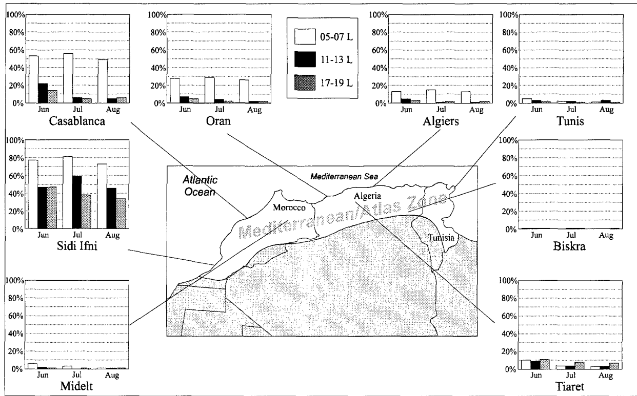
Figure 3-21. Summer Percent Frequencies of Ceilings Below 3,000 Feet (900 meters). The graphs show a monthly breakdown on the percentage of ceilings below 3,000 feet (900 meters) based on location and diurnal influence.
