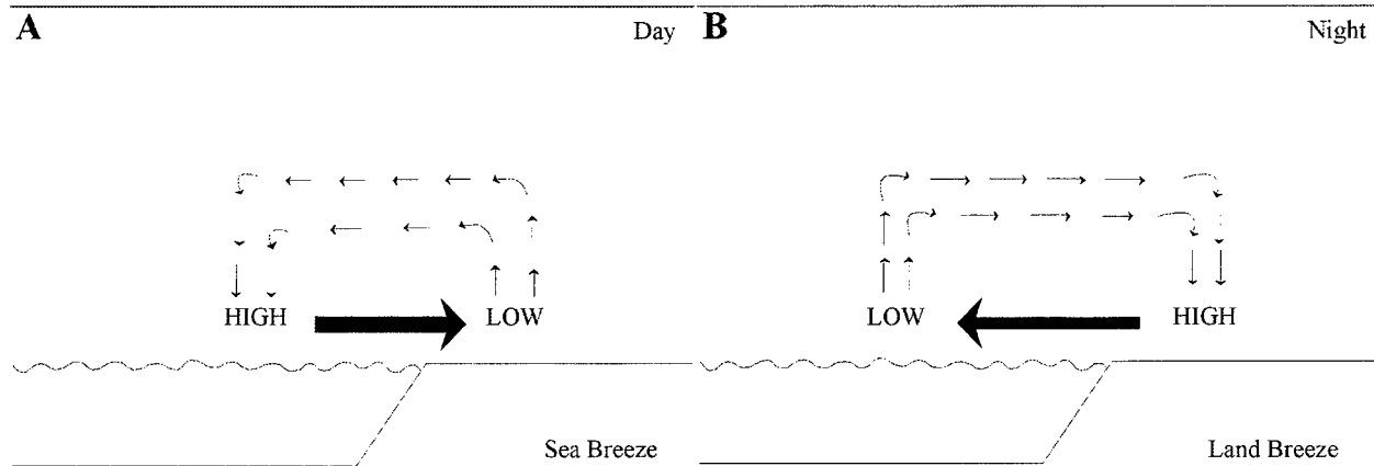
Figure 2-23. The Sea and Land Breezes. Sea (A) and Land (B) flows intensify in proportion to daily heat exchanges between land and water. Thick arrows depict the surface flow.
