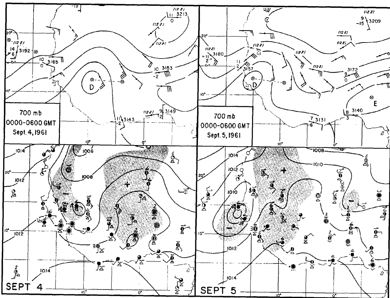
Figure 2-19. African Wave over West Africa Sept. 4-5, 1961, 700-mb and Surface. "X"s and dashed lines show the past 24-hour movement. The shading in the figure represents areas of 24-hour pressure change greater than 2 mb. The D on the 700-mb charts (top) marks the center of the closed low that later became Hurricane Debbie. It reached hurricane strength within 48 hours. The E shows another wave that became Hurricane Esther. The African wave off the coast has a closed low at the surface.
