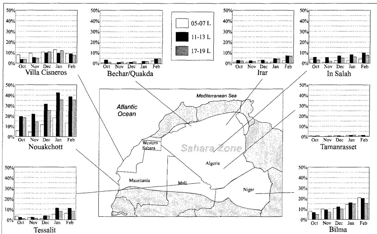
Figure 4-13. Winter Percent Frequencies of Visibilities Below 4,800 Meters. The graphs show a monthly breakdown on the percentage of visibilities below 4,800 meters based on location and diurnal influences.
