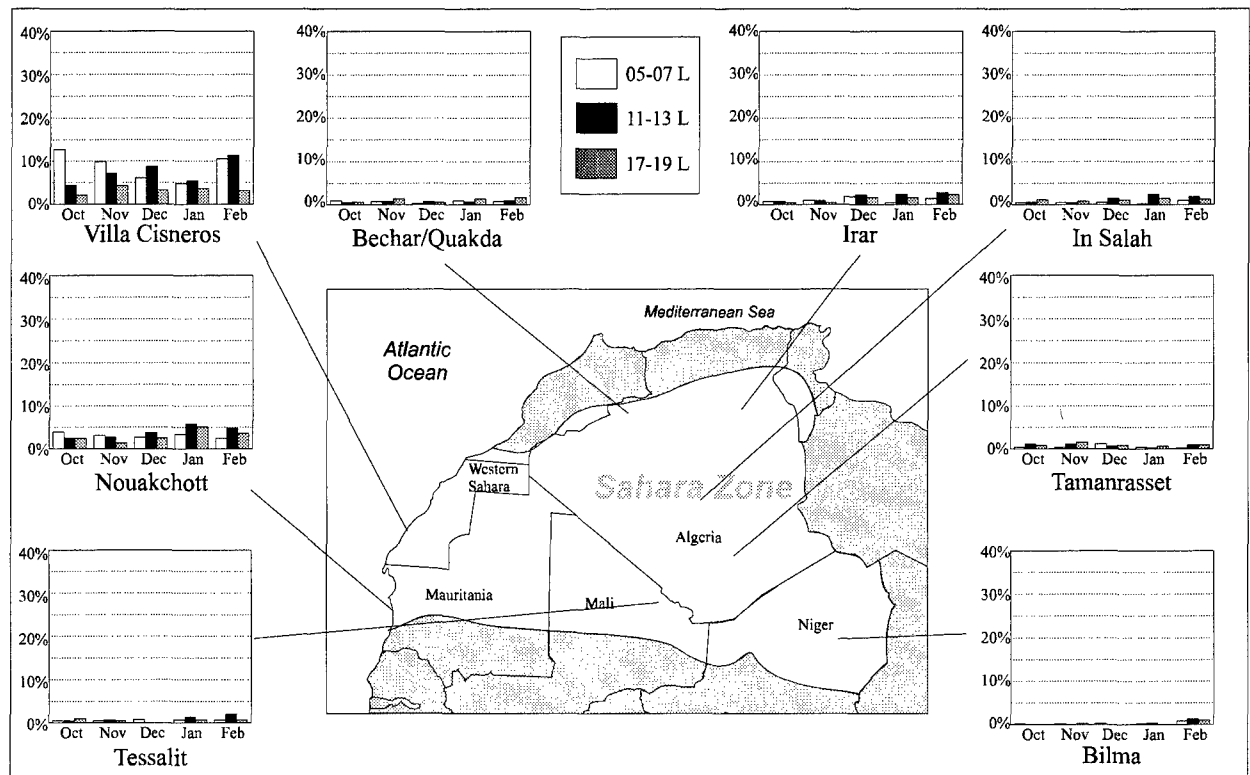
Figure 4-12. Winter Percent Frequencies of Ceilings Below 3,000 Feet (900 Meters). The graphs show a monthly breakdown on the percentage of ceilings below 3,000 feet (900 meters) based on location and diurnal influences.
