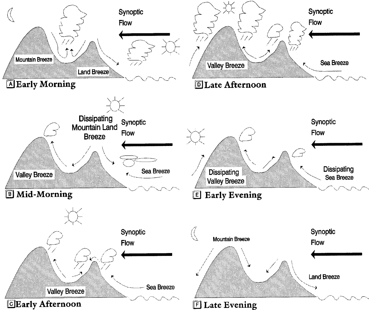
Figure 2-24. Land/Sea Breeze with Onshore Gradient Flow. Onshore gradient flow accelerates orographic lifting by day and produces localized convergence over open water during early morning. By mid- to late afternoon, the sea breeze is well established, and convection moves inland over the ridge tops.
