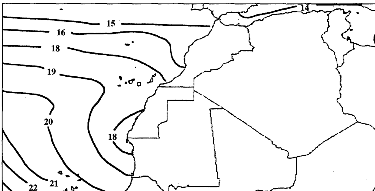
Figure 2-2b. Mean January Sea-Surface Temperatures (° C). The isopleth lines show the difference in Sea-surface temperatures that impact weather conditions along coastal Northwest Africa.
