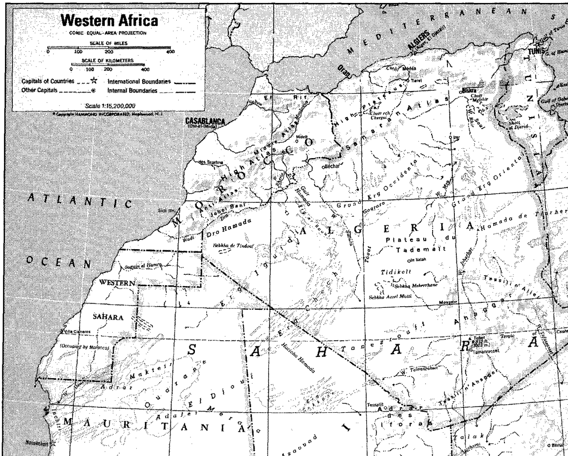
Figure 3-1. Topography of the Mediterranean/Atlas Zone.
