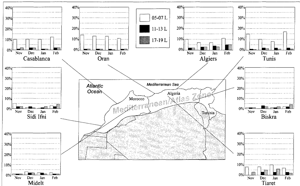
Figure 3-4. Winter Percent Frequencies of Visibilities Below 4,800 Meters. The graphs show a monthly breakdown of the percentage of visibilities below 4,800 meters based on location and diurnal influences.
