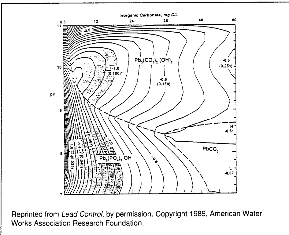
Figure 3. Dissolved inorganic carbonate vs. pH: with phosphates = 0.5 mg PO 4 /L, I = 0.005, T = 25 °C.
