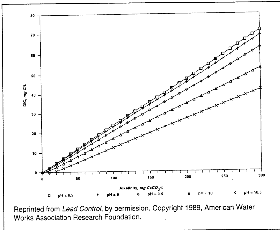
Figure 2f. Relationship between alkalinity and DIC for various pH levels: pH = 8.5-10.5, I = 0.00075, T = 25 °C.
