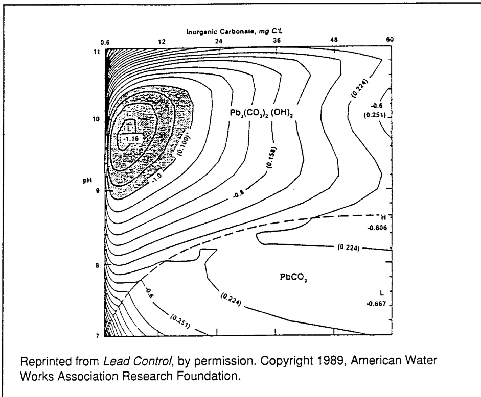
Figure 1. Dissolved inorganic carbonate vs. pH: No phosphite, I = 0.01, T = 25 °C.
