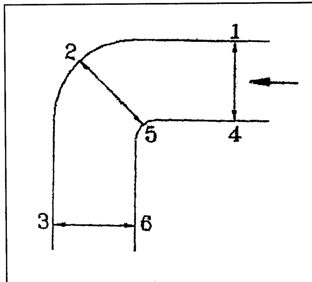
Figure 5. Location of blow-through thickness measurements.
