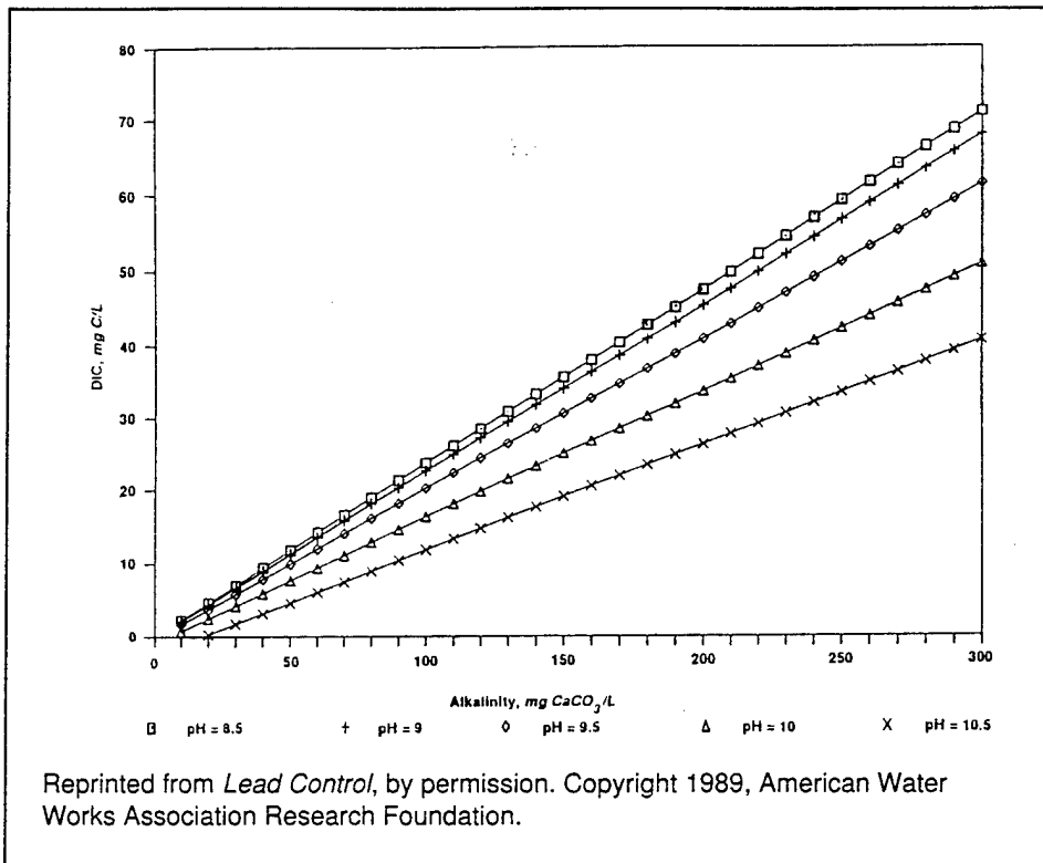
Figure 2d. Relationship between alkalinity and DIC for various pH levels: pH = 8.5-10.5, I = 0.005, T = 25 °C.
