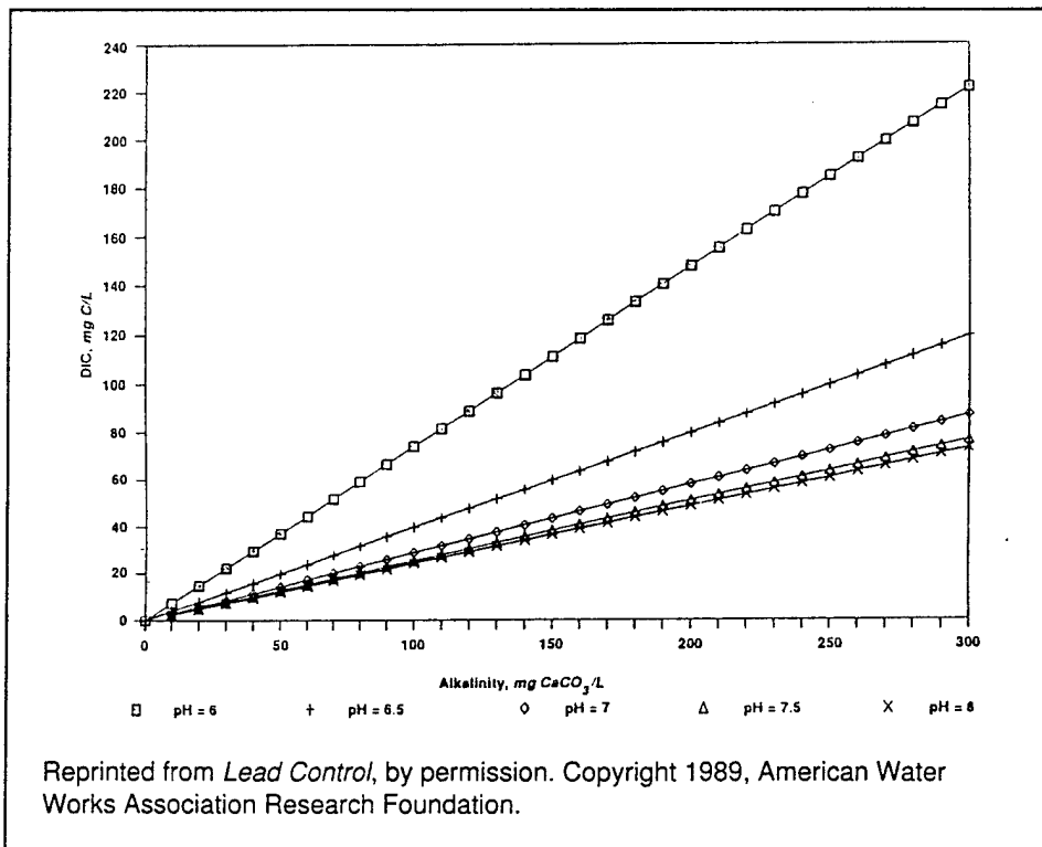
Figure 2e. Relationship between alkalinity and DIC for various pH levels: pH = 6-8, I = 0.00075, T = 25 °C.
