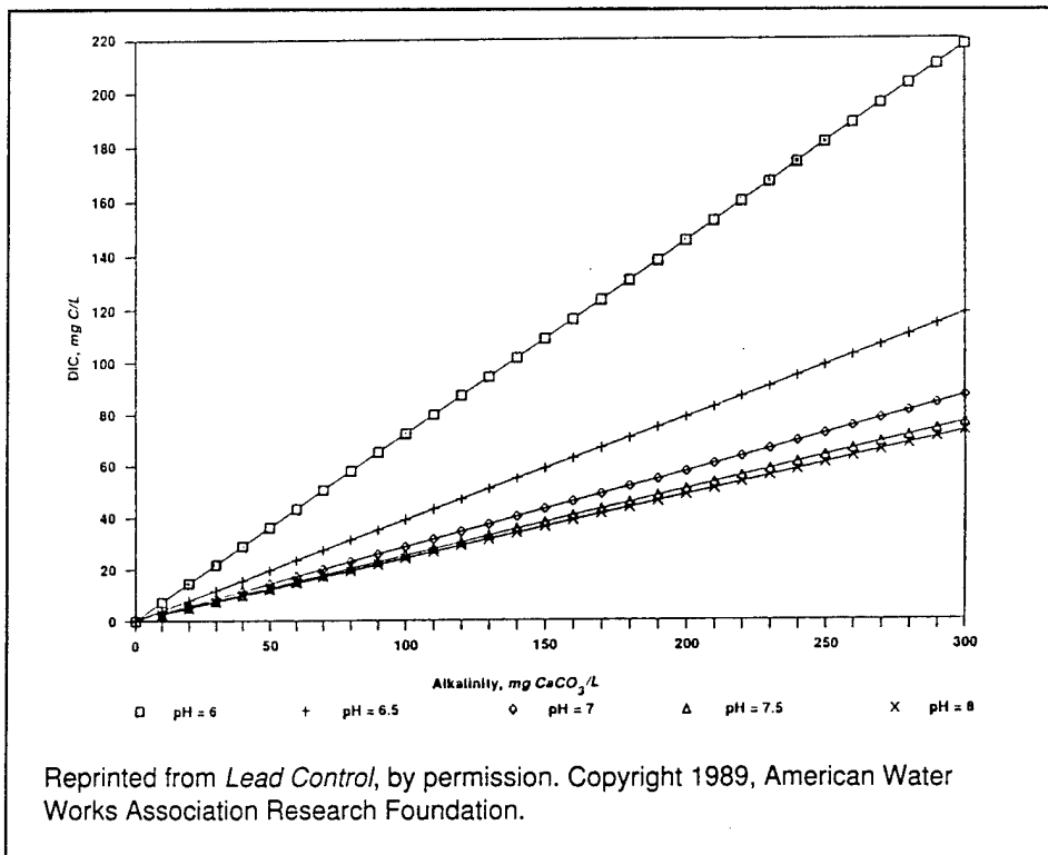
Figure 2a. Relationship between alkalinity and DIC for various pH levels: pH = 6-8, I = 0.01, T = 25 °C.
