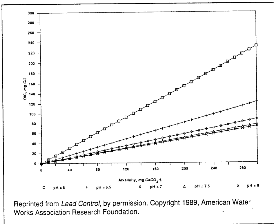
Figure 2g. Relationship between alkalinity and DIC for various pH levels: pH = 6-8, I = 0.00025, T = 25 °C.
