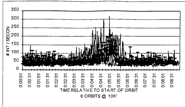
FIGURE 35. UNSUPRESSED MODE 2 INTERROGATIONS
