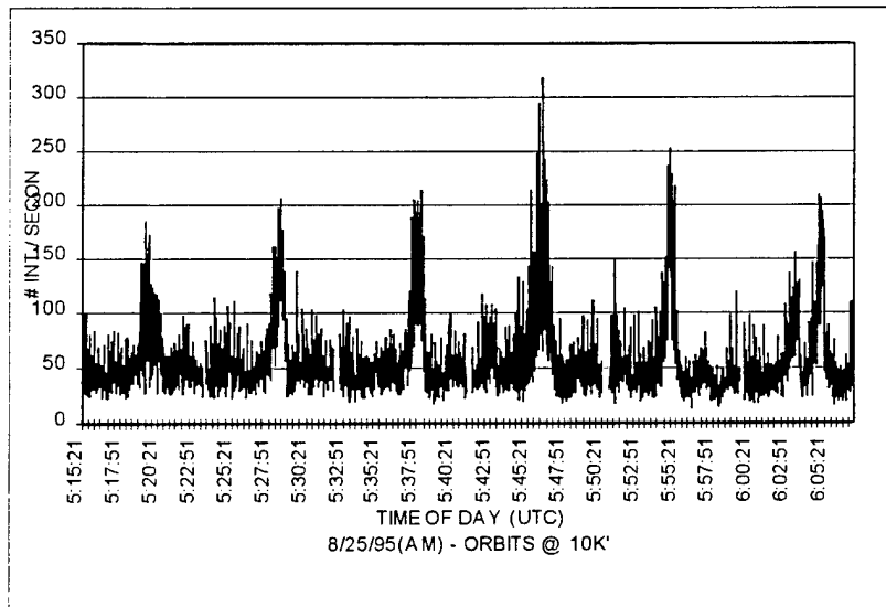
FIGURE 34. UNSUPPRESSED MODE 2 INTERROGATIONS
