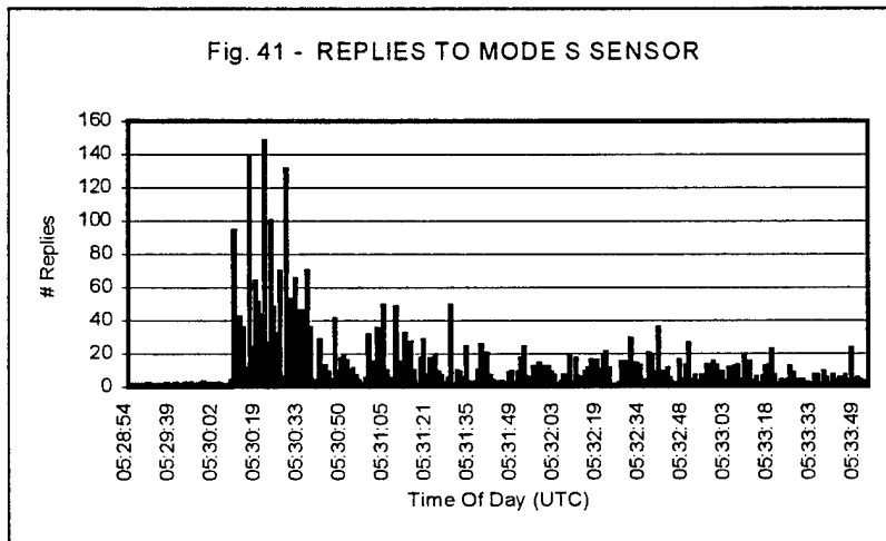
FIGURE 41. REPLIES TO MODE S SENSOR
