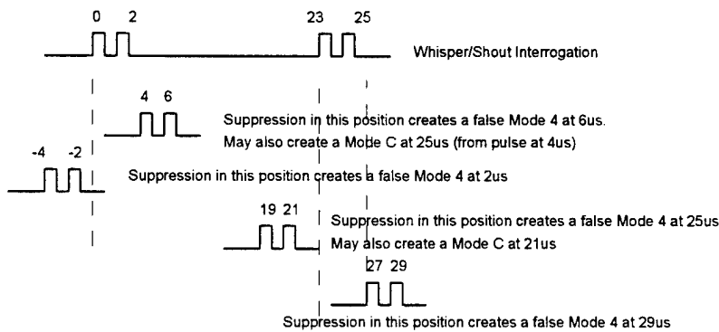
FIGURE 5. CREATION OF FALSE MODE 4 BY COMBINING WITH SUPPRESSION
