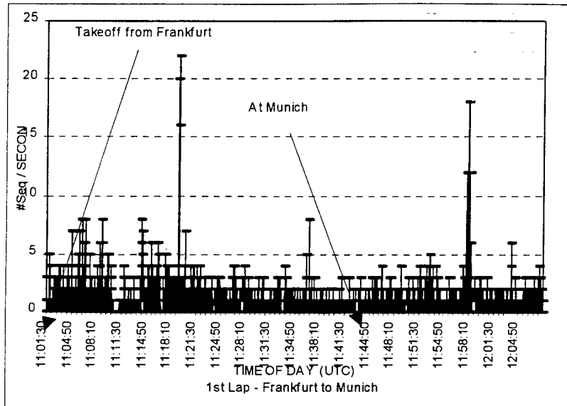
FIGURE 8. MODE 4 INTERROGATIONS
