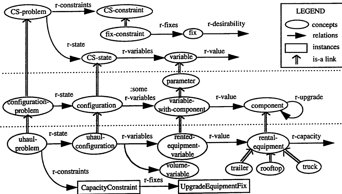
Figure 1: EXPECT's representation of some of the factual knowledge needed for propose-and-revise problems, for configuration problems, and for the U-Haul domain. Notice that the relations across these subdomains are naturally captured in the subsumption hierarchy.
