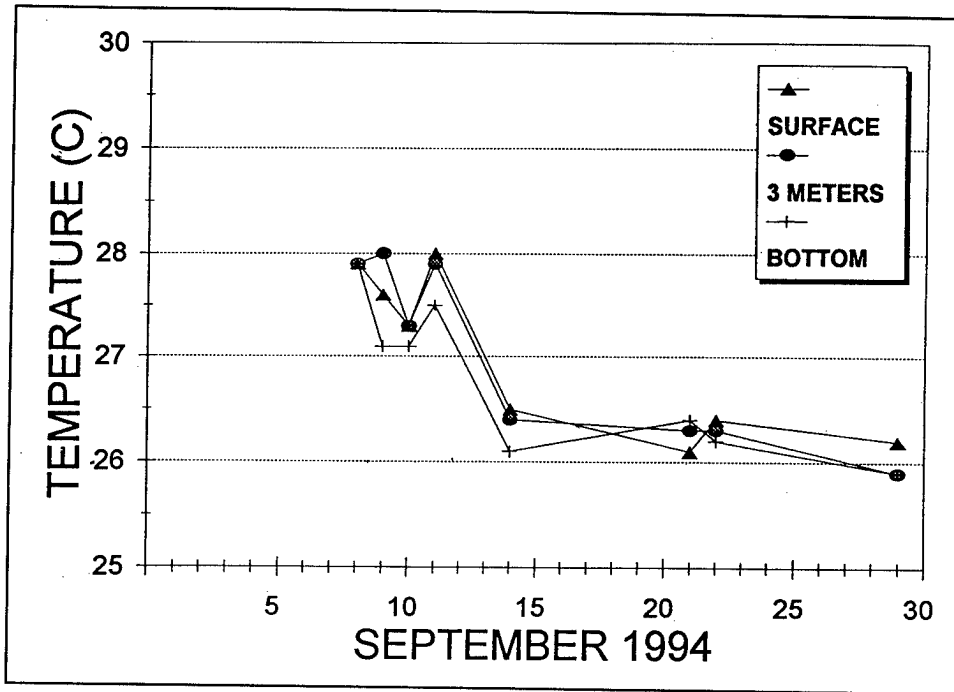
Figure 9. Surface, mid-water, and bottom temperature profiles, Canaveral, Florida, September 1994
