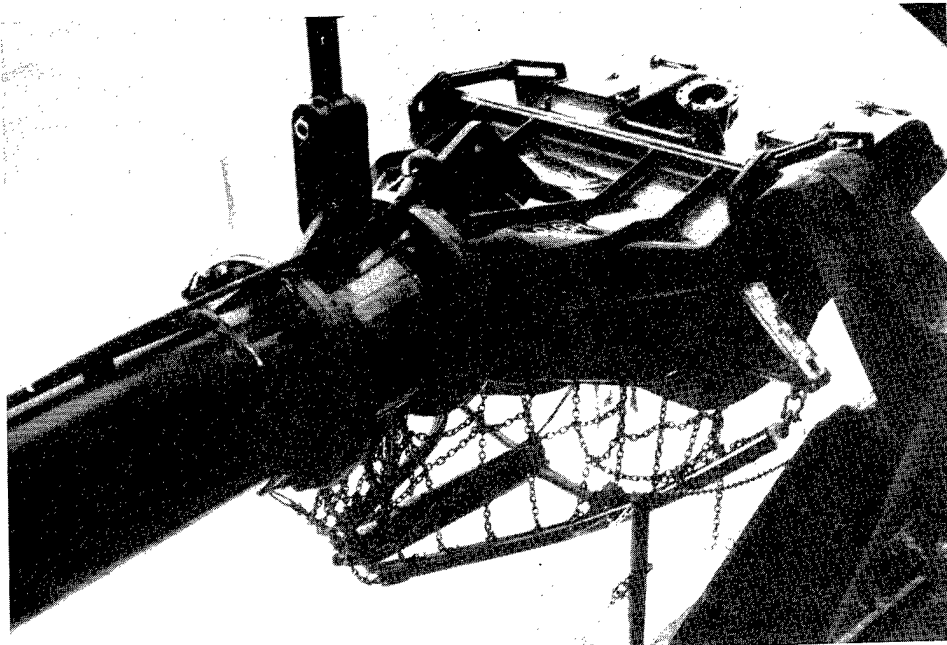
Figure 1. California draghead with flexible chain deflector
