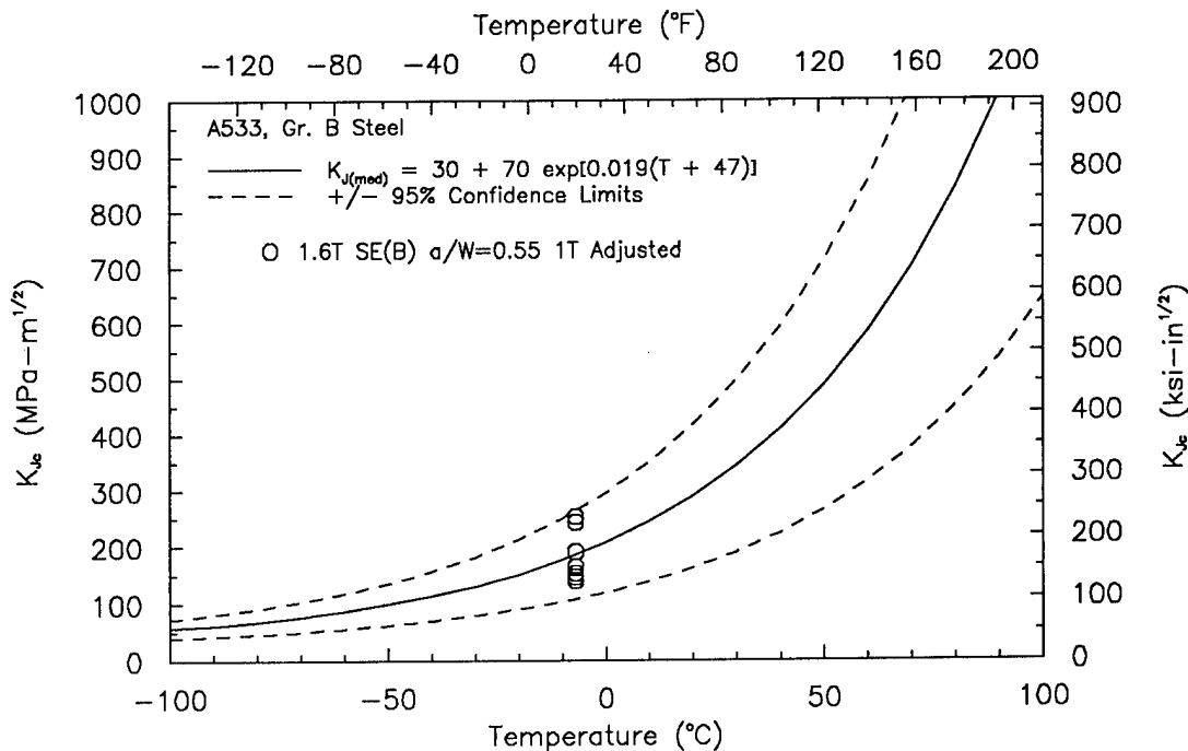
Figure 8 Master curve obtained from 1.6T SE(B) specimens tested at -7^{\circ}\text{C} .
