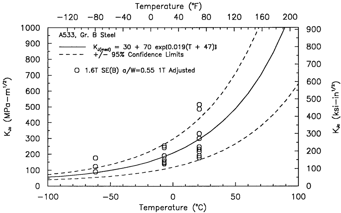
Figure 9 Comparison of the fracture toughness measured at -62^{\circ}\text{C} and 21^{\circ}\text{C} with the master curve and confidence limits for the deeply notched 1.6T SE(B) specimens.
