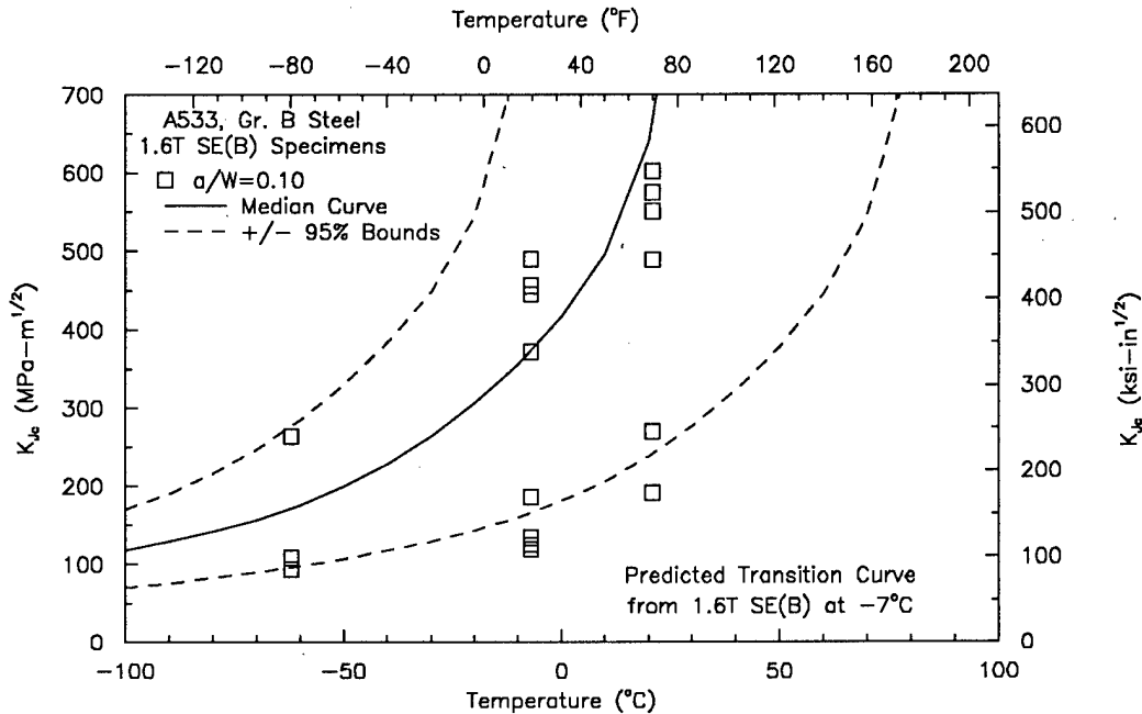
Figure 17 Comparison of the predicted median and confidence limits with the measured cleavage fracture toughness for 1.6T SE(B) specimens with a/W=0.1 .
