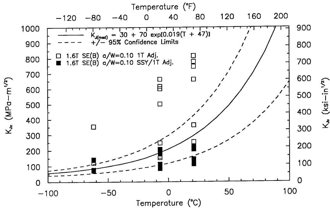
Figure 11 As-measured and constraint-corrected fracture toughness results for shallow cracked 1.6T SE(B) specimens.
