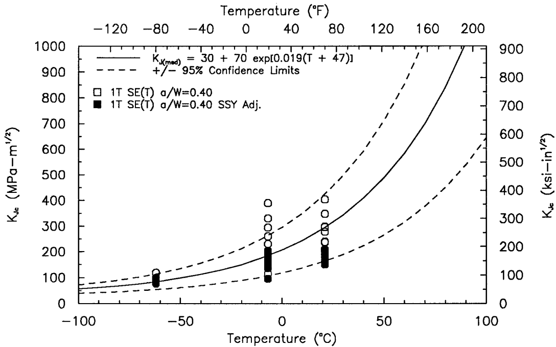
Figure 12 As-measured and constraint-corrected fracture toughness results for 1T SE(T) specimens, a/W=0.4 compared with master curve from 1.6T SE(B) specimens.
