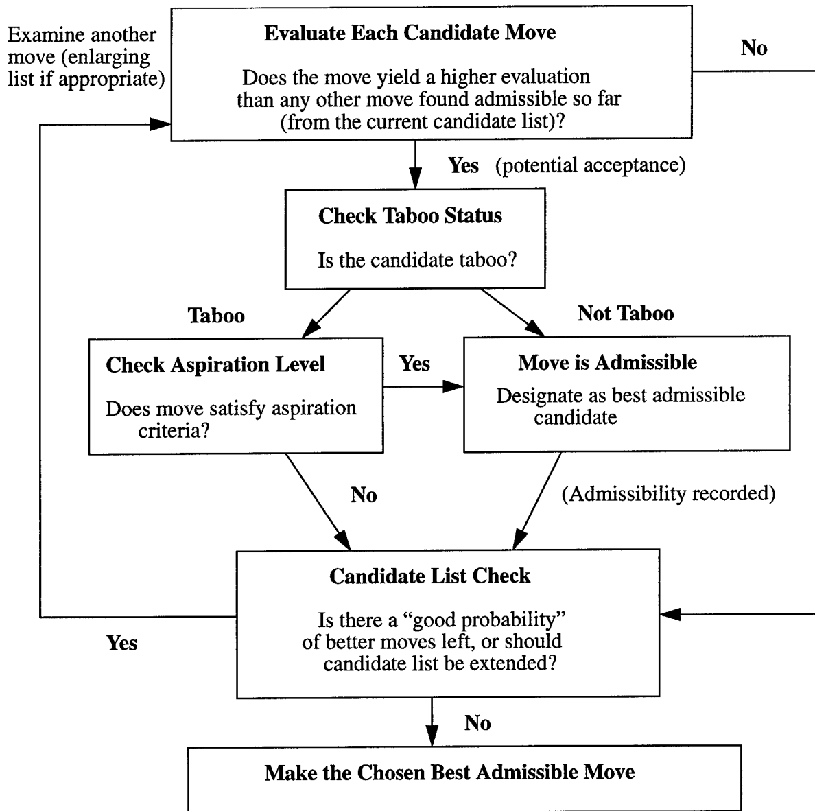
Figure 9. Flow chart from Glover that describes how the tabu search defines the selection process for the next move.
