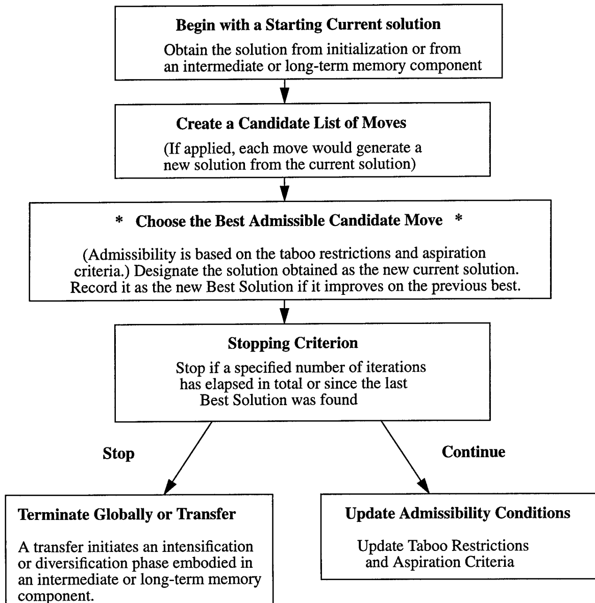
Figure 8. Flow chart from Glover that logically organizes the decisions made during the taboo search process.
