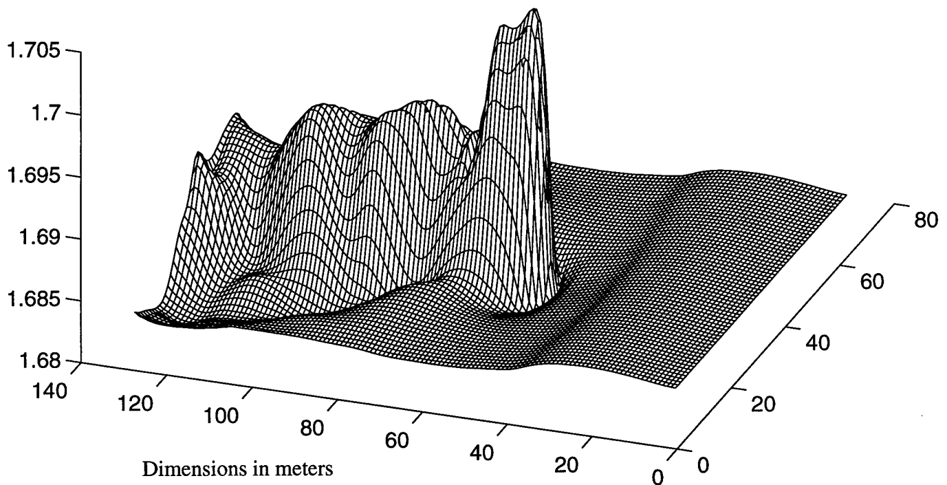
Figure 14. The above contour uses temperature ( ^{\circ}\text{C} ) as the vertical axis. The data was taken from a horizontal slice of a three dimensional model of temperatures in a fully developed hydrothermal plume in the presence of cross flow and rotational vorticity developed by Lavelle and supplied to the author. Note the presence of multiple local peaks distinct from the global peak in the wake of the plume source and the fact that the entire grid spans only 0.025^{\circ}\text{C} . This slice is taken from a 13MW discrete source in the presence of a 1.5 cm/s cross flow 150m above the vent.
