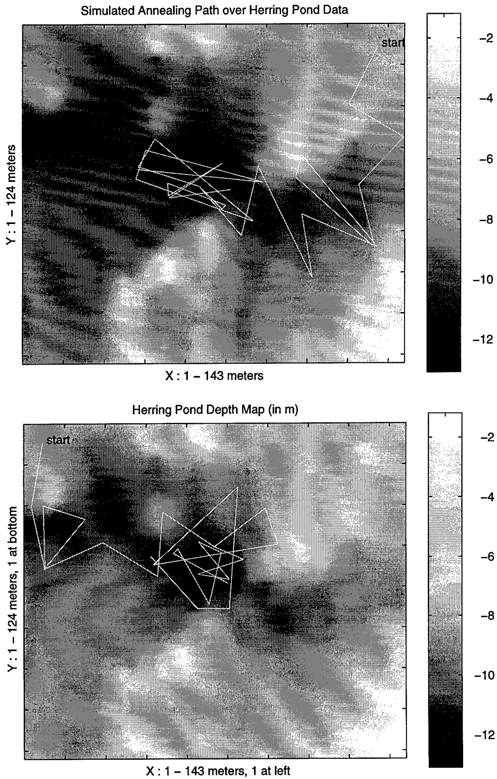
Figure 7. These plots show the path of a simulated annealing routine over the Herring Pond data set. Motion is purely geometric and true to the algorithm without consideration for the vehicle dynamics. Yet, in both cases, it is successful in reaching the global deep spot in the middle of the pond.
