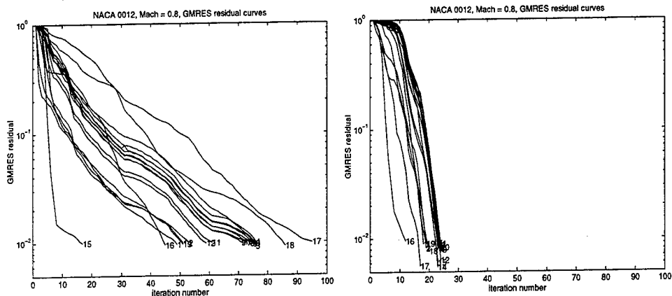
Figure 7: The GMRES convergence history for the entire nonlinear iteration. The left figure does not have a coarse space in the Schwarz preconditioner, the right figure contains a 7 \times 8 coarse space. The number at the tail of each curve corresponds to the Newton iteration number.
