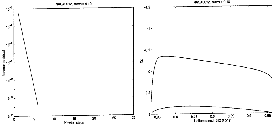
Figure 4: For M_\infty = 0.1 , the left figure shows the history of the Newton residual, and the right shows the (upper surface) C_p curve at convergence.
