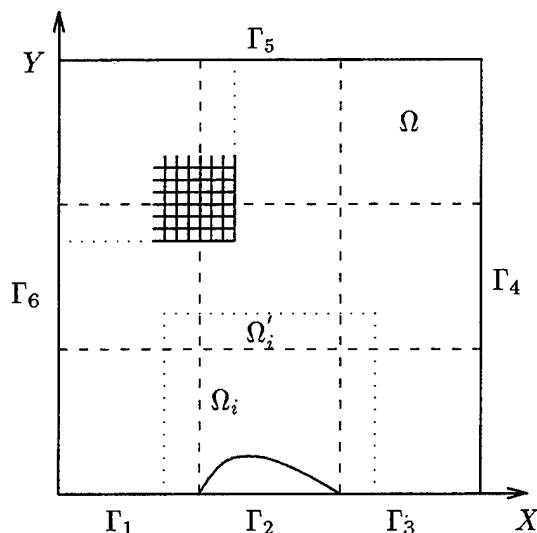
Figure 3: Domain \Omega with an exaggerated NACA 0012 curve at the bottom. The dashed lines indicate the partition of the domain into nonoverlapping substructures, and the dotted lines indicate the overlapping subdomains. The incomplete fine mesh of solid lines illustrates an overlap of 3 subintervals. \Gamma_6 is the inflow, \Gamma_5 the freestream, and \Gamma_4 the outflow boundary.
