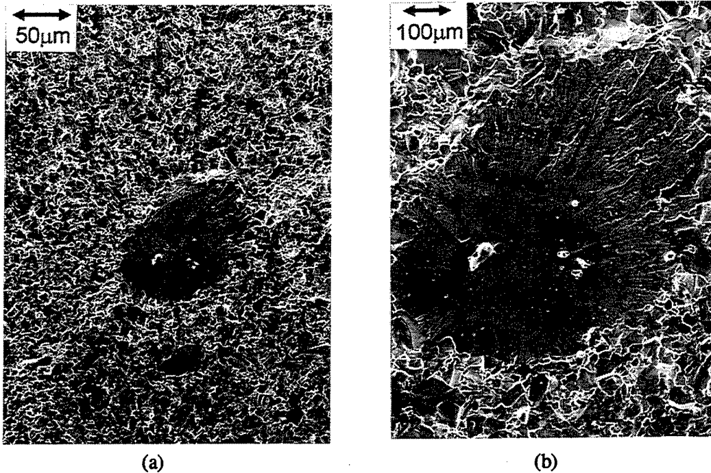
Figure 3. Fracture origin of TiB_2 specimen shows (a) a large grain at the center of the "pseudo mirror" and (b) a small particle within the large grain.
